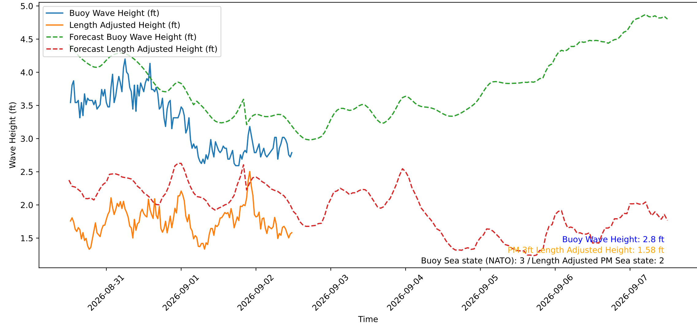
Wave Heights over Time for Red Beach at 2026-09-02 12:10:49
