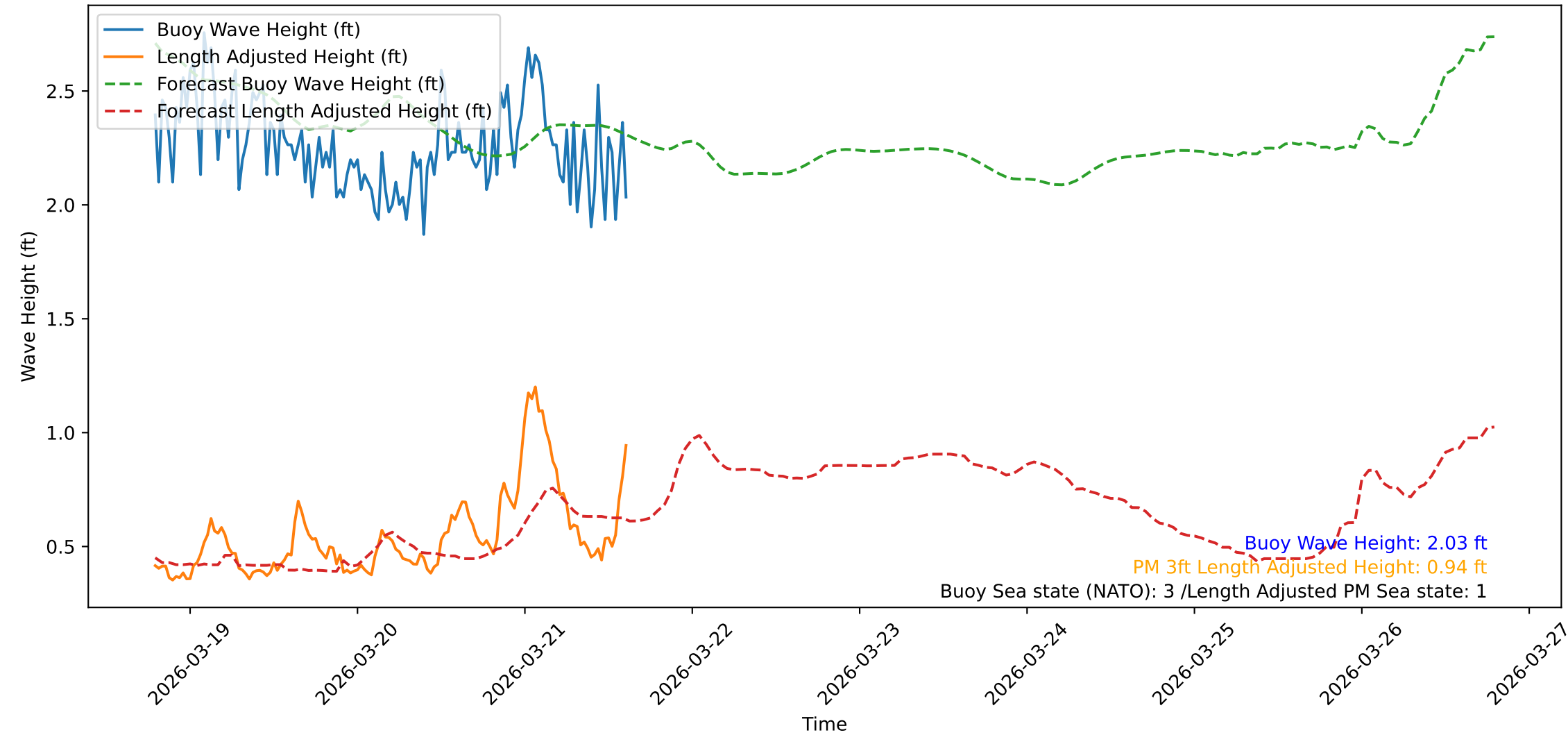
Wave Heights over Time for Red Beach at 2026-03-21 18:40:47
