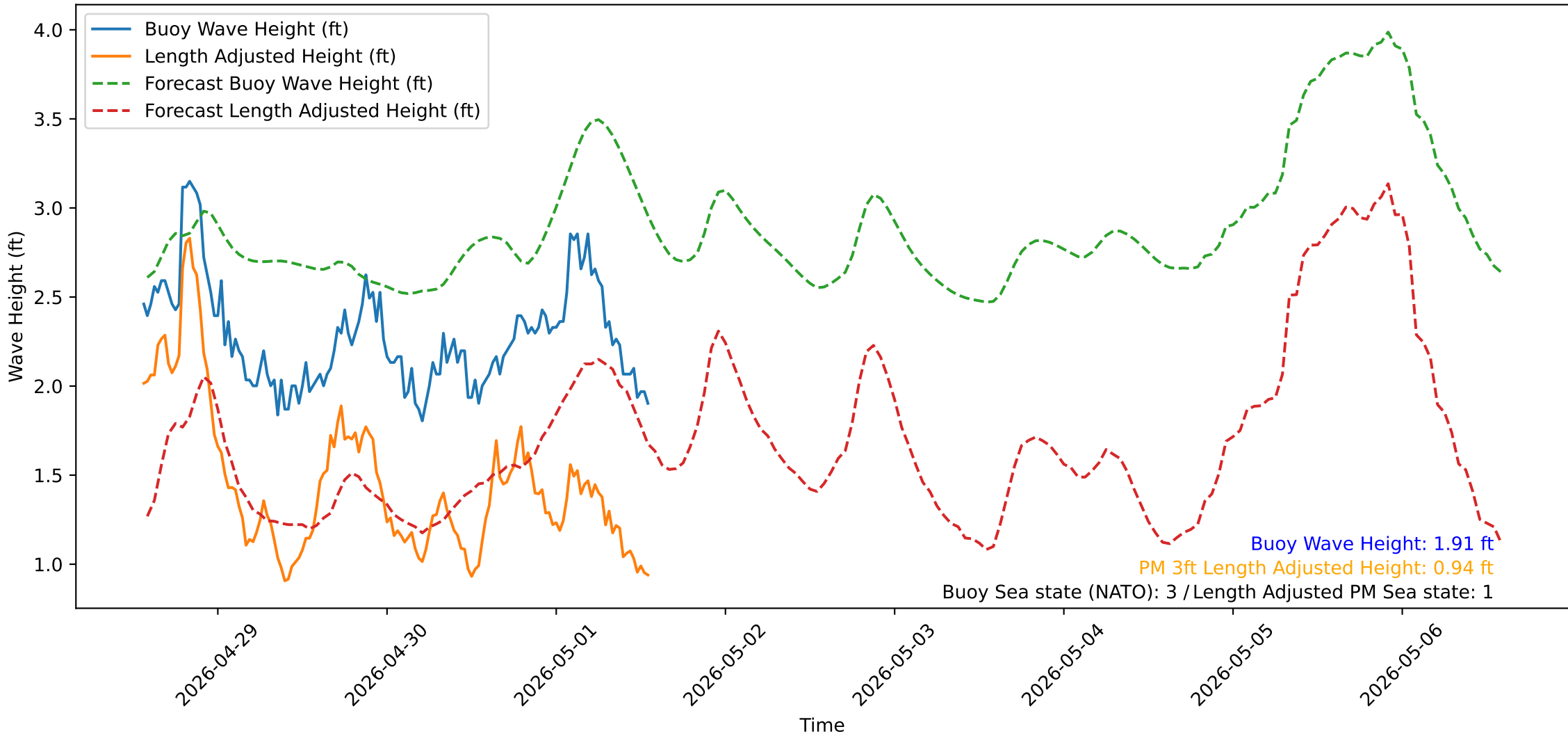
Wave Heights over Time for Green Beach at 2026-05-01 13:41:13
