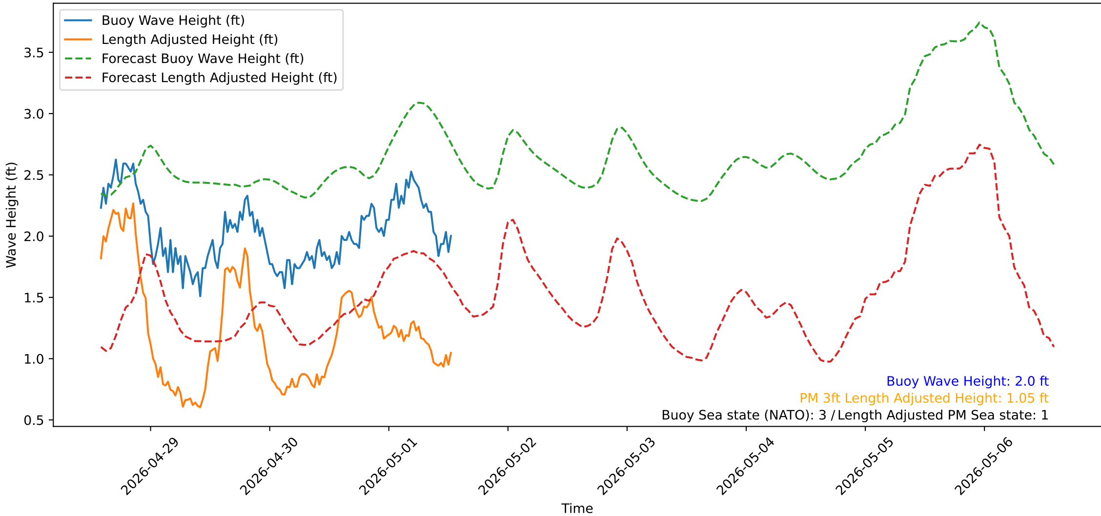
Wave Heights over Time for Red Beach at 2026-05-01 13:40:51
