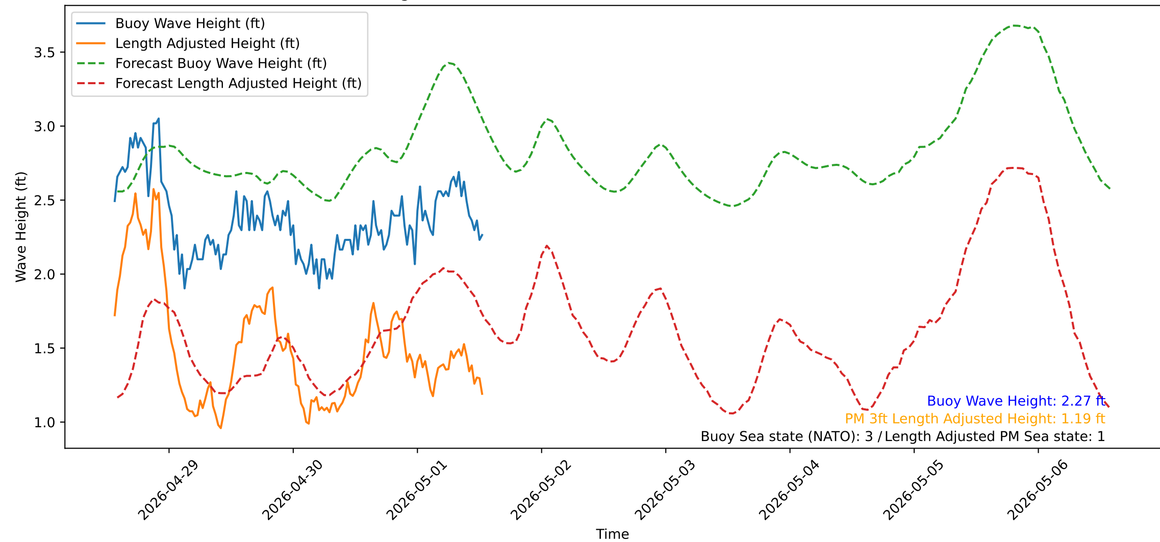
Wave Heights over Time for Oceanside Harbor at 2026-05-01 13:40:31
