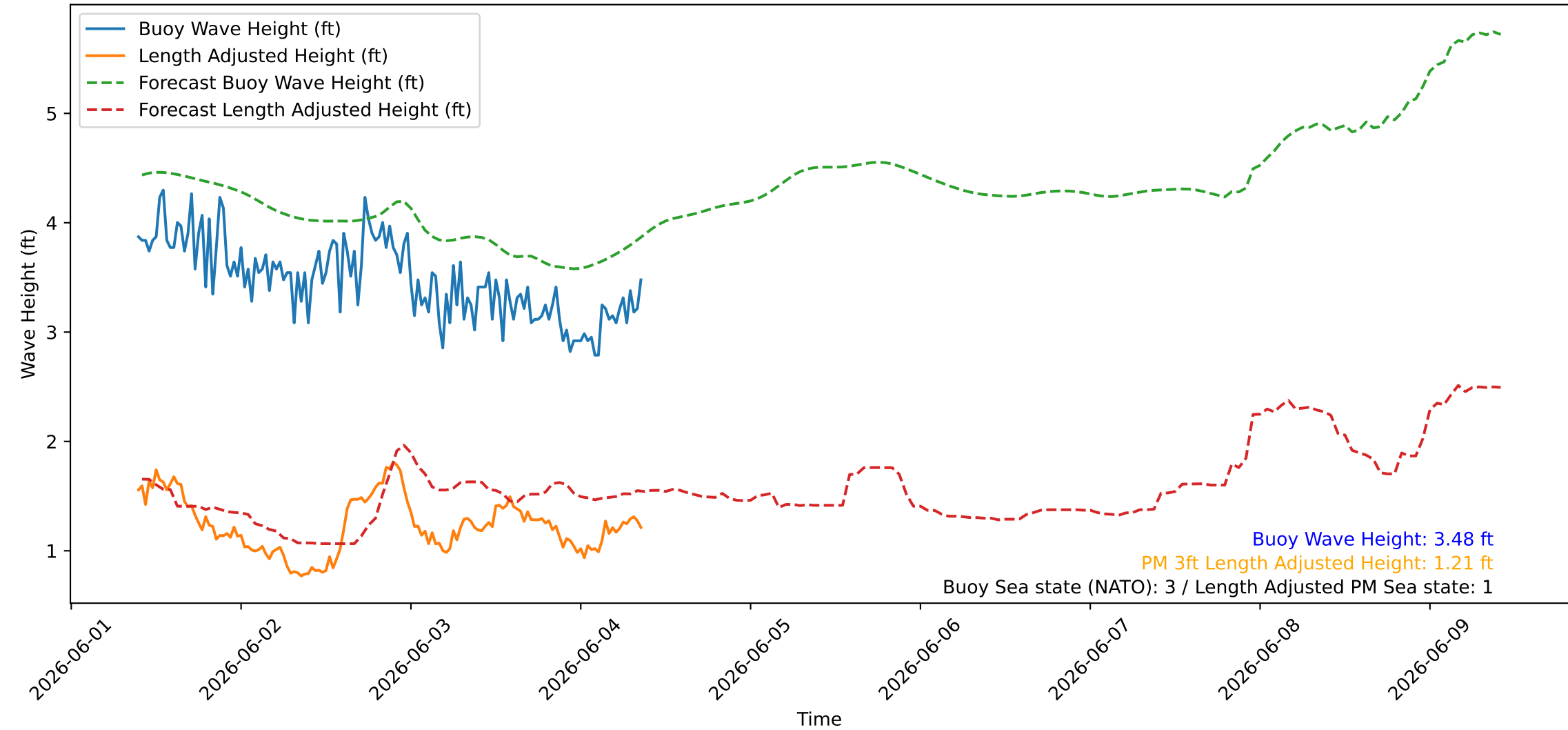
Wave Heights over Time for Green Beach at 2026-06-04 09:31:08
