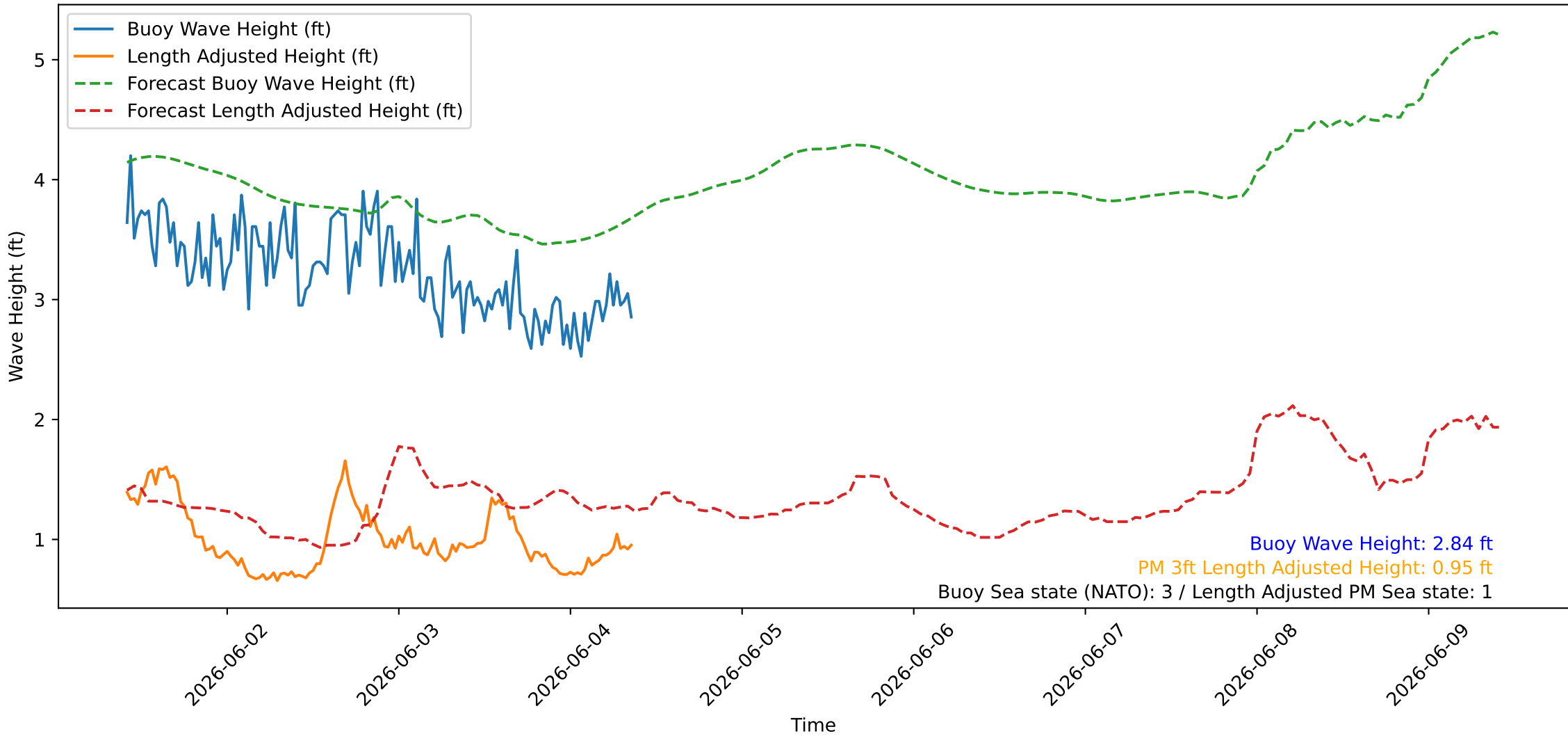
Wave Heights over Time for Red Beach at 2026-06-04 09:30:45
