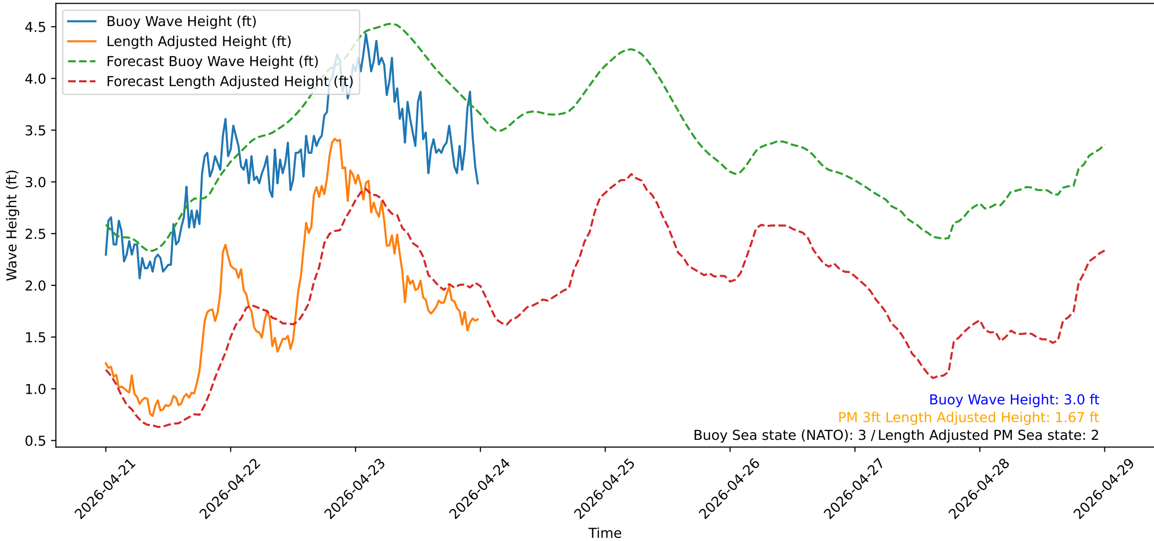
Wave Heights over Time for Oceanside Harbor at 2026-04-24 00:00:31
