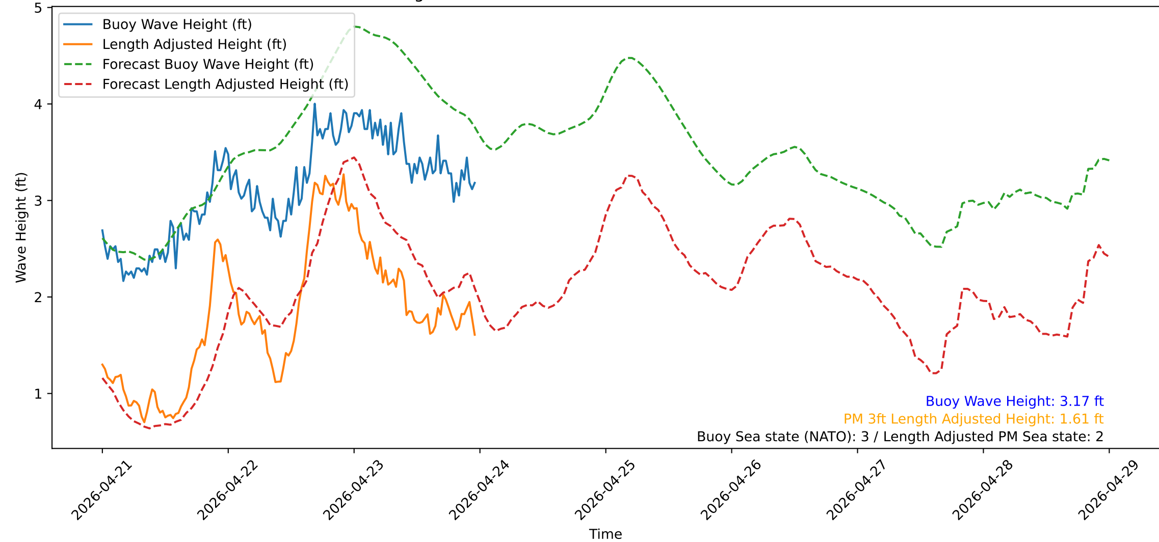
Wave Heights over Time for Green Beach at 2026-04-24 00:01:13
