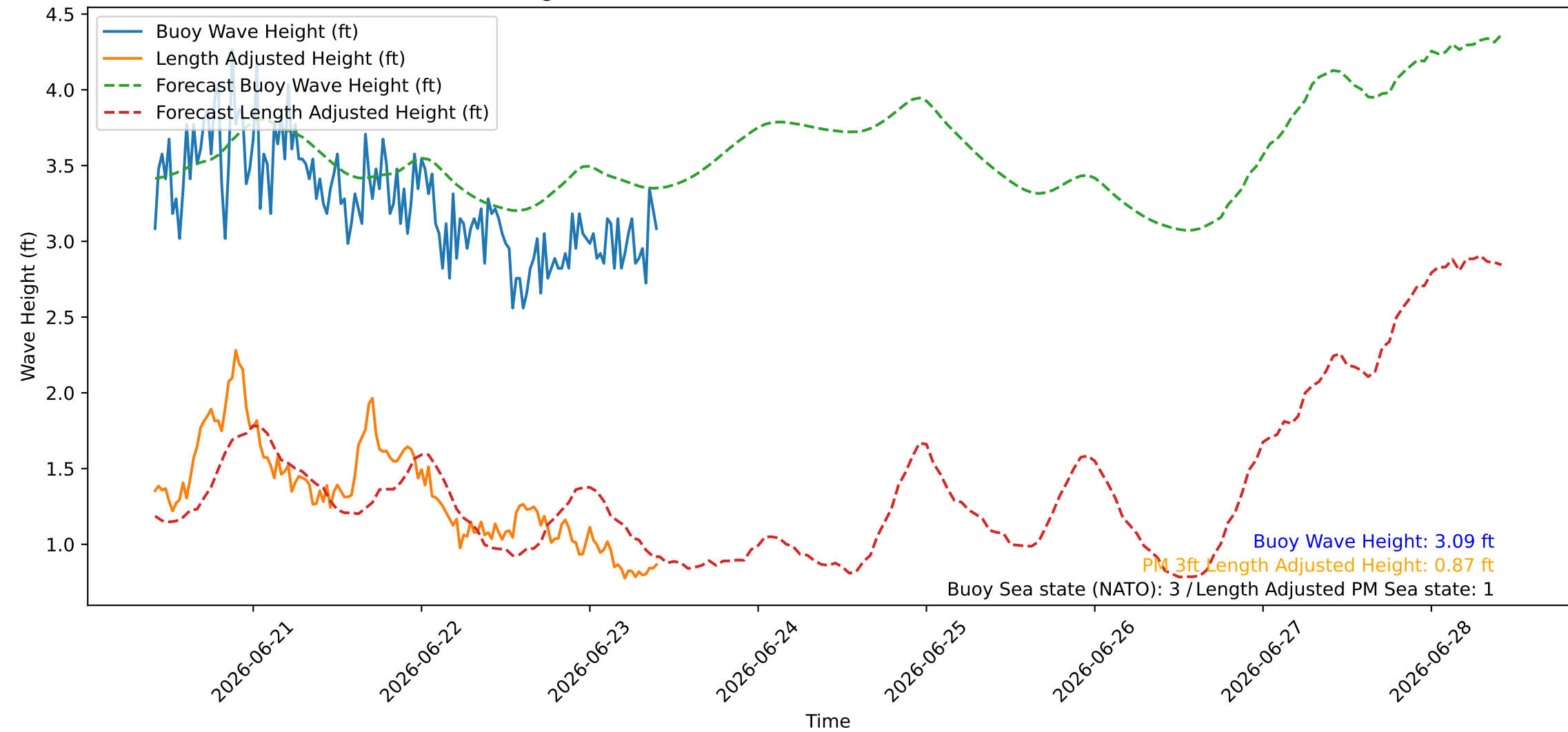
Wave Heights over Time for Oceanside Harbor at 2026-06-23 10:10:26
