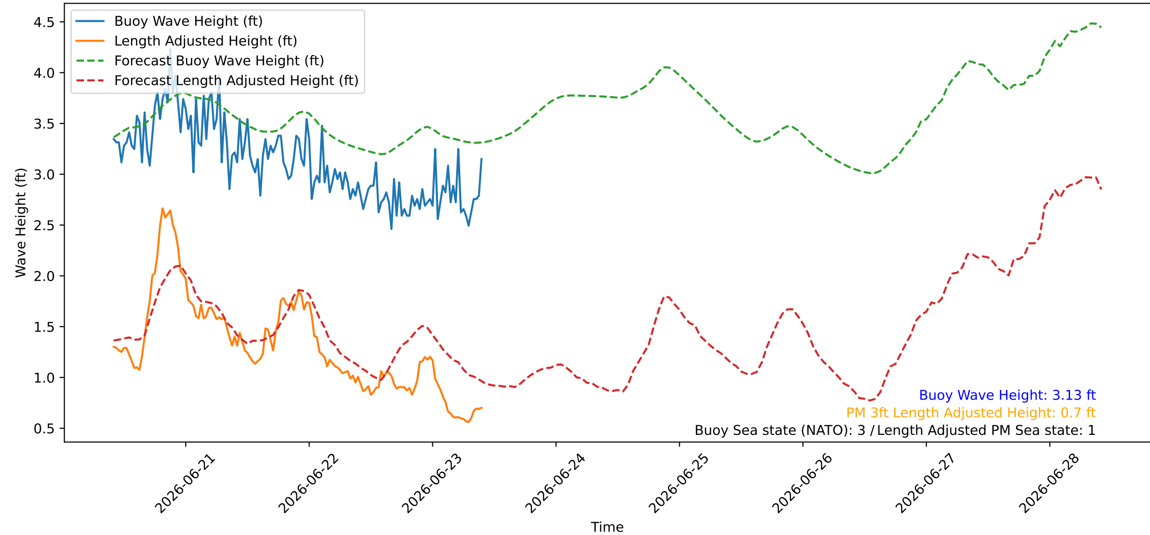
Wave Heights over Time for Green Beach at 2026-06-23 10:11:08
