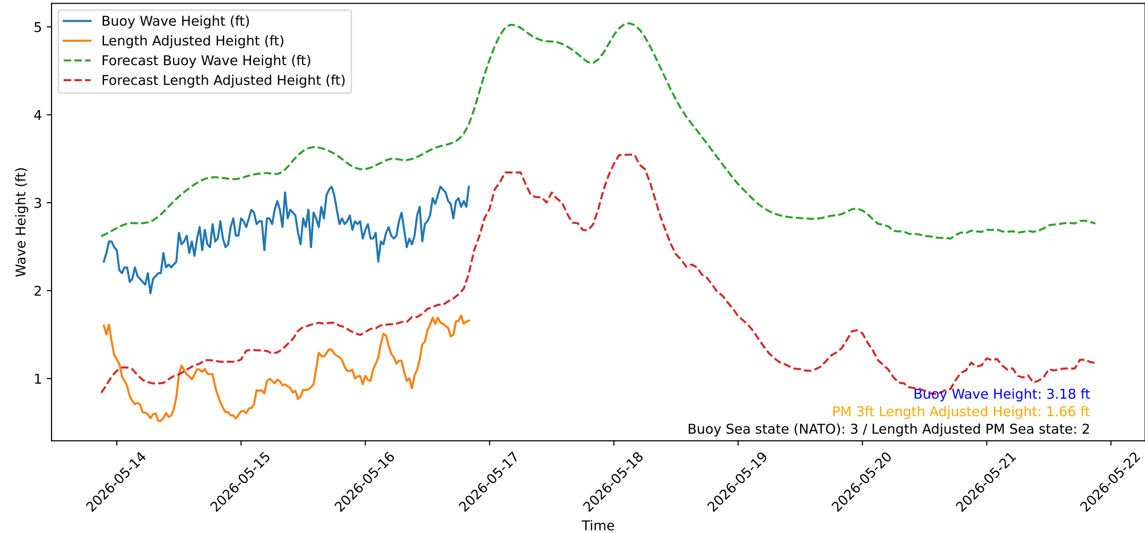
Wave Heights over Time for Red Beach at 2026-05-16 21:10:51
