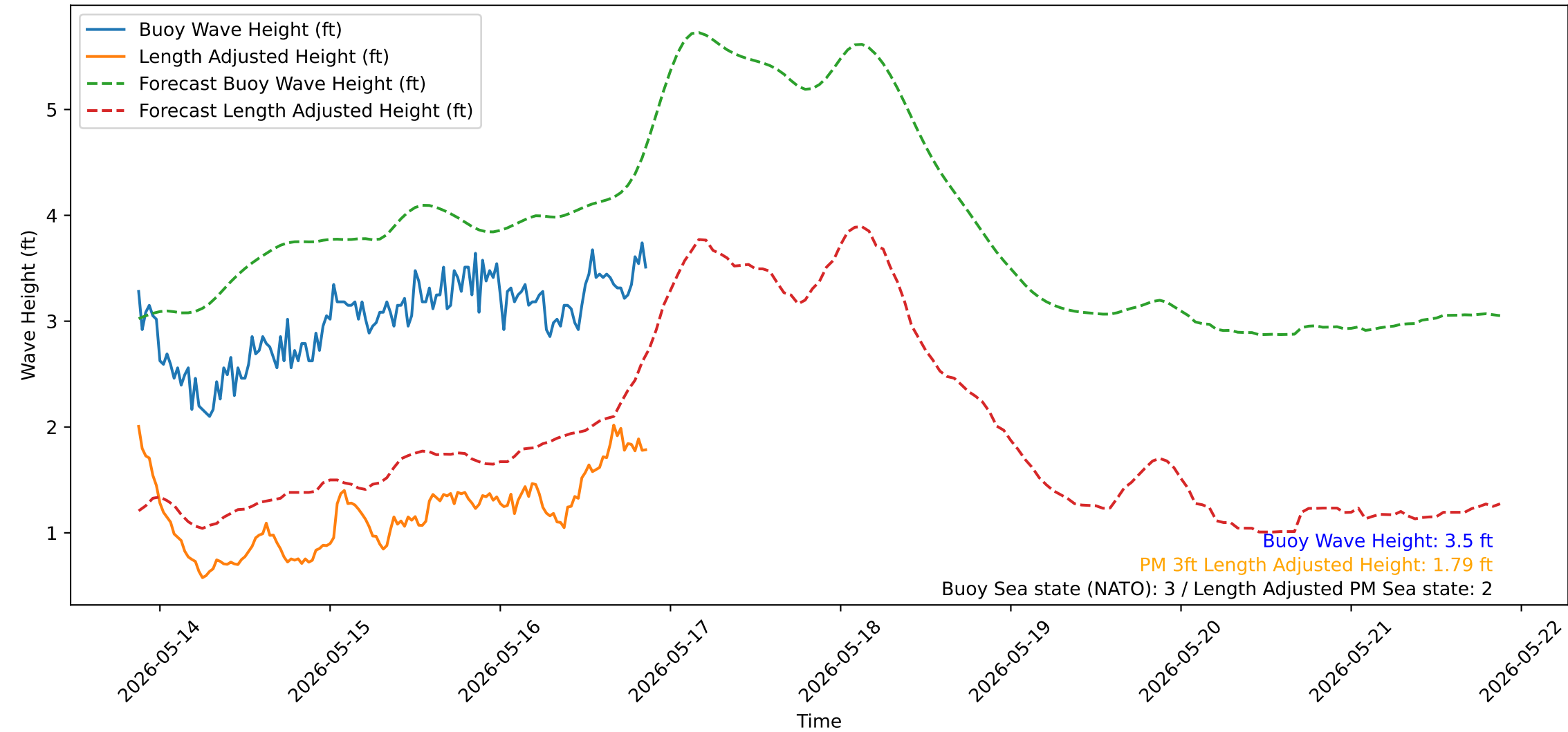
Wave Heights over Time for Green Beach at 2026-05-16 21:11:14
