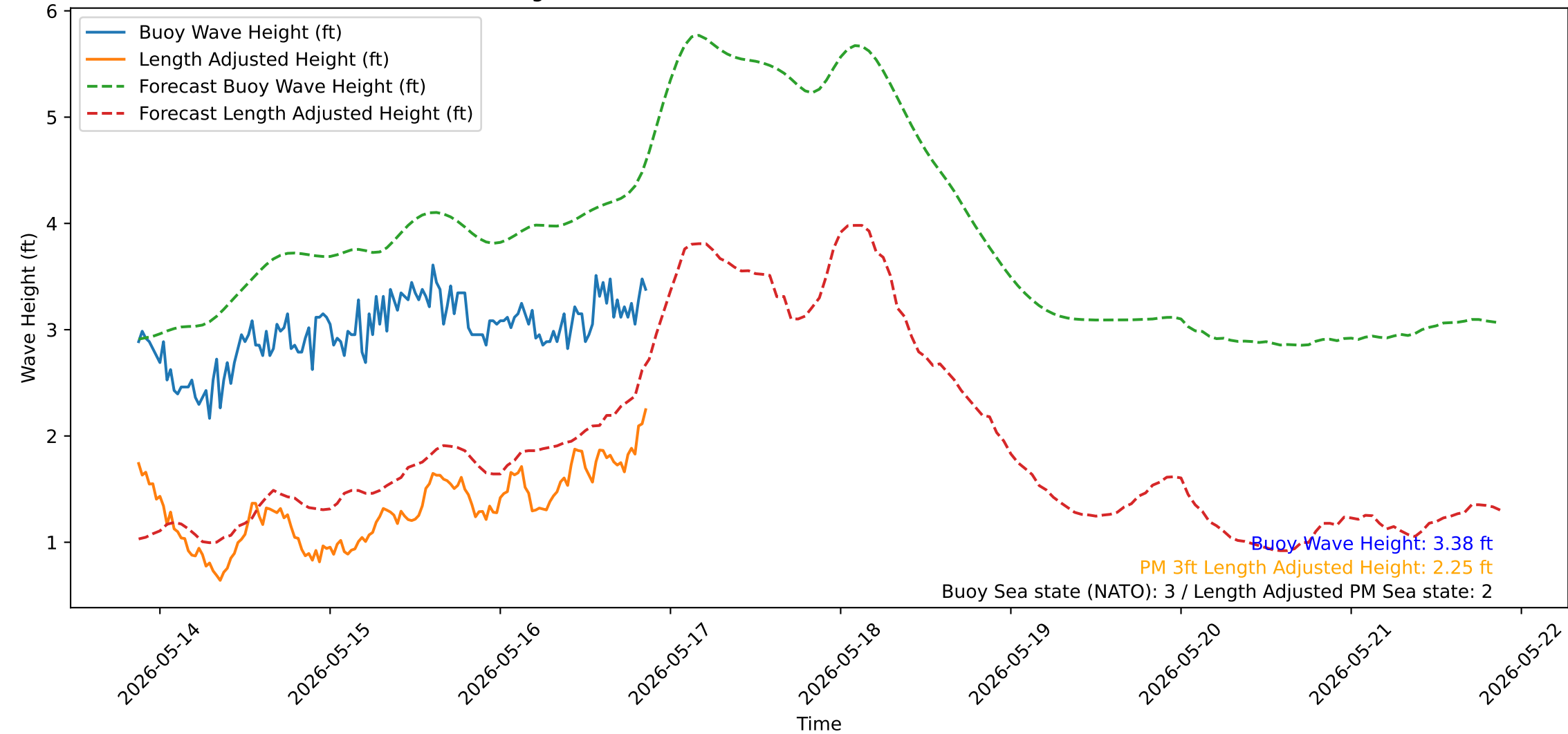
Wave Heights over Time for Oceanside Harbor at 2026-05-16 21:10:31
