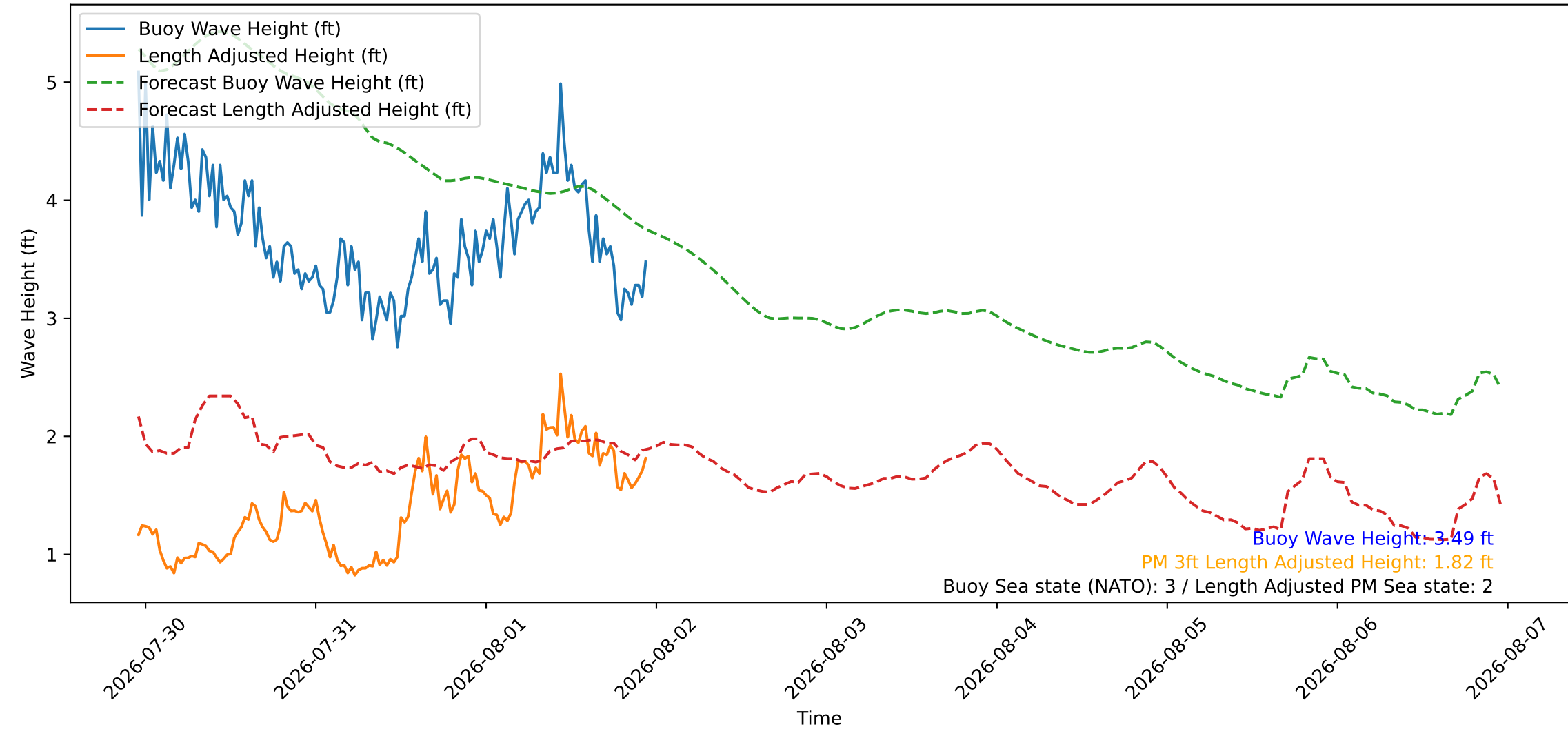
Wave Heights over Time for Green Beach at 2026-08-01 23:11:08
