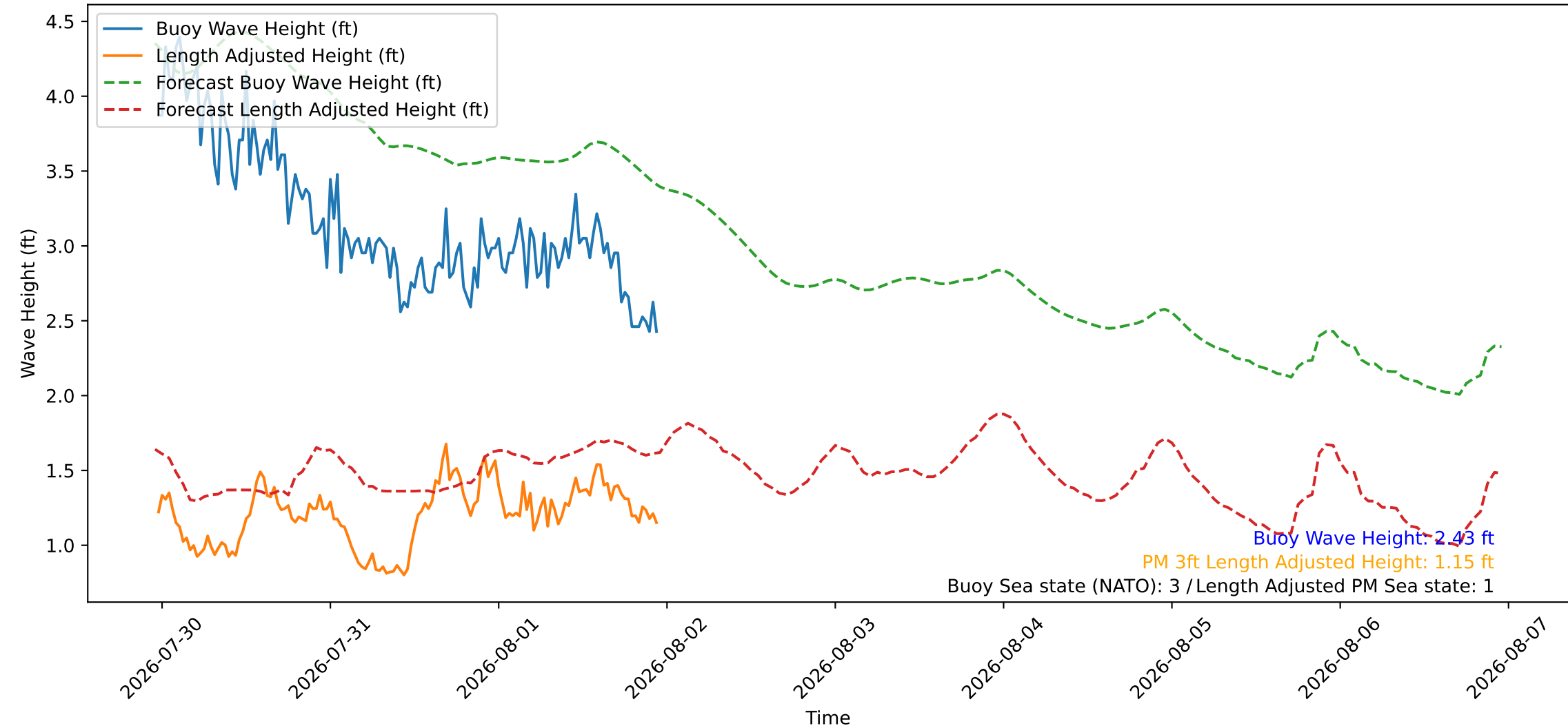
Wave Heights over Time for Red Beach at 2026-08-01 23:10:45
