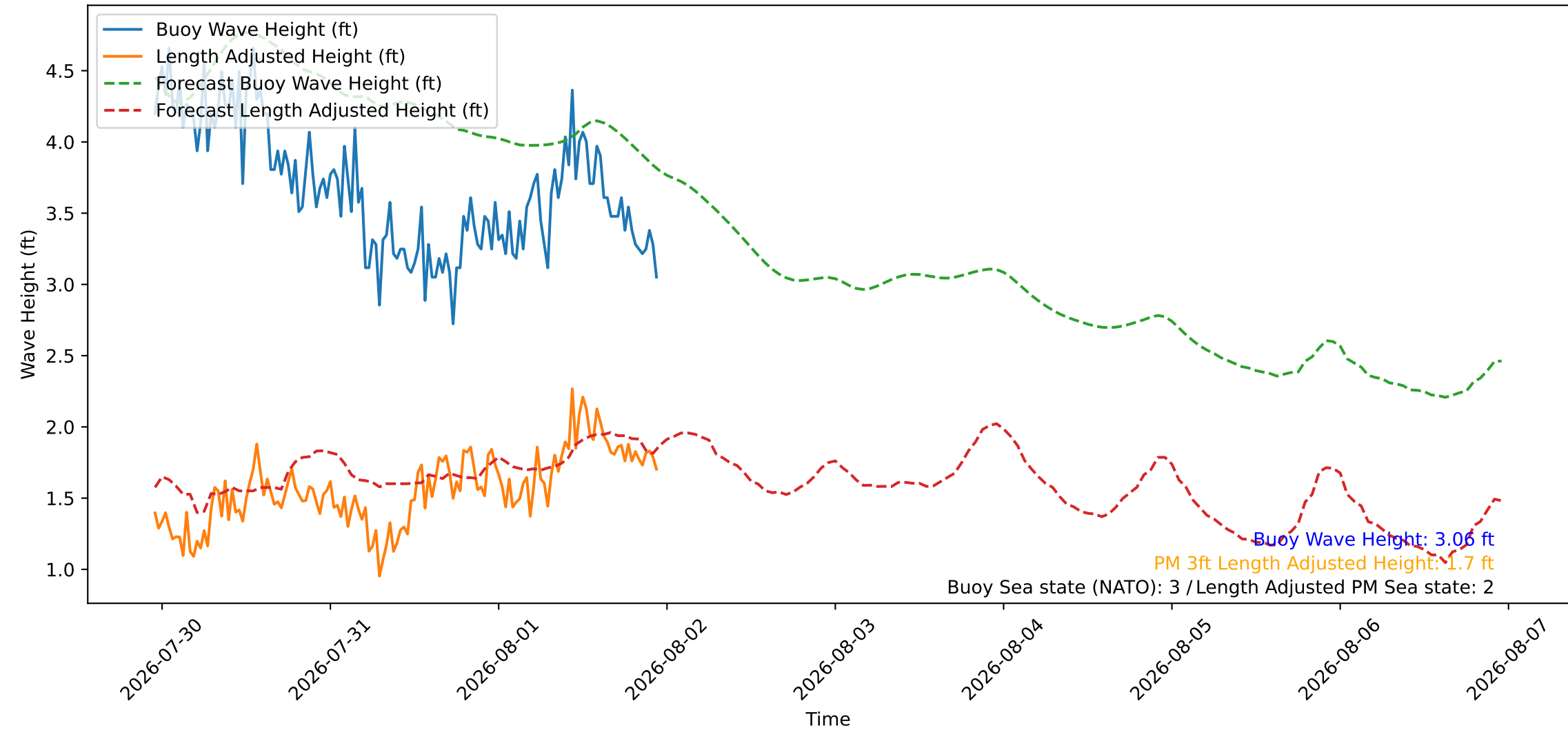
Wave Heights over Time for Oceanside Harbor at 2026-08-01 23:10:26
