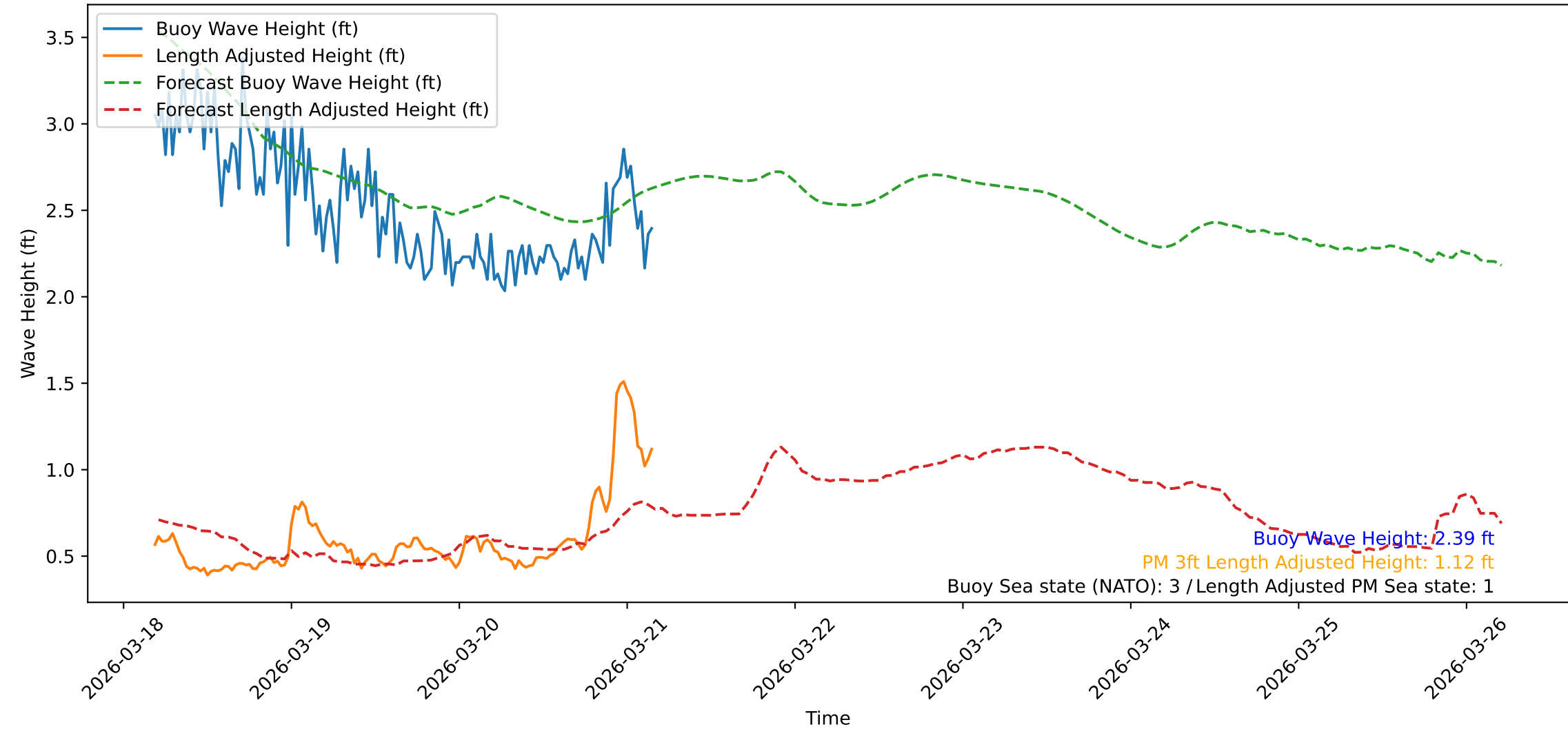
Wave Heights over Time for Green Beach at 2026-03-21 04:31:10
