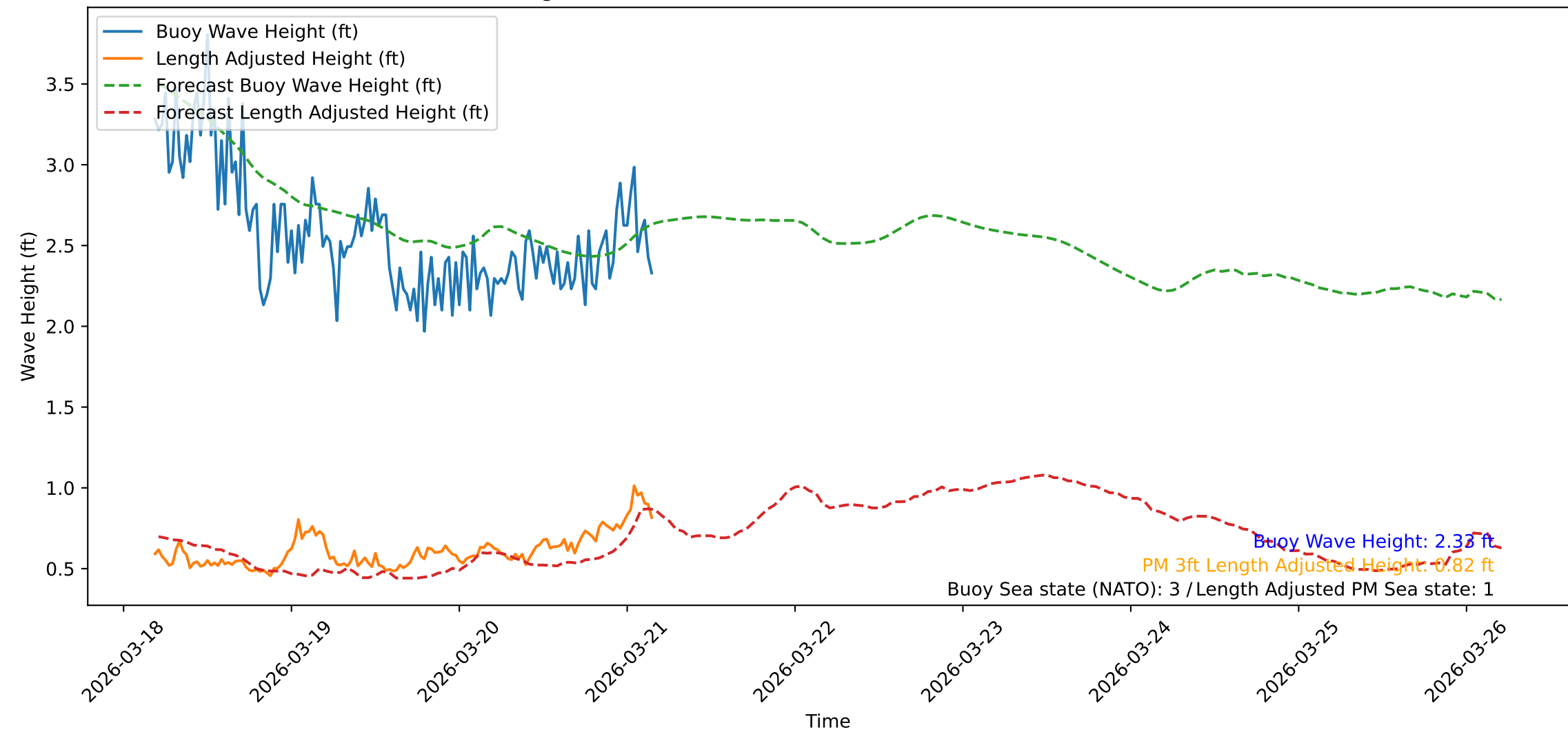
Wave Heights over Time for Oceanside Harbor at 2026-03-21 04:30:32
