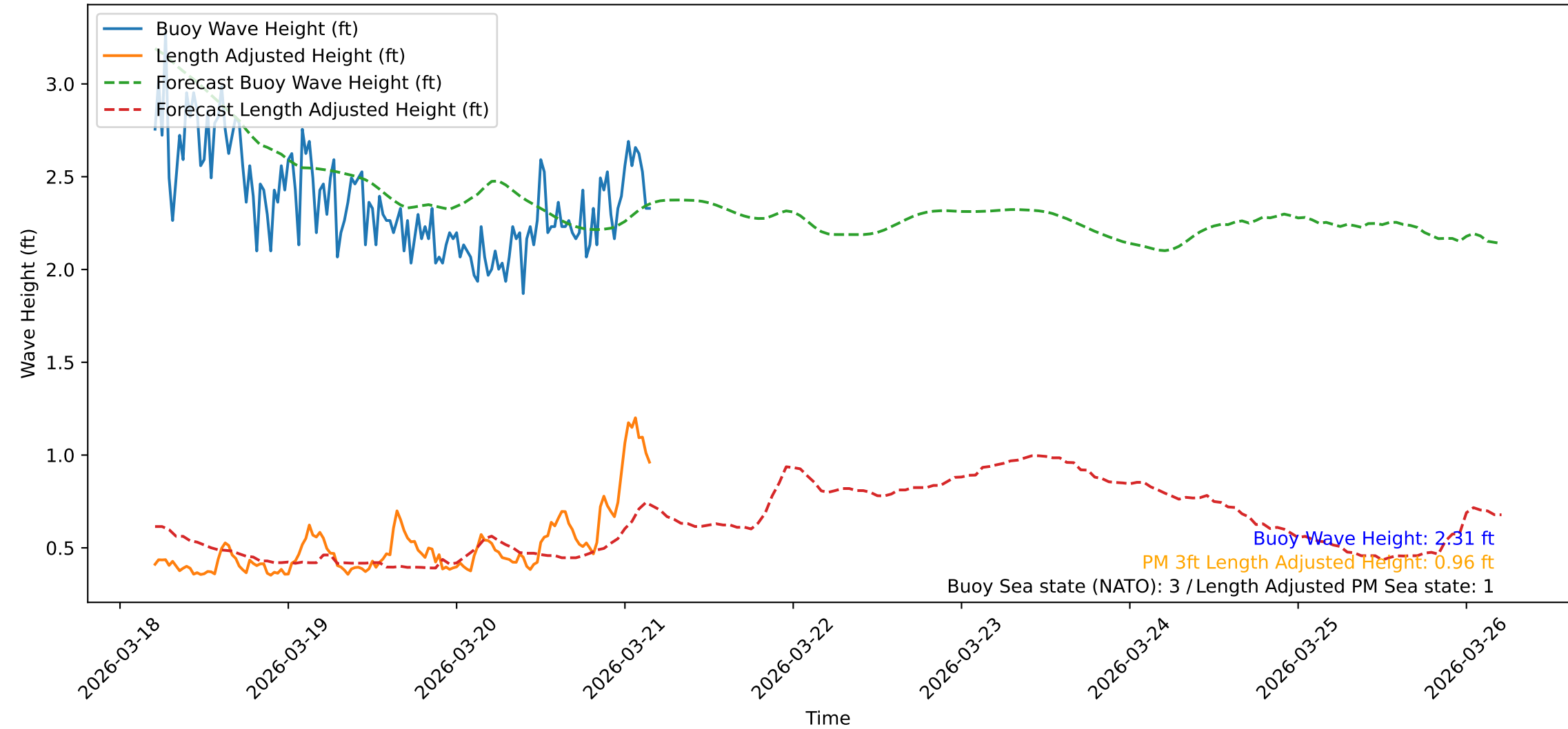
Wave Heights over Time for Red Beach at 2026-03-21 04:30:48
