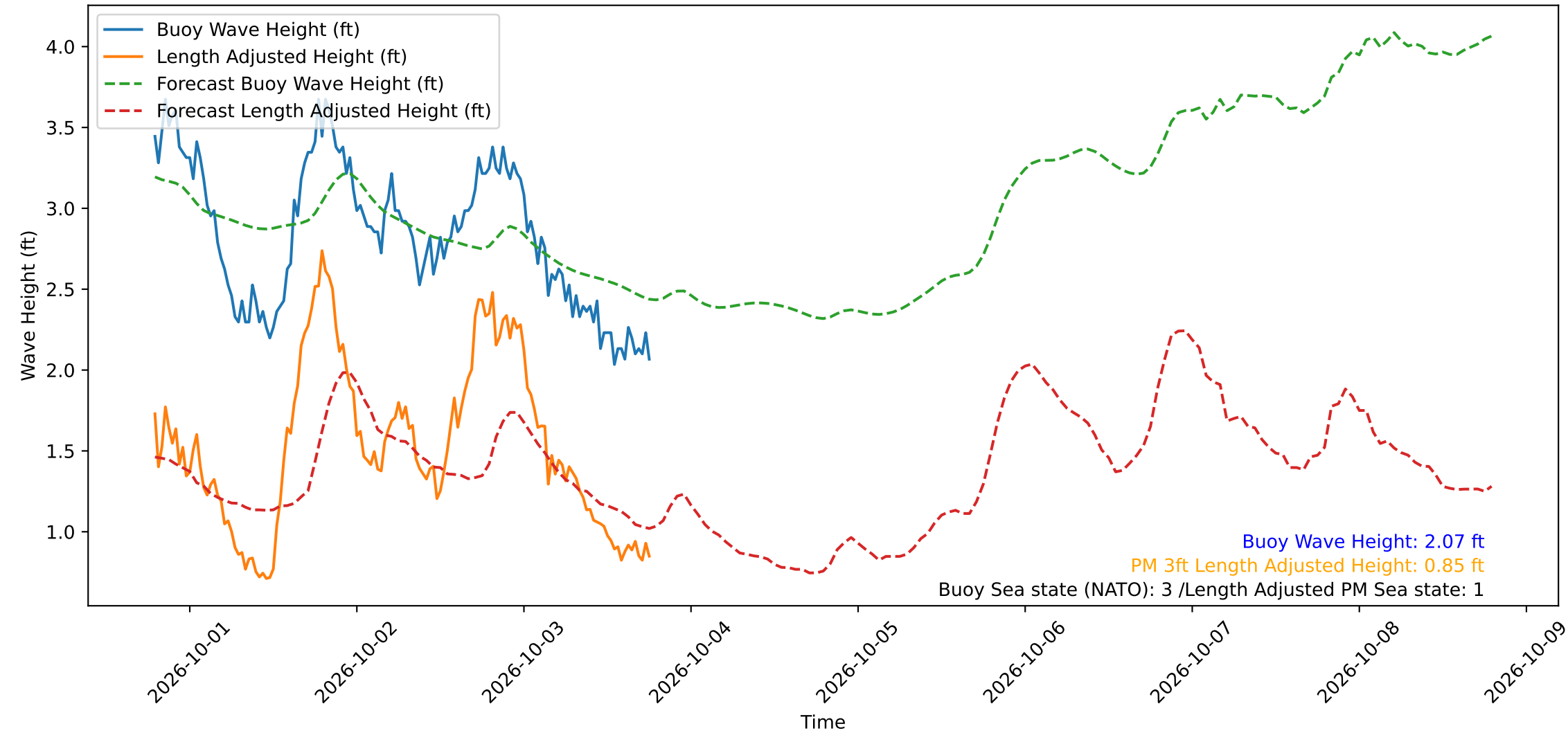
Wave Heights over Time for Green Beach at 2026-10-03 18:41:11
