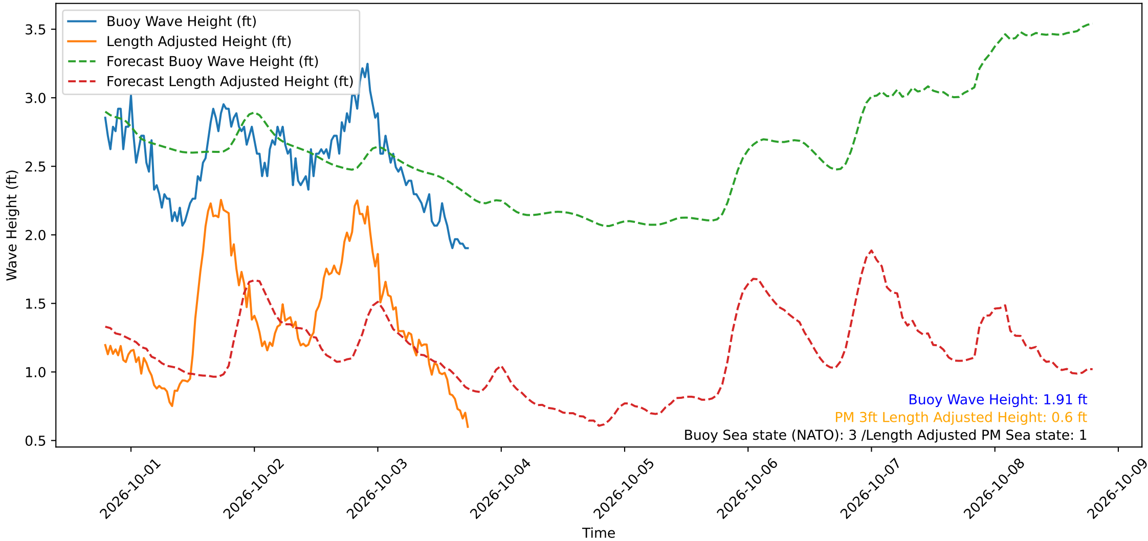
Wave Heights over Time for Red Beach at 2026-10-03 18:40:49
