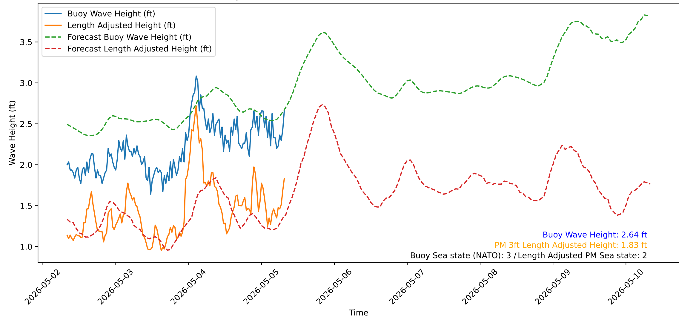
Wave Heights over Time for Oceanside Harbor at 2026-05-05 08:10:32
