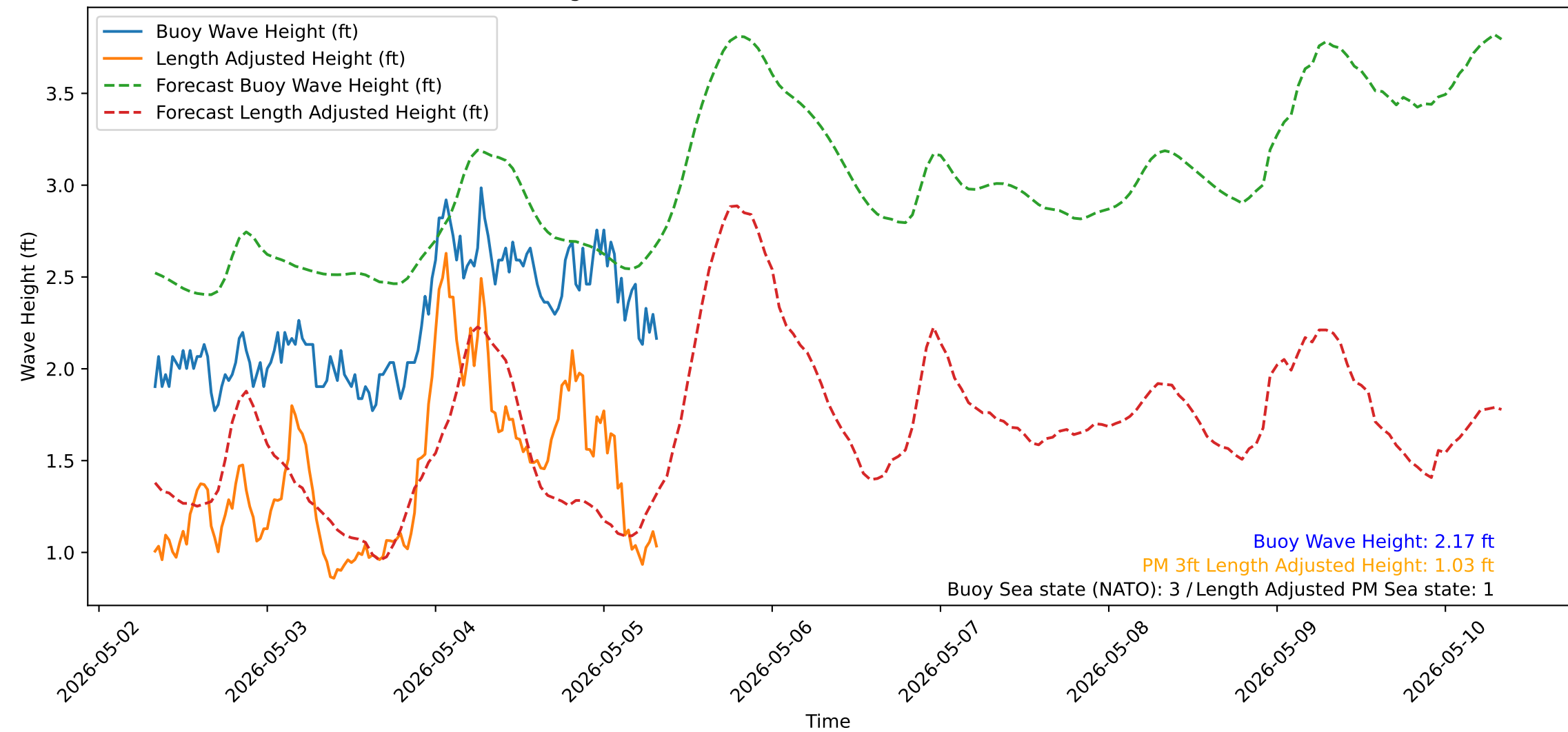
Wave Heights over Time for Green Beach at 2026-05-05 08:11:14
