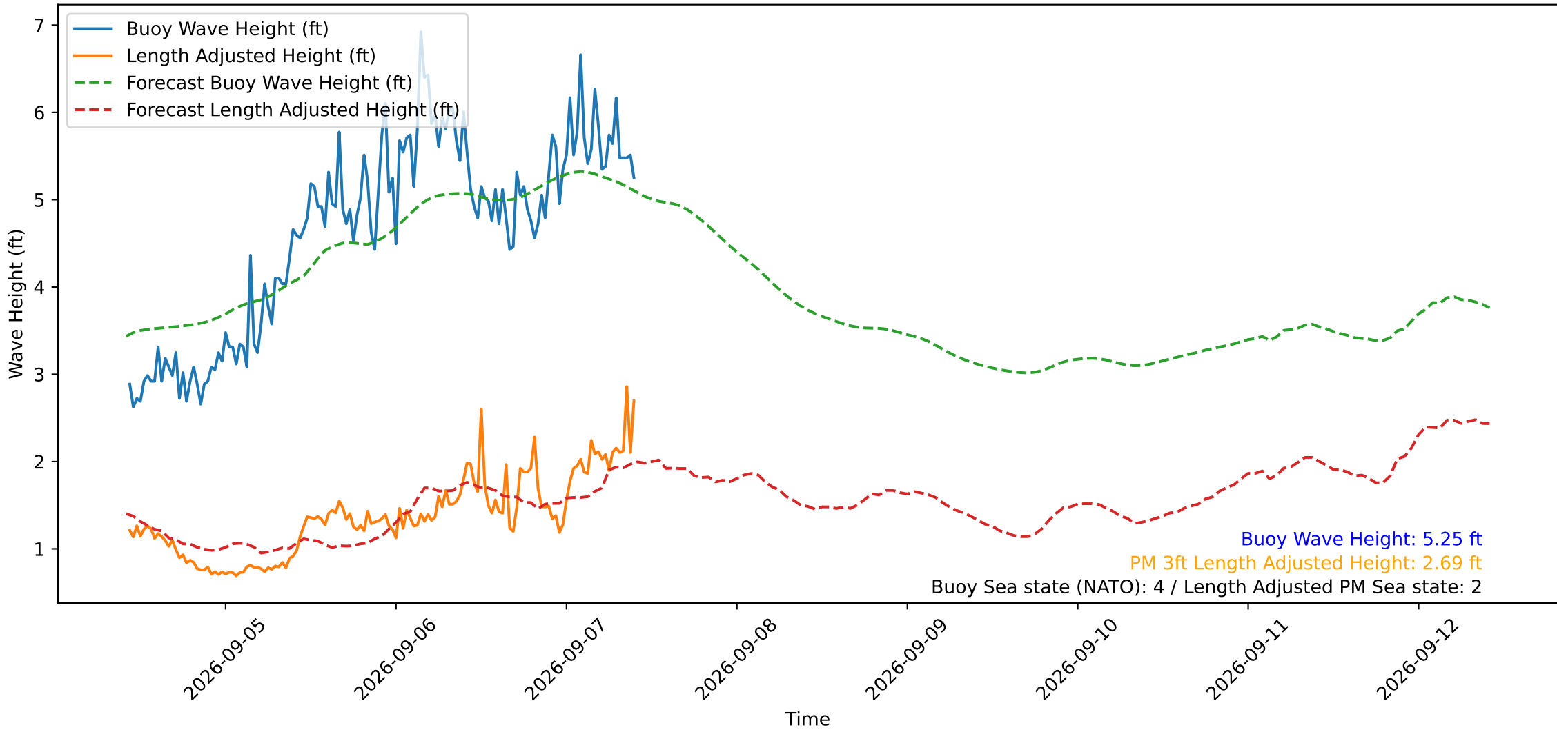
Wave Heights over Time for Red Beach at 2026-09-07 10:10:49
