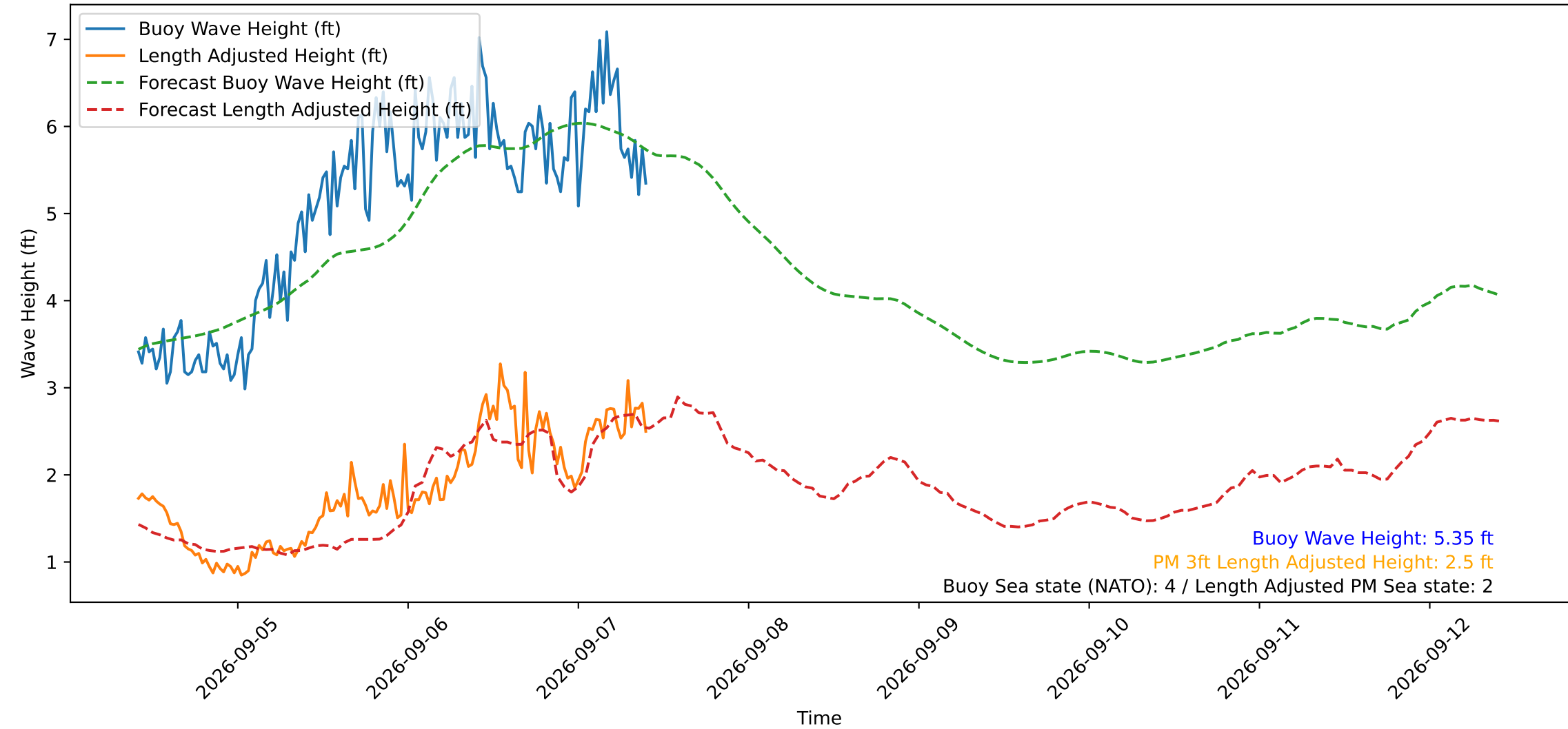
Wave Heights over Time for Oceanside Harbor at 2026-09-07 10:10:30
