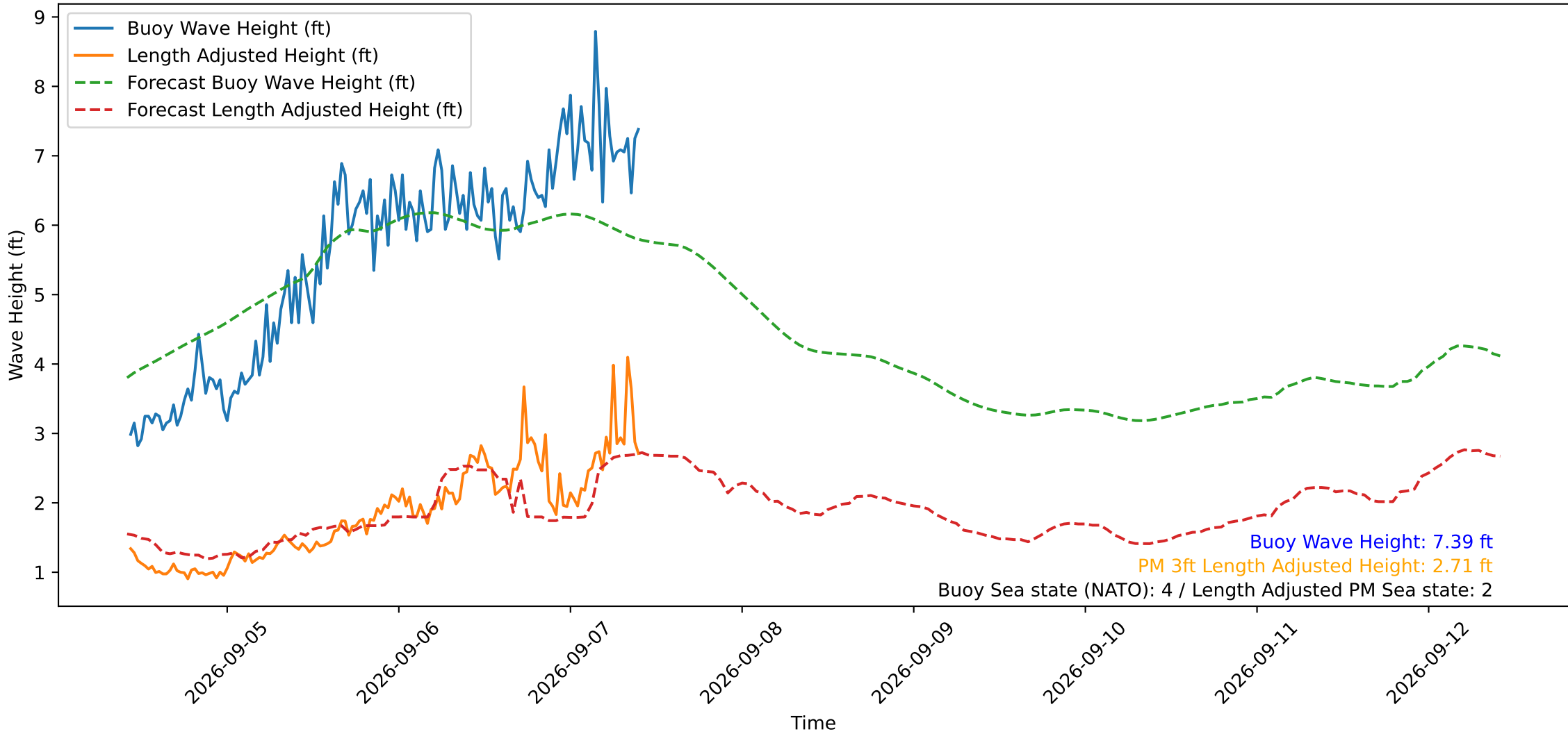
Wave Heights over Time for Green Beach at 2026-09-07 10:11:12
