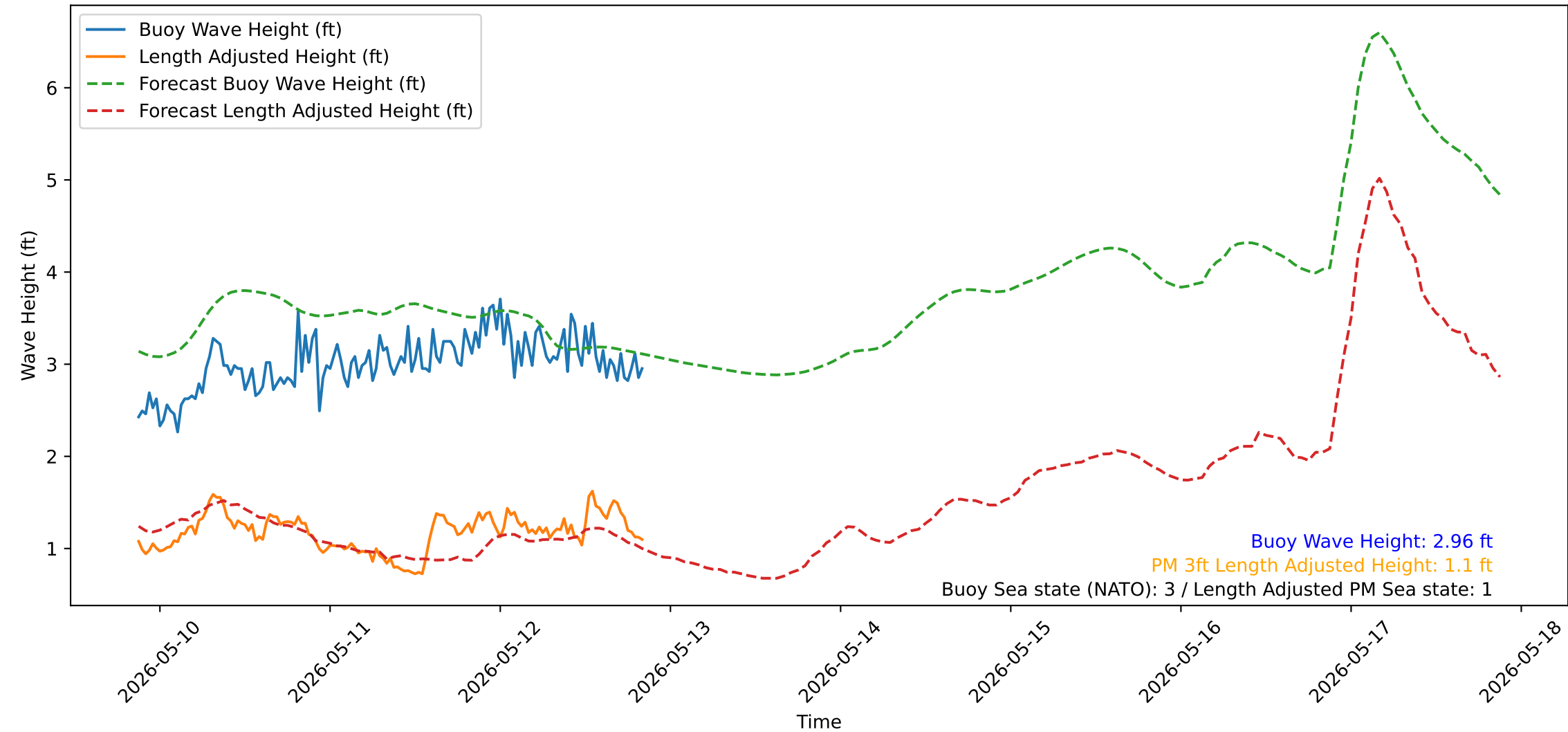
Wave Heights over Time for Oceanside Harbor at 2026-05-12 21:00:31
