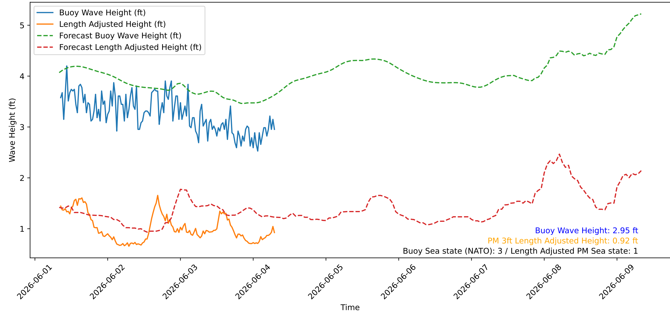
Wave Heights over Time for Red Beach at 2026-06-04 08:00:45
