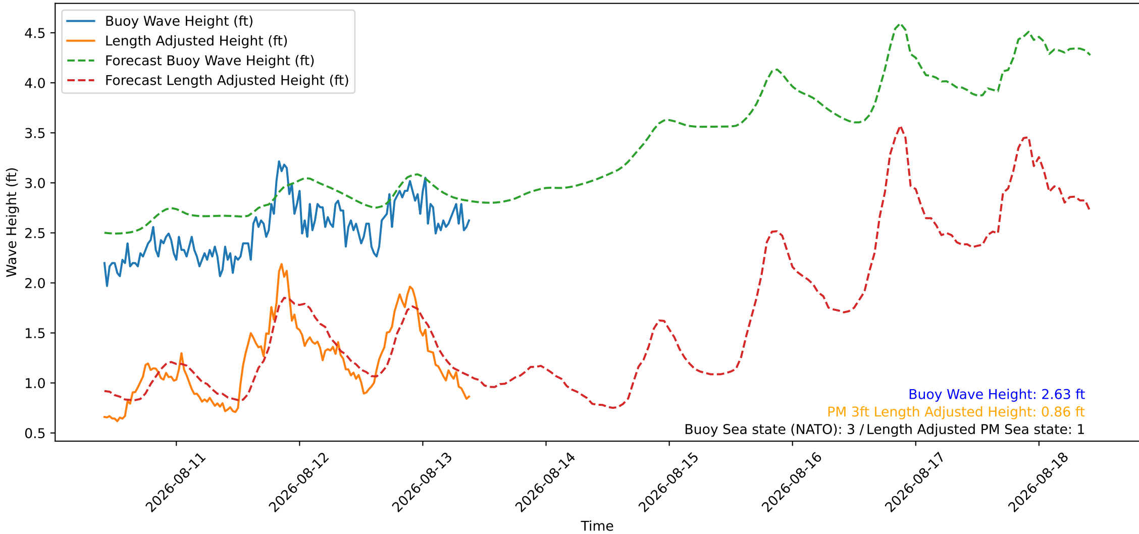
Wave Heights over Time for Green Beach at 2026-08-13 10:01:07
