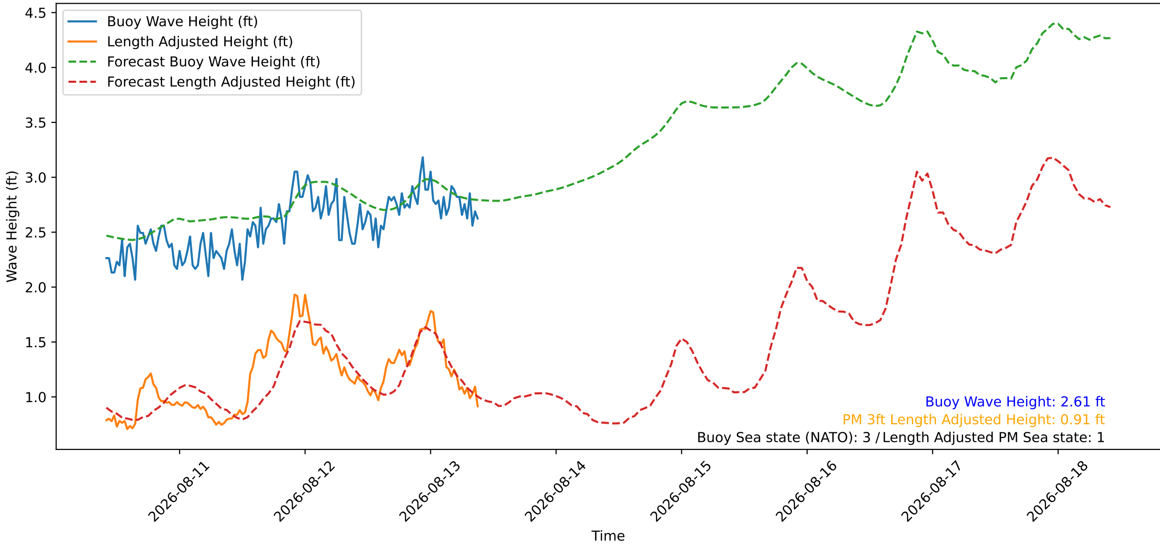
Wave Heights over Time for Oceanside Harbor at 2026-08-13 10:00:26
