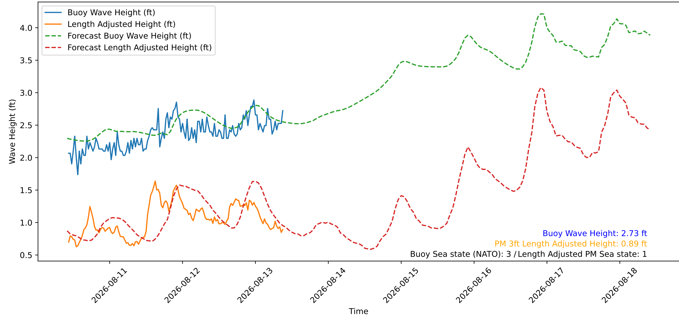
Wave Heights over Time for Red Beach at 2026-08-13 10:00:45
