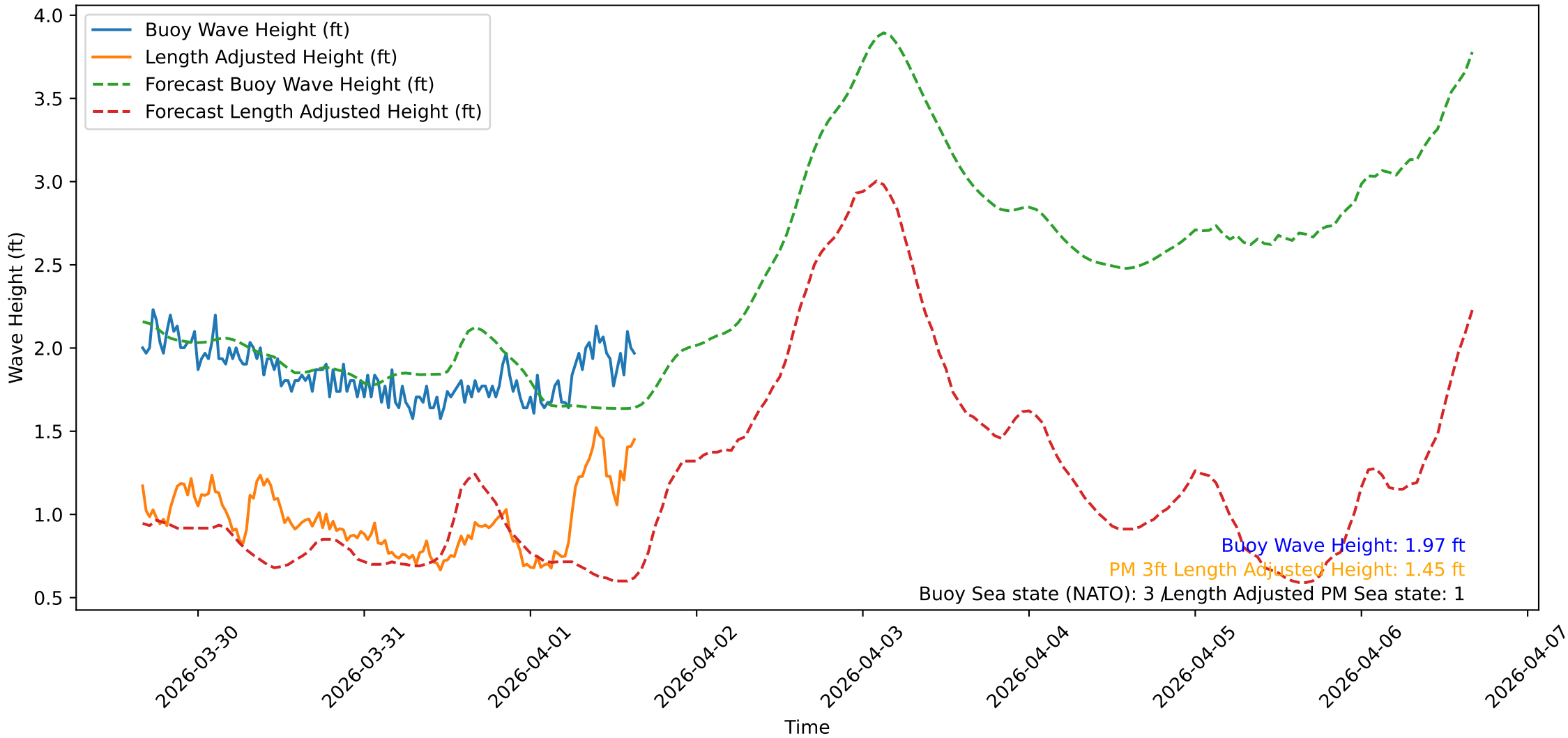
Wave Heights over Time for Oceanside Harbor at 2026-04-01 15:50:30
