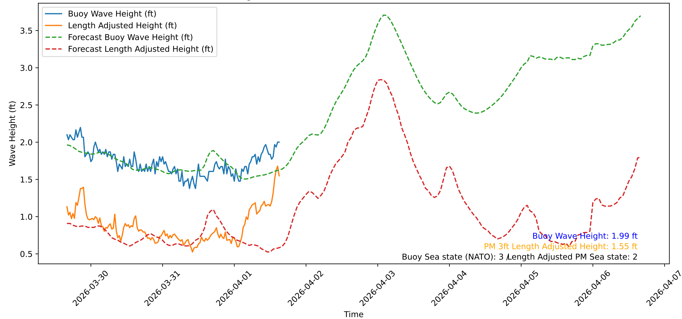
Wave Heights over Time for Red Beach at 2026-04-01 15:50:47
