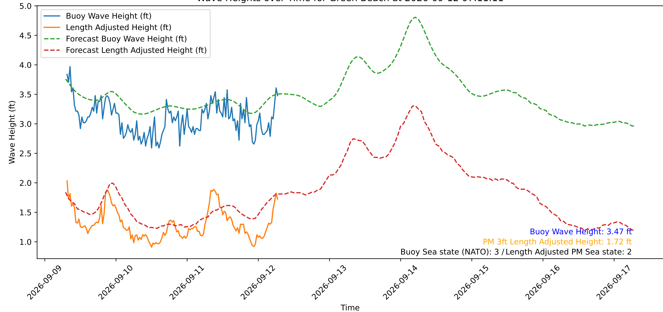
Wave Heights over Time for Green Beach at 2026-09-12 07:11:11
