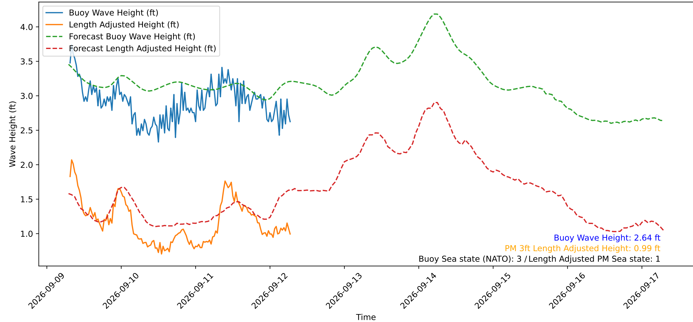
Wave Heights over Time for Red Beach at 2026-09-12 07:10:48
