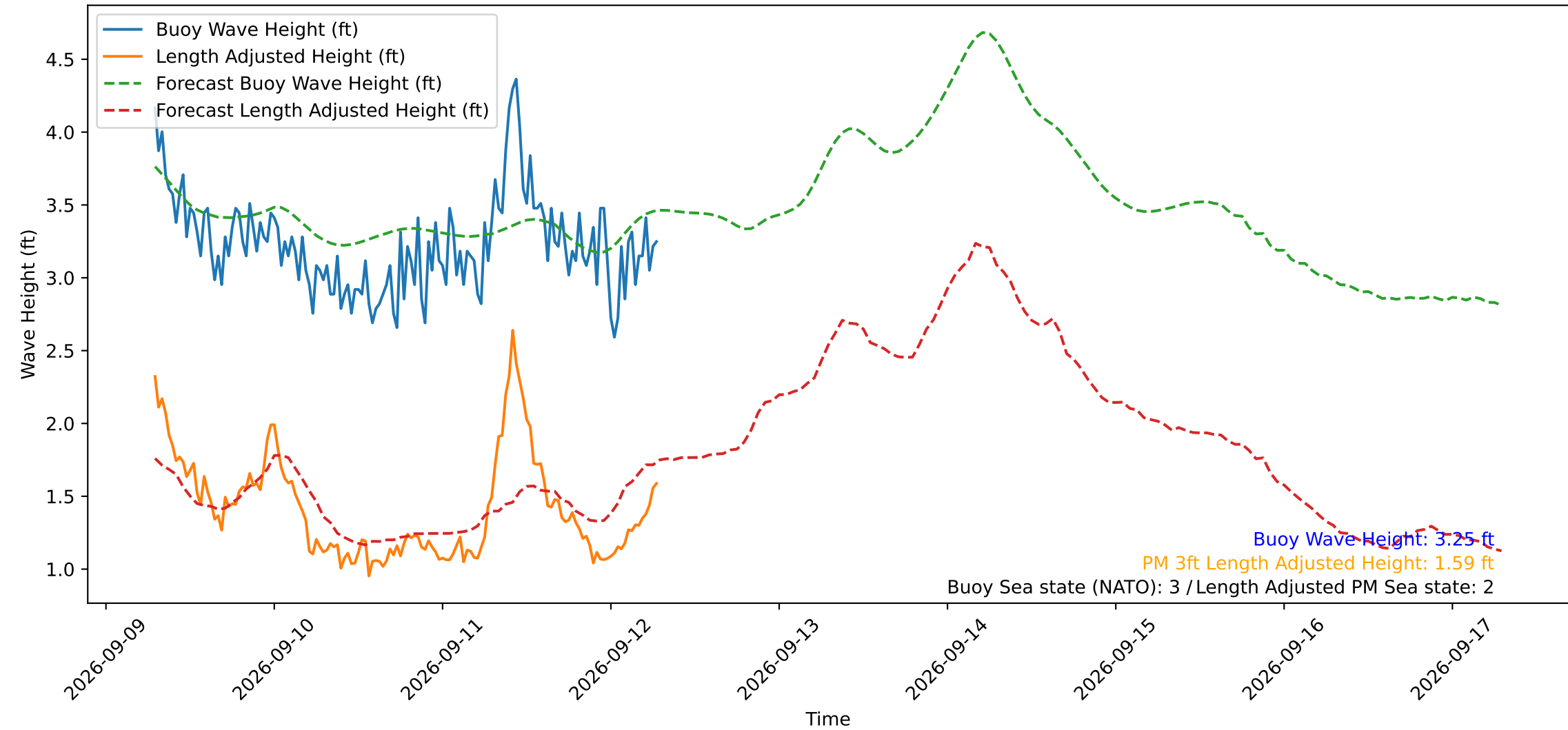
Wave Heights over Time for Oceanside Harbor at 2026-09-12 07:10:29
