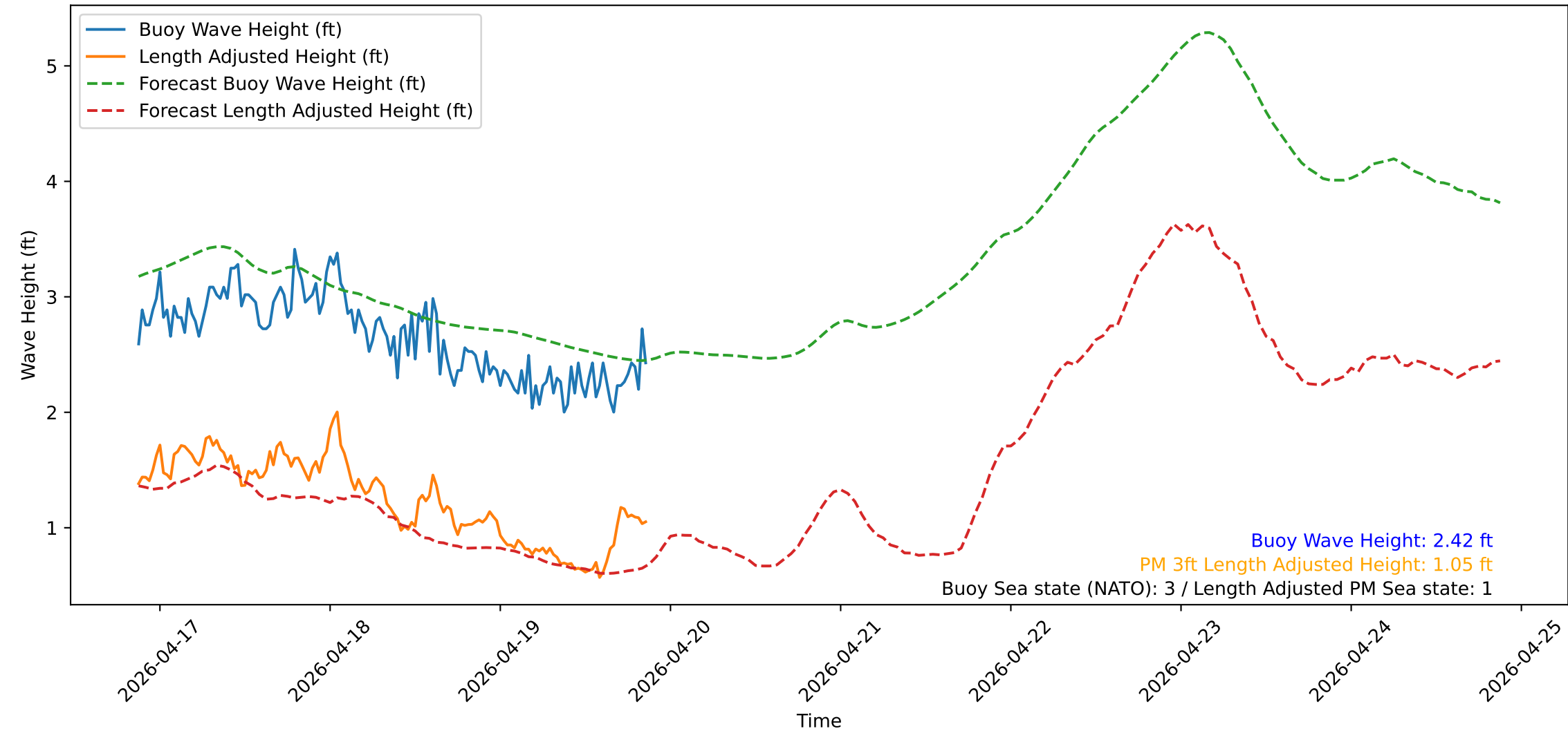
Wave Heights over Time for Oceanside Harbor at 2026-04-19 21:10:31
