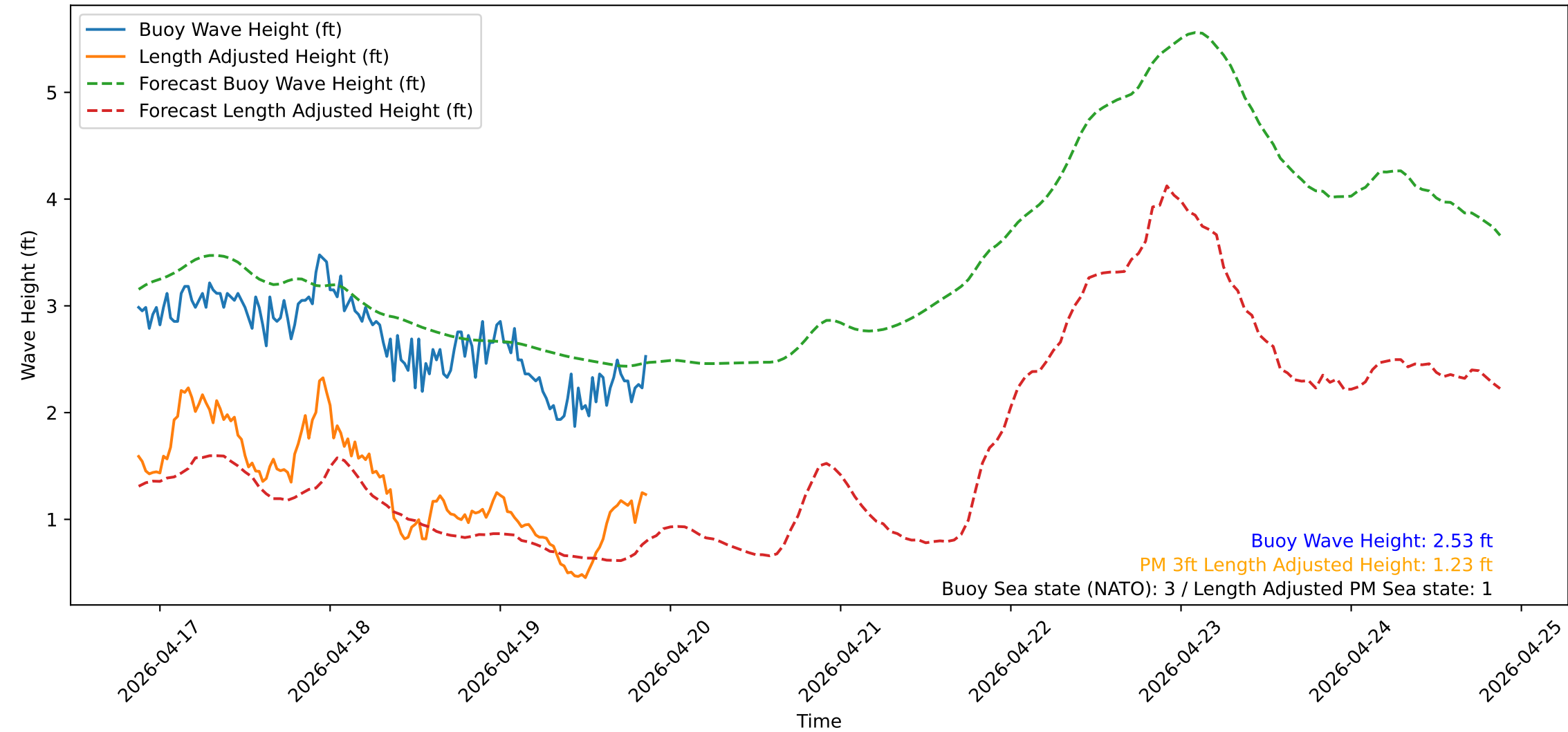
Wave Heights over Time for Green Beach at 2026-04-19 21:11:13
