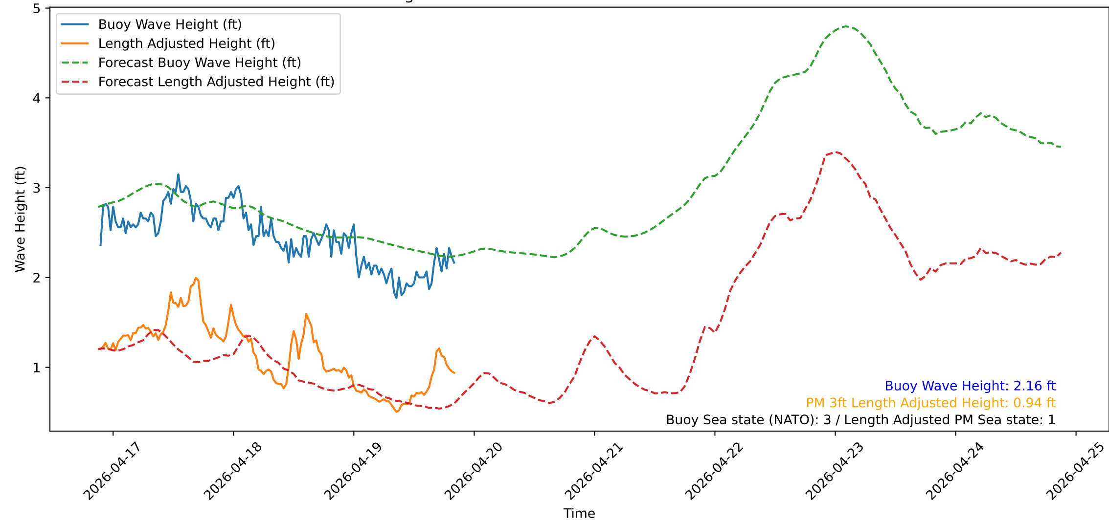
Wave Heights over Time for Red Beach at 2026-04-19 21:10:50
