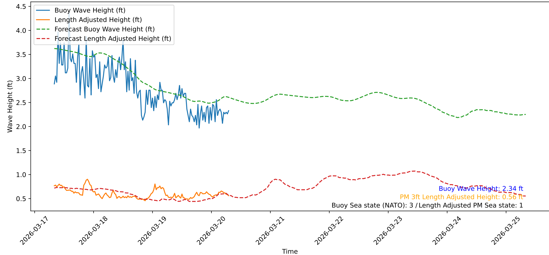
Wave Heights over Time for Oceanside Harbor at 2026-03-20 07:50:31
