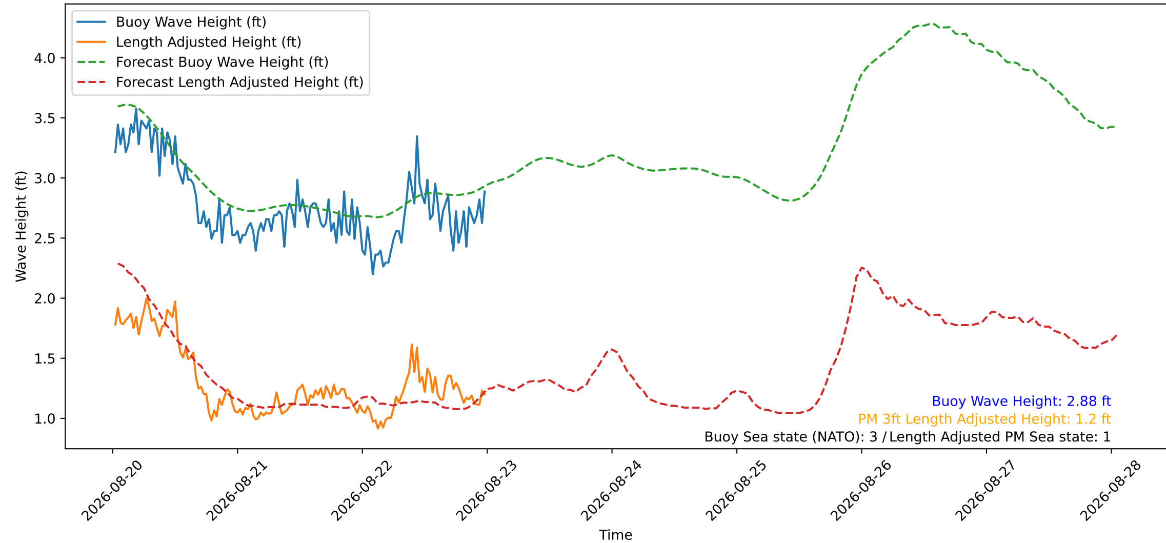
Wave Heights over Time for Oceanside Harbor at 2026-08-23 00:40:30
