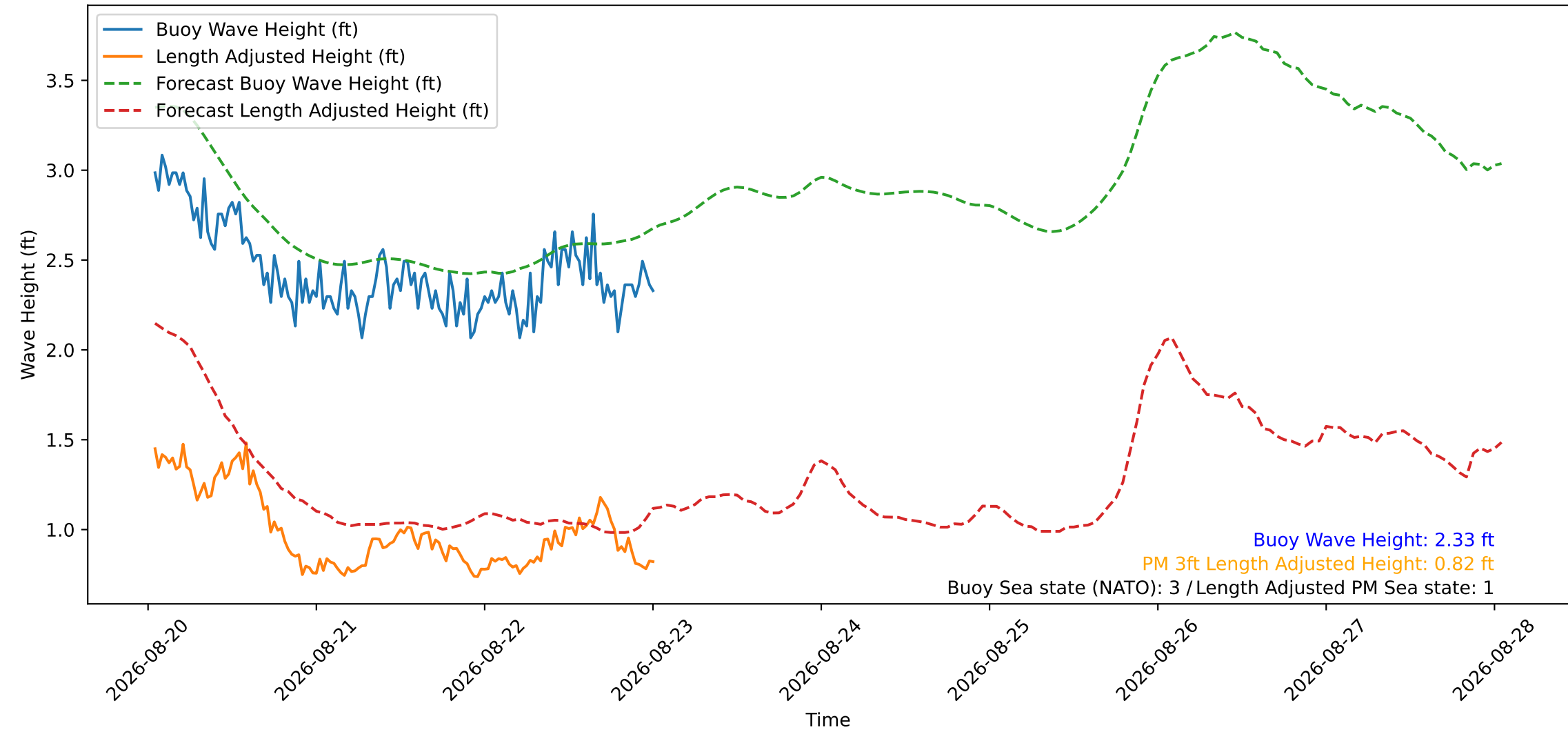
Wave Heights over Time for Red Beach at 2026-08-23 00:40:49
