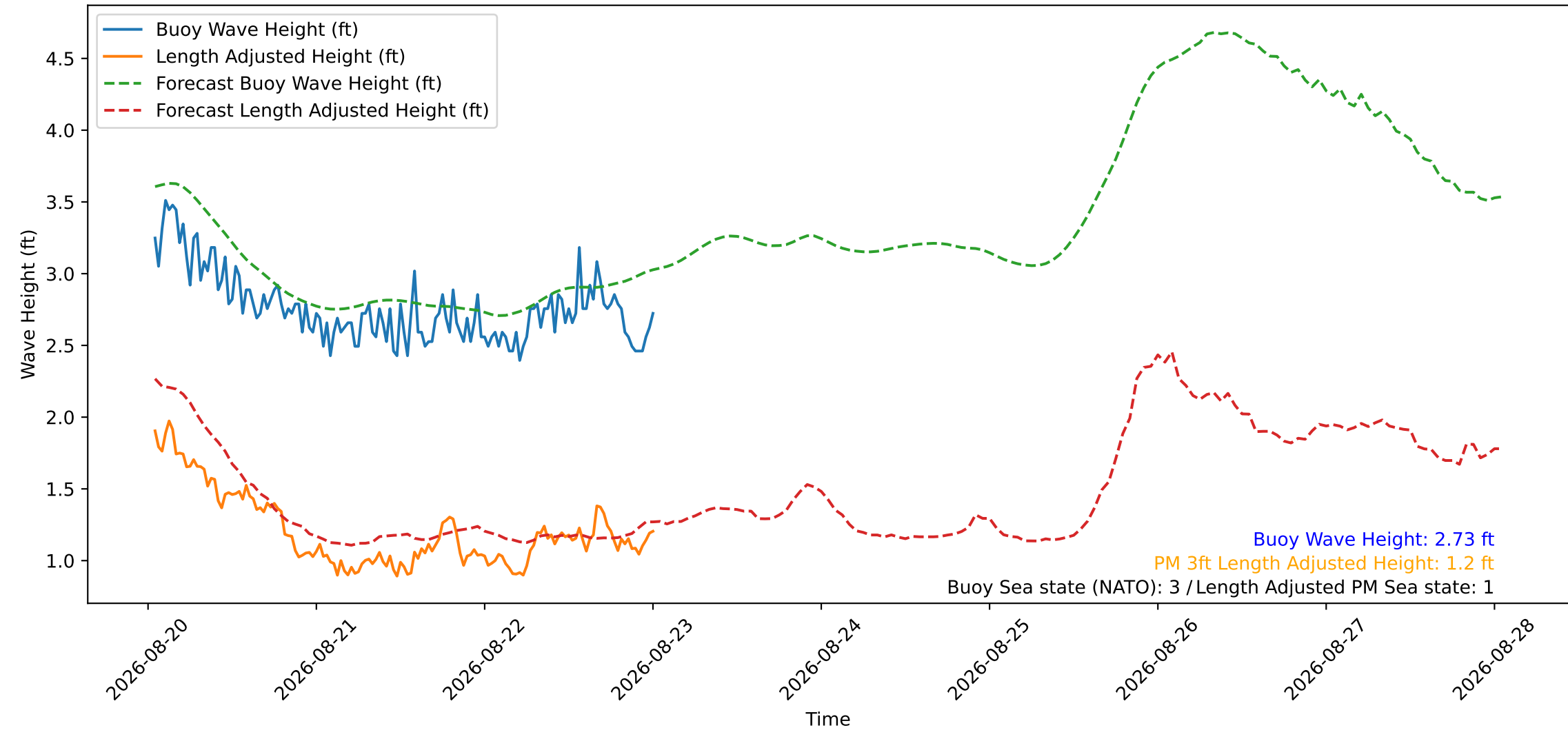
Wave Heights over Time for Green Beach at 2026-08-23 00:41:12
