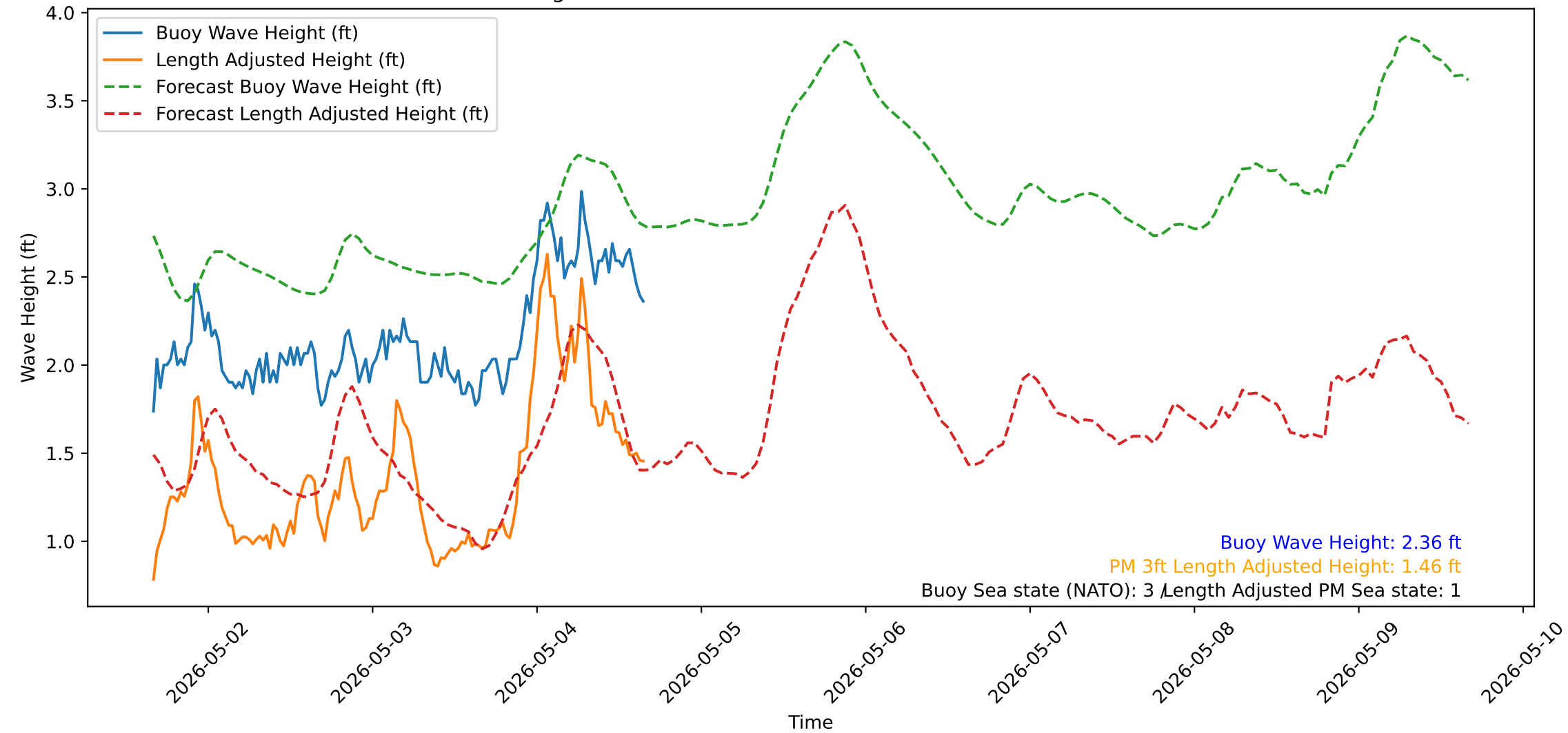
Wave Heights over Time for Green Beach at 2026-05-04 16:11:13
