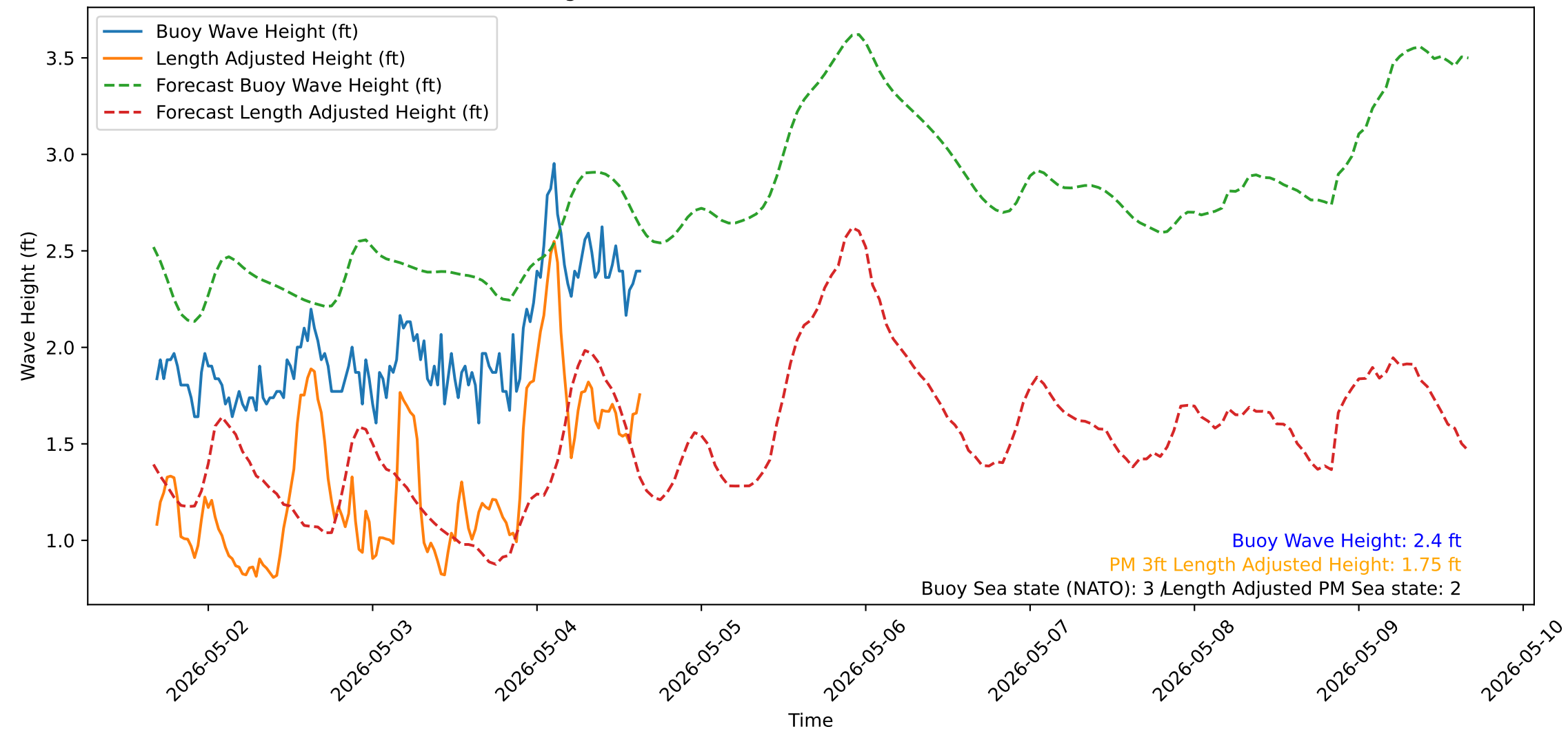
Wave Heights over Time for Red Beach at 2026-05-04 16:10:51
