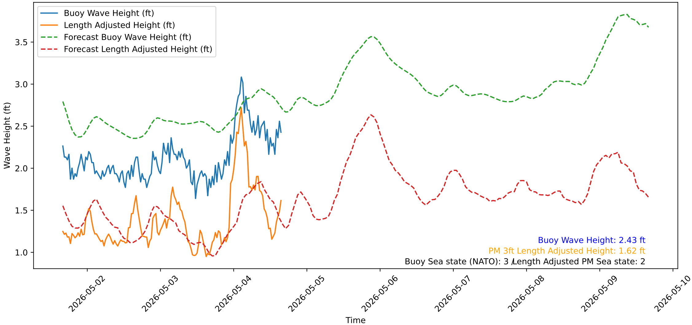
Wave Heights over Time for Oceanside Harbor at 2026-05-04 16:10:32
