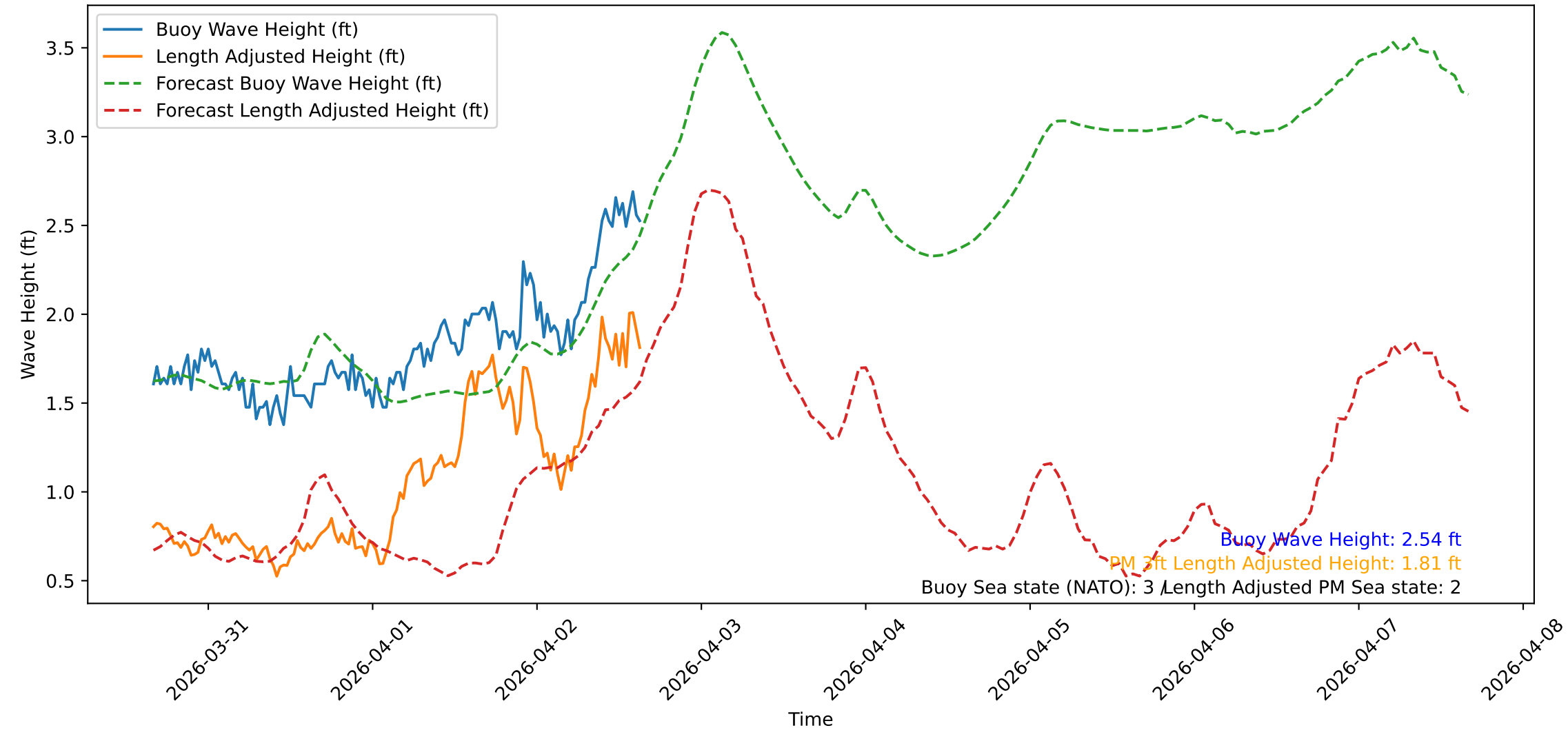
Wave Heights over Time for Red Beach at 2026-04-02 15:50:51
