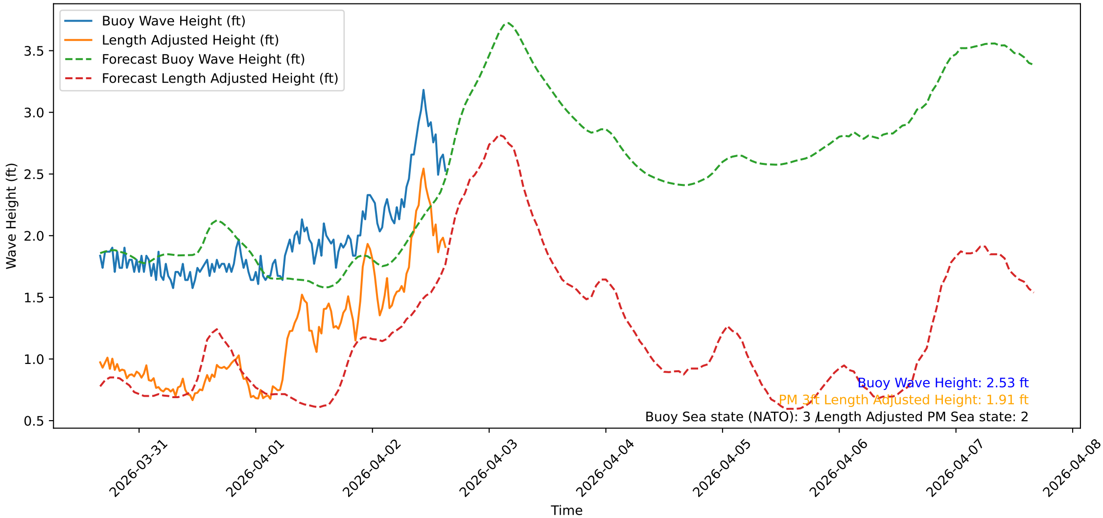
Wave Heights over Time for Oceanside Harbor at 2026-04-02 15:50:35
