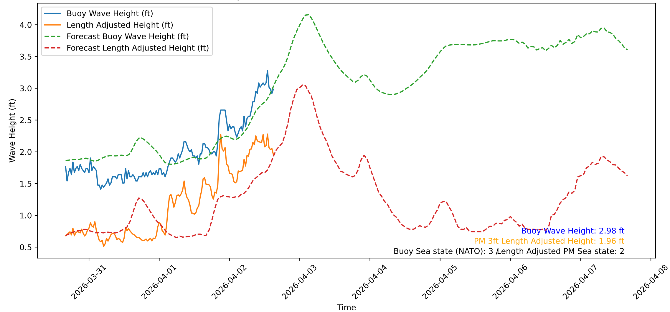
Wave Heights over Time for Green Beach at 2026-04-02 15:51:13
