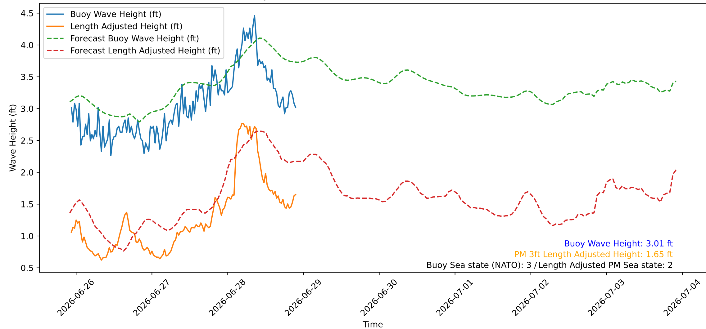
Wave Heights over Time for Red Beach at 2026-06-28 22:20:46
