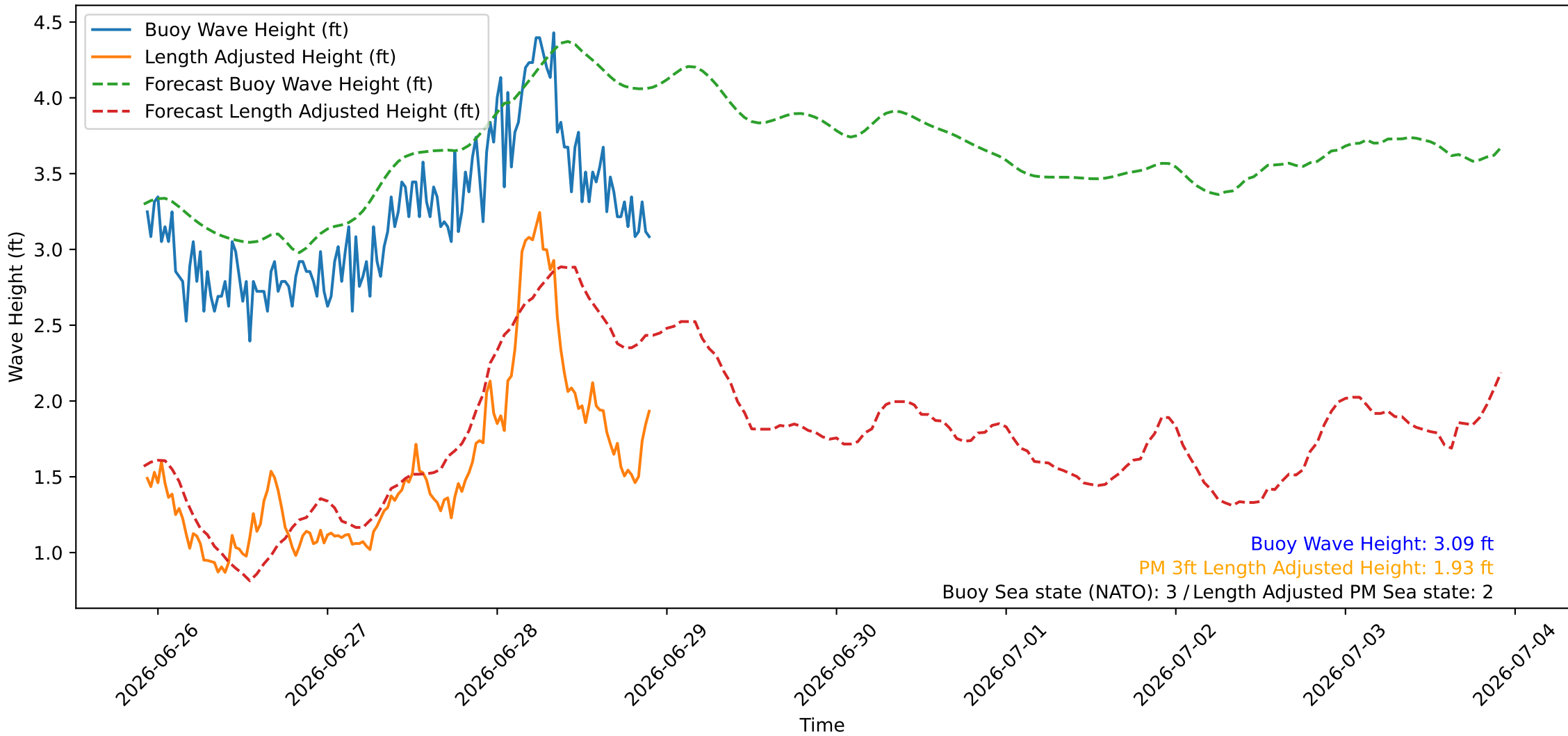
Wave Heights over Time for Oceanside Harbor at 2026-06-28 22:20:26
