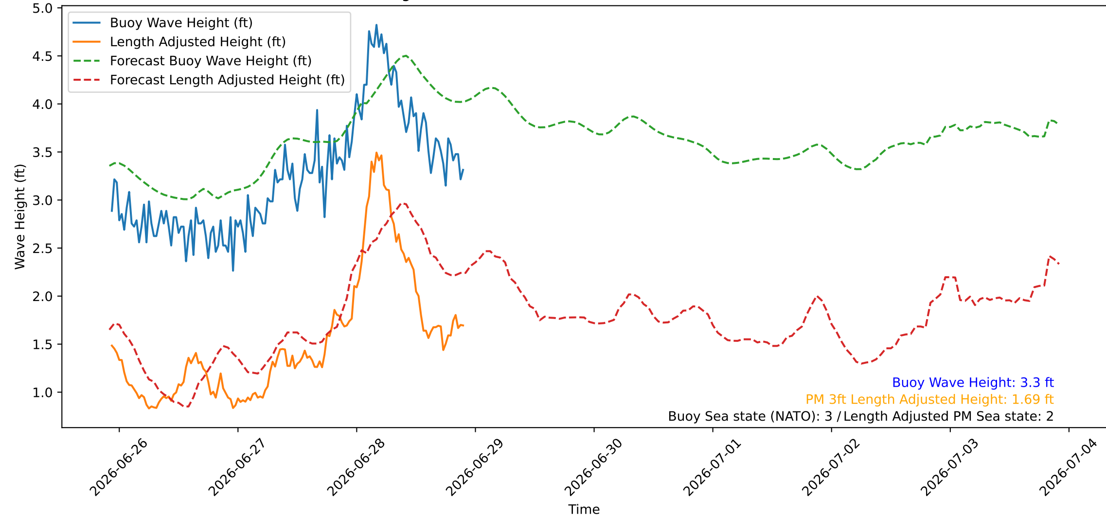
Wave Heights over Time for Green Beach at 2026-06-28 22:21:09
