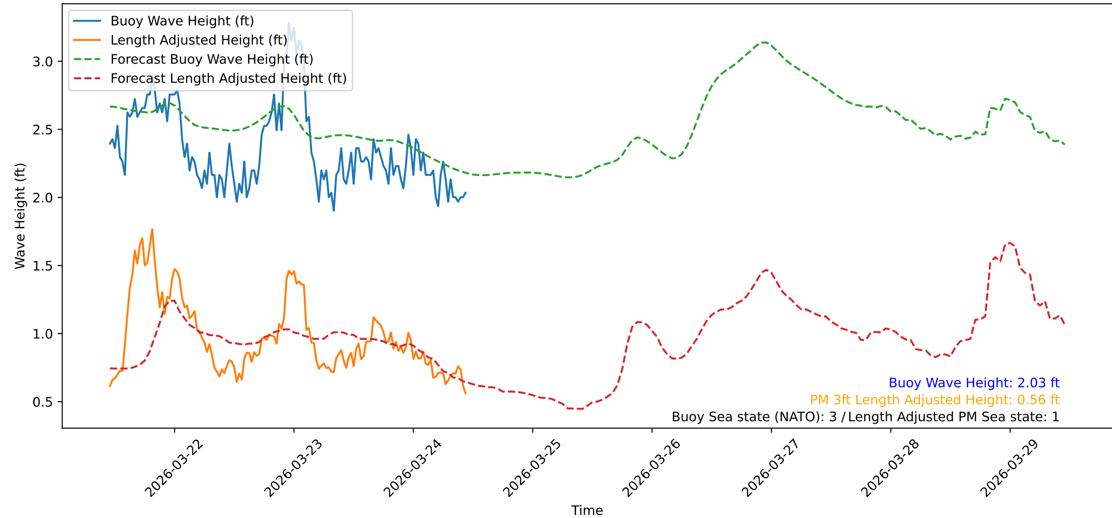
Wave Heights over Time for Green Beach at 2026-03-24 11:11:09
