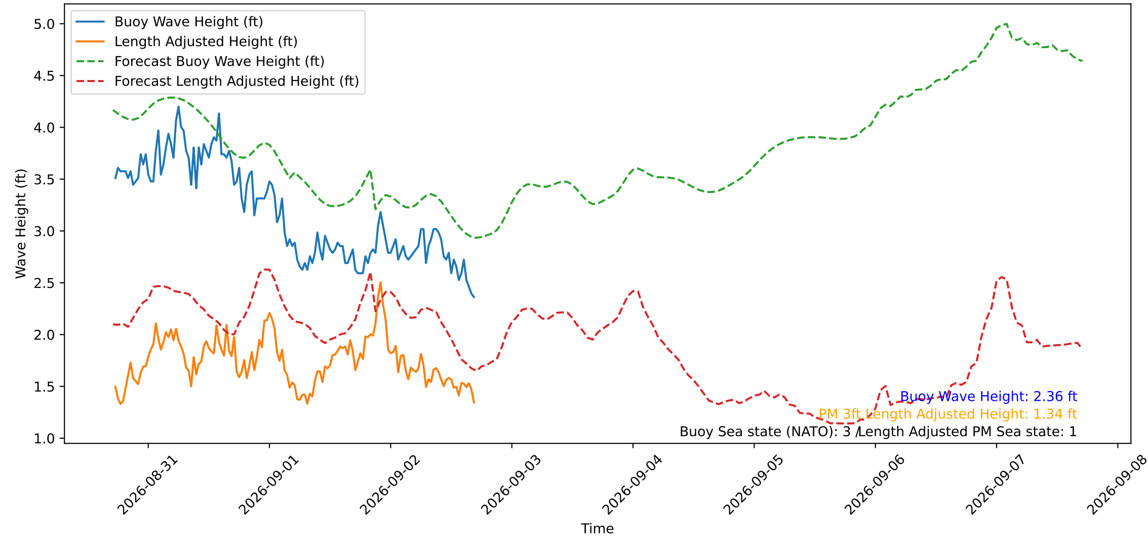
Wave Heights over Time for Red Beach at 2026-09-02 17:10:50
