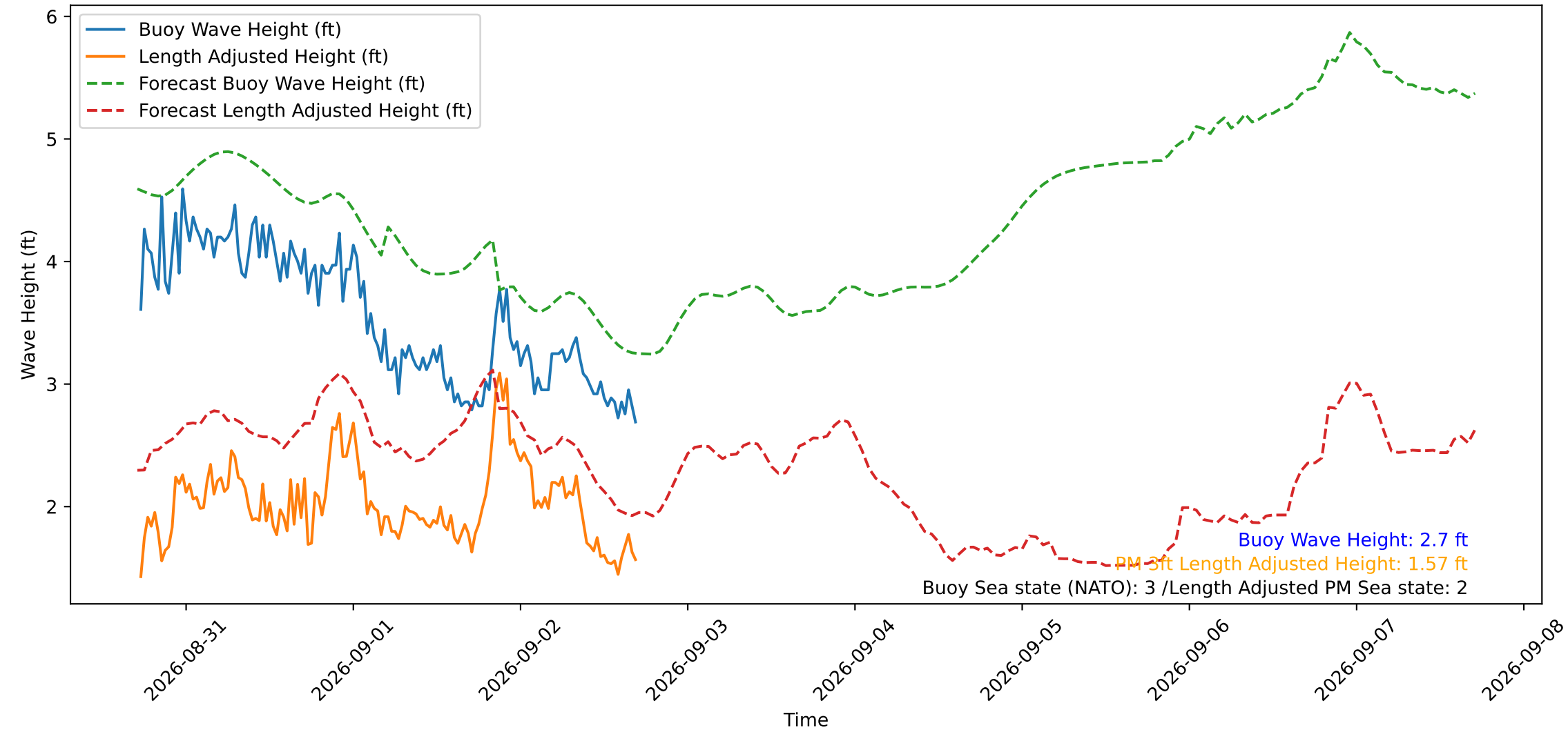
Wave Heights over Time for Green Beach at 2026-09-02 17:11:13
