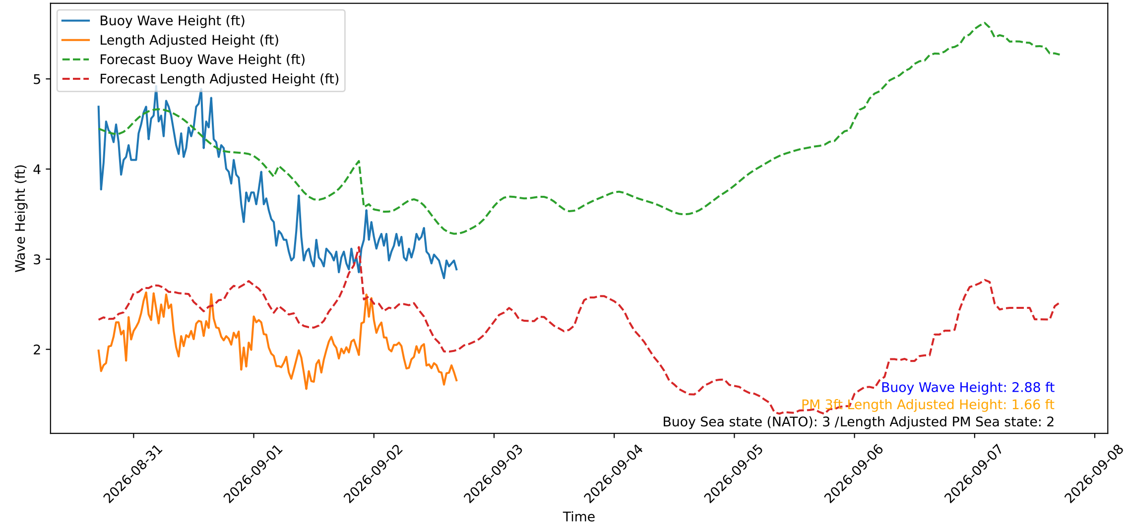
Wave Heights over Time for Oceanside Harbor at 2026-09-02 17:10:30
