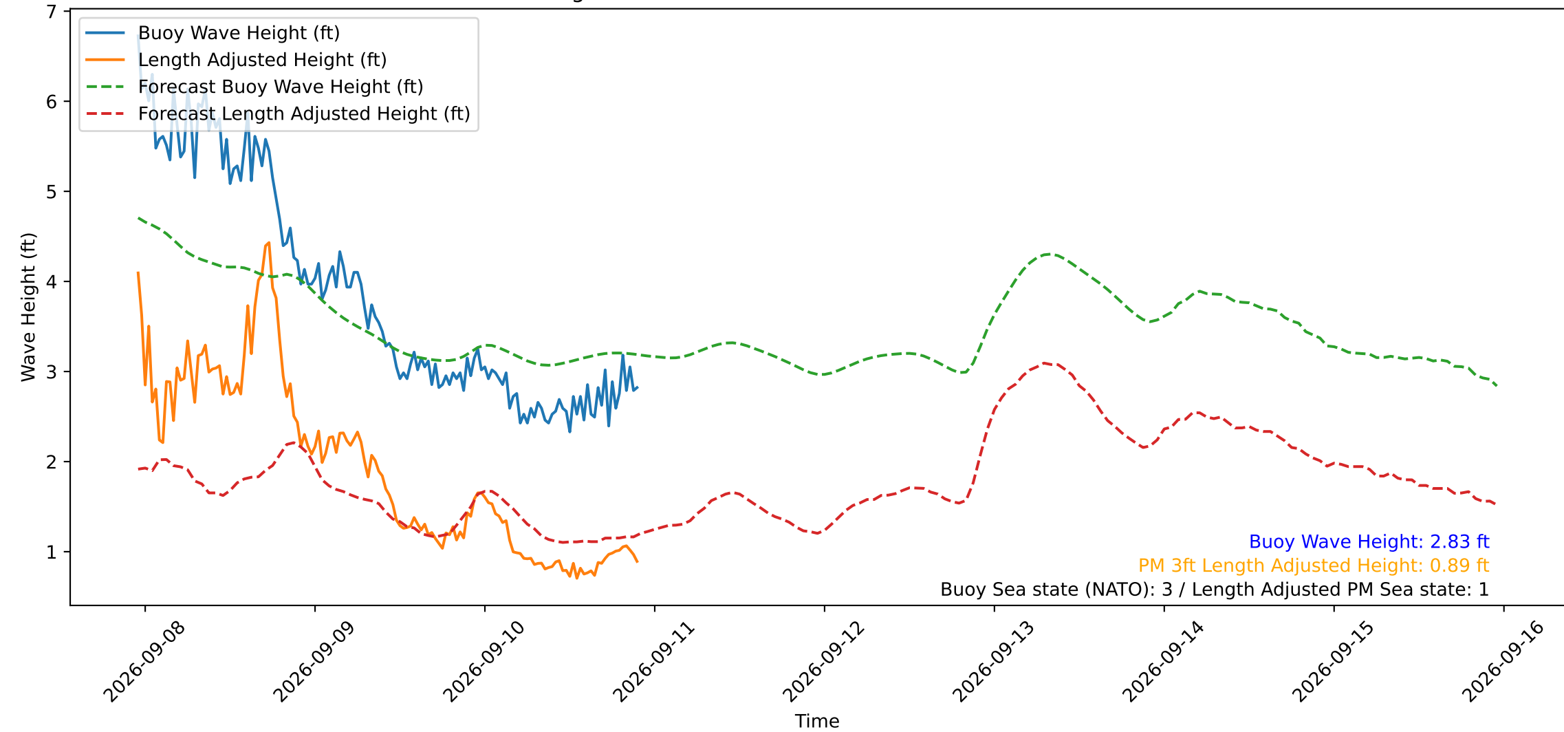
Wave Heights over Time for Red Beach at 2026-09-10 22:40:49
