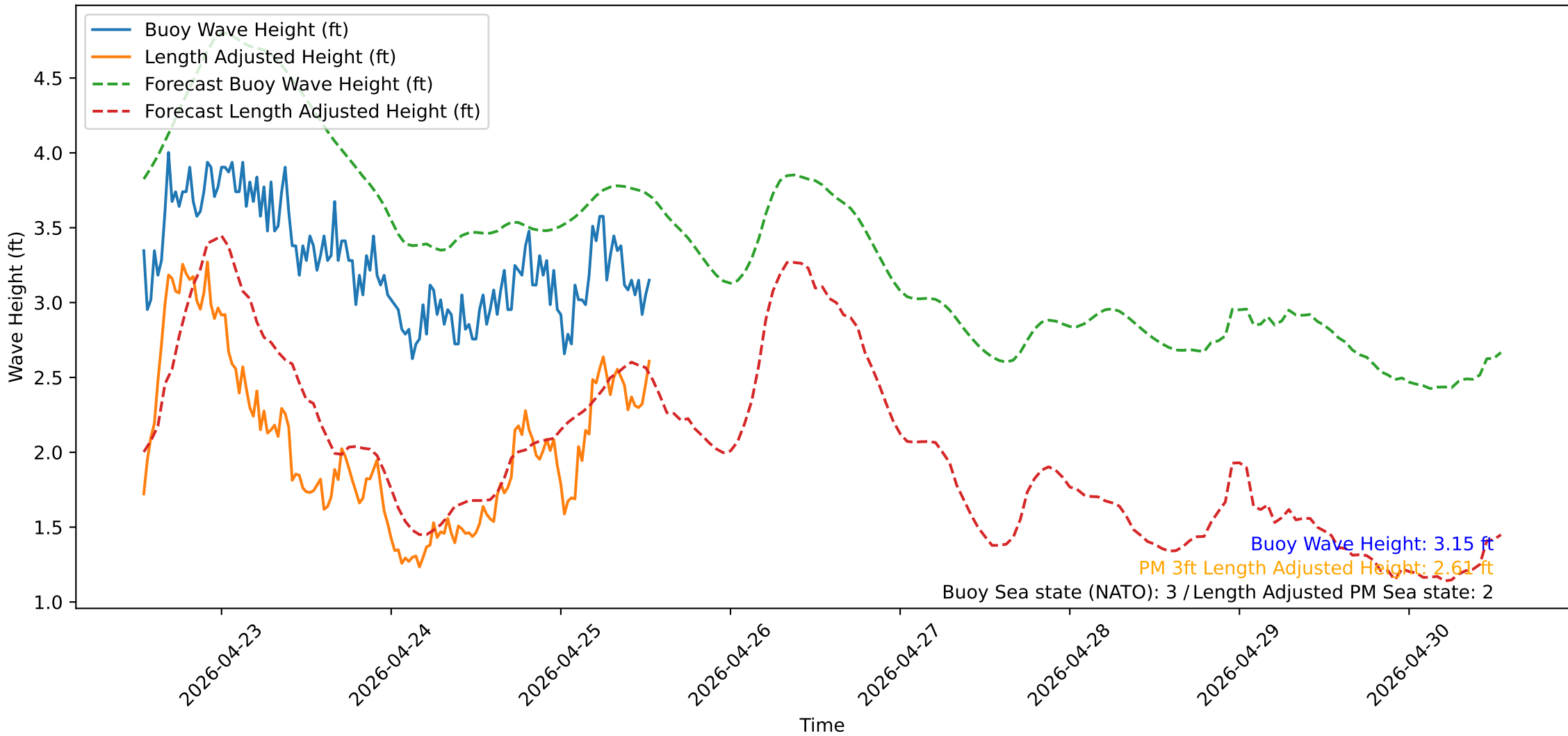
Wave Heights over Time for Green Beach at 2026-04-25 13:11:12
