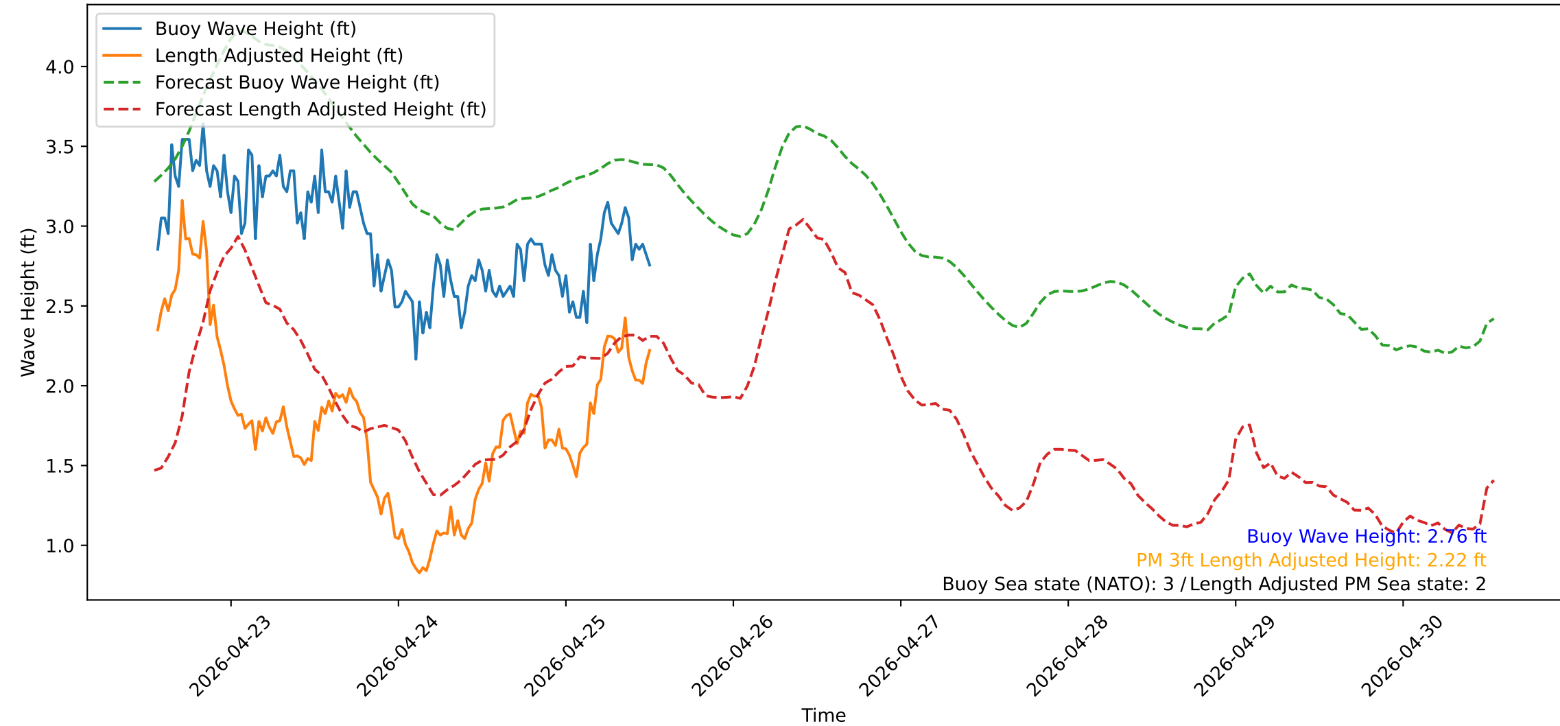
Wave Heights over Time for Red Beach at 2026-04-25 13:10:50
