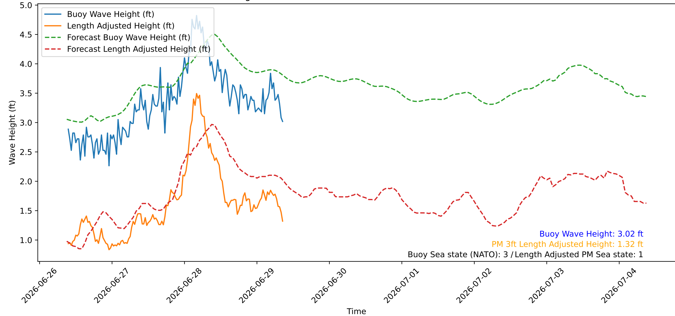
Wave Heights over Time for Green Beach at 2026-06-29 09:21:09
