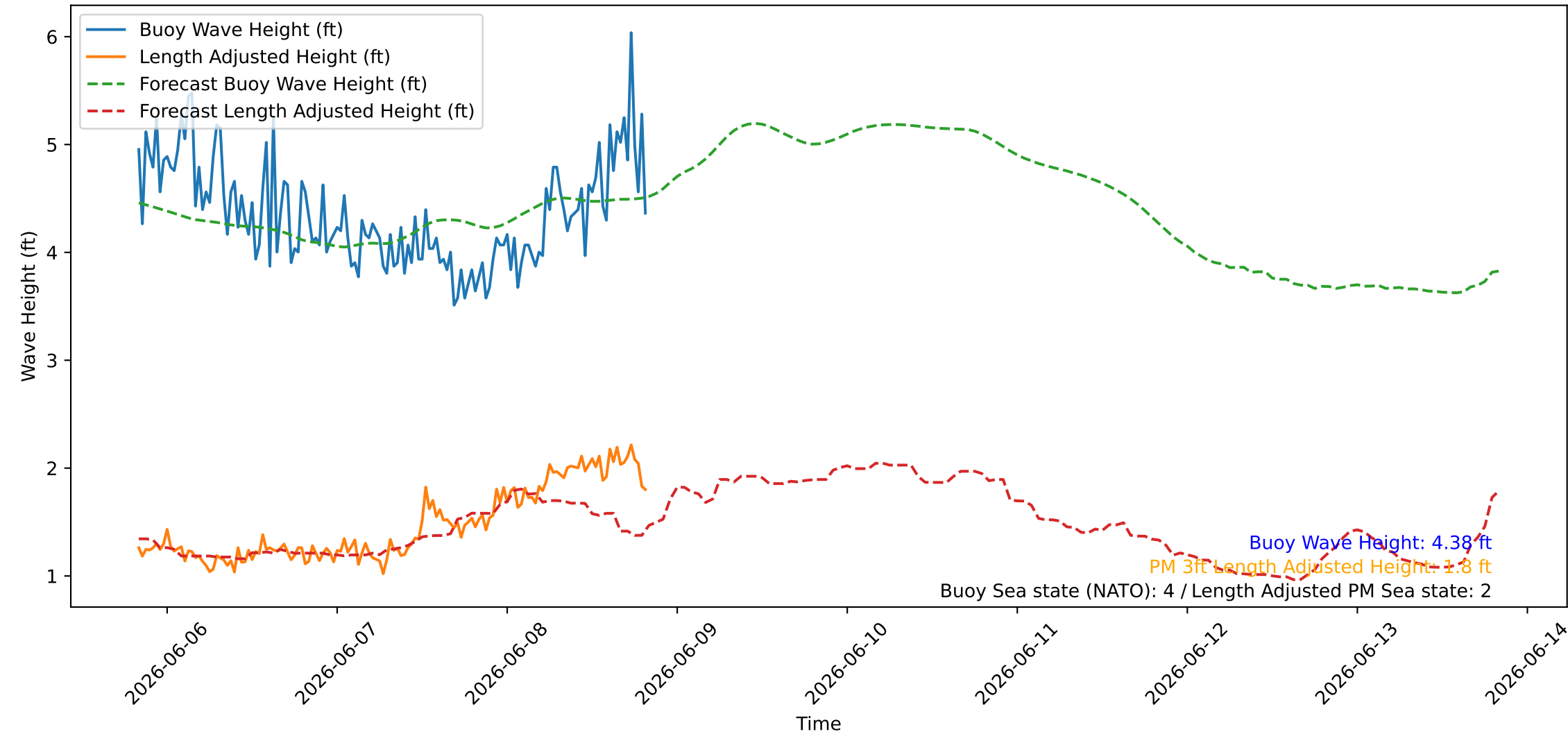
Wave Heights over Time for Oceanside Harbor at 2026-06-08 20:00:26
