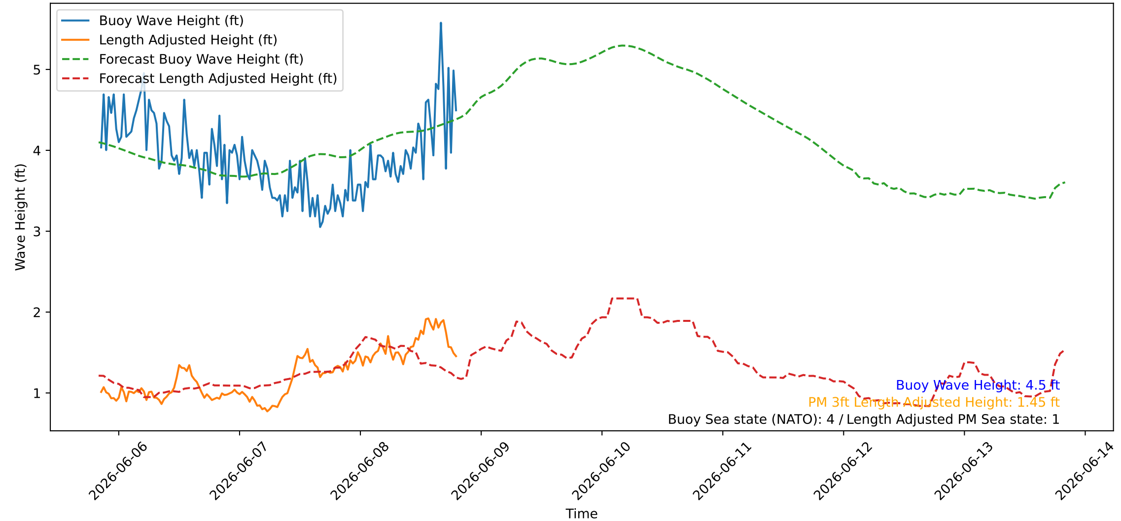
Wave Heights over Time for Red Beach at 2026-06-08 20:00:46
