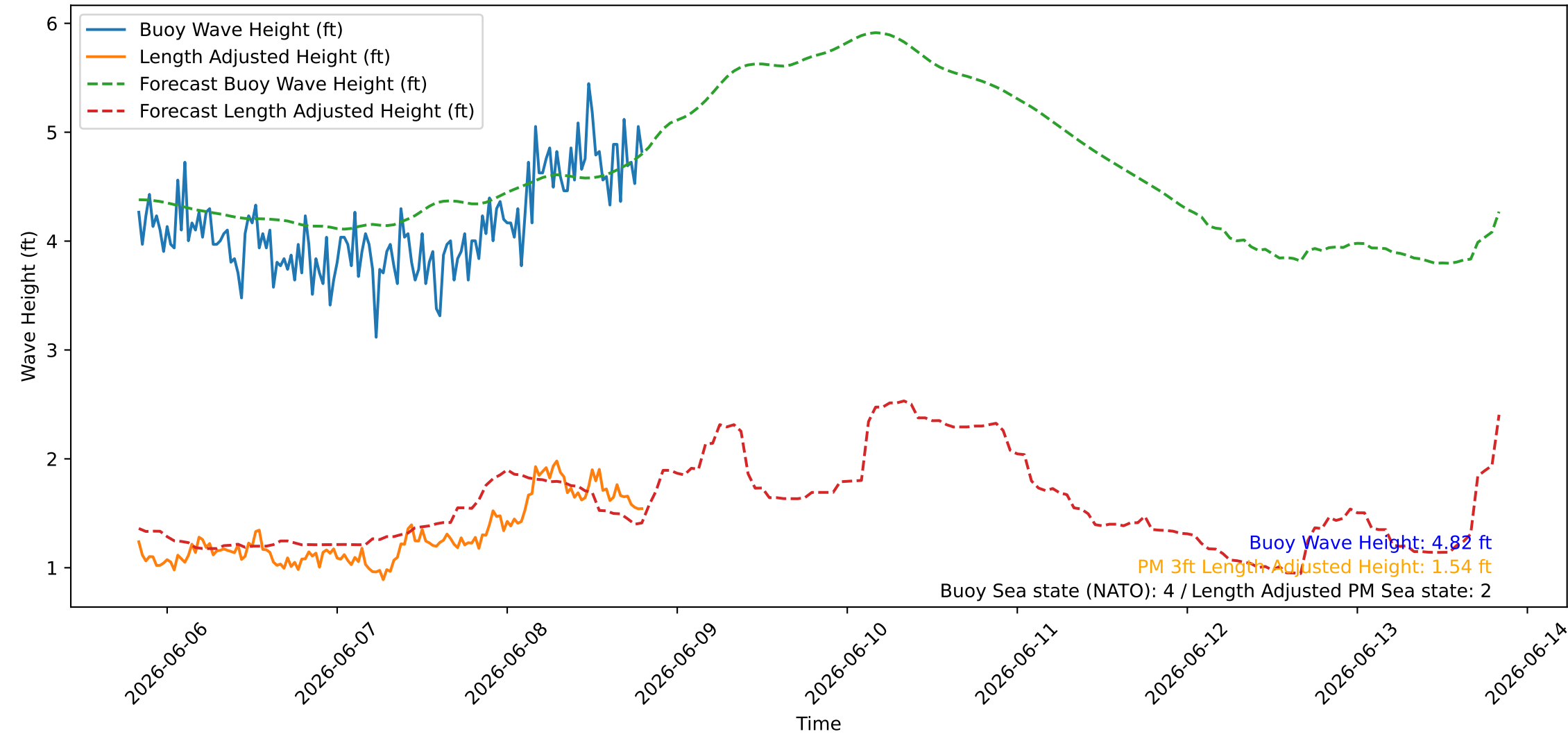
Wave Heights over Time for Green Beach at 2026-06-08 20:01:08
