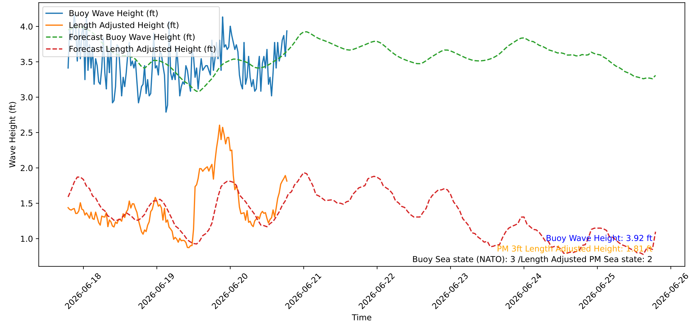
Wave Heights over Time for Oceanside Harbor at 2026-06-20 19:10:26
