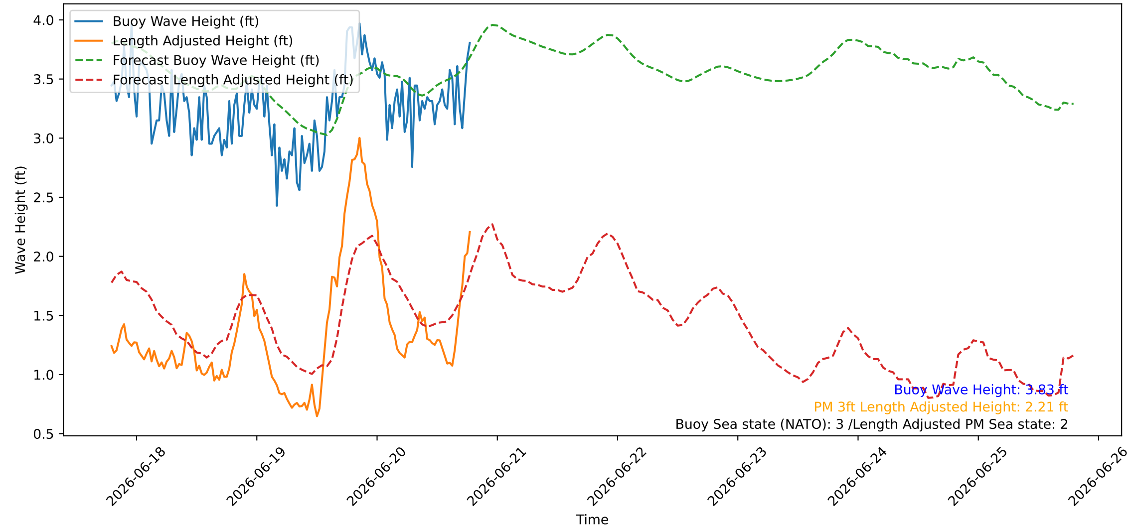
Wave Heights over Time for Green Beach at 2026-06-20 19:11:08
