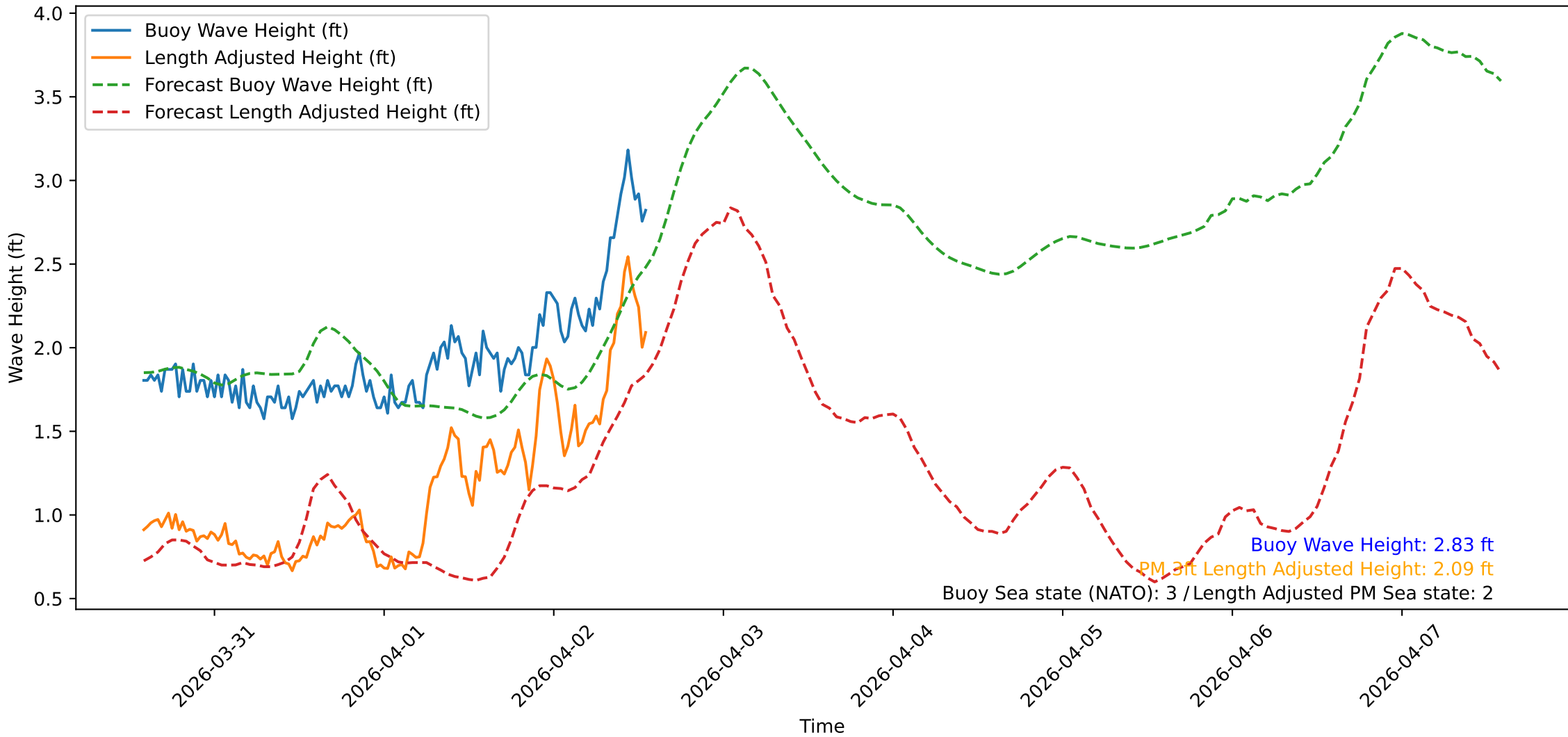
Wave Heights over Time for Oceanside Harbor at 2026-04-02 13:50:31
