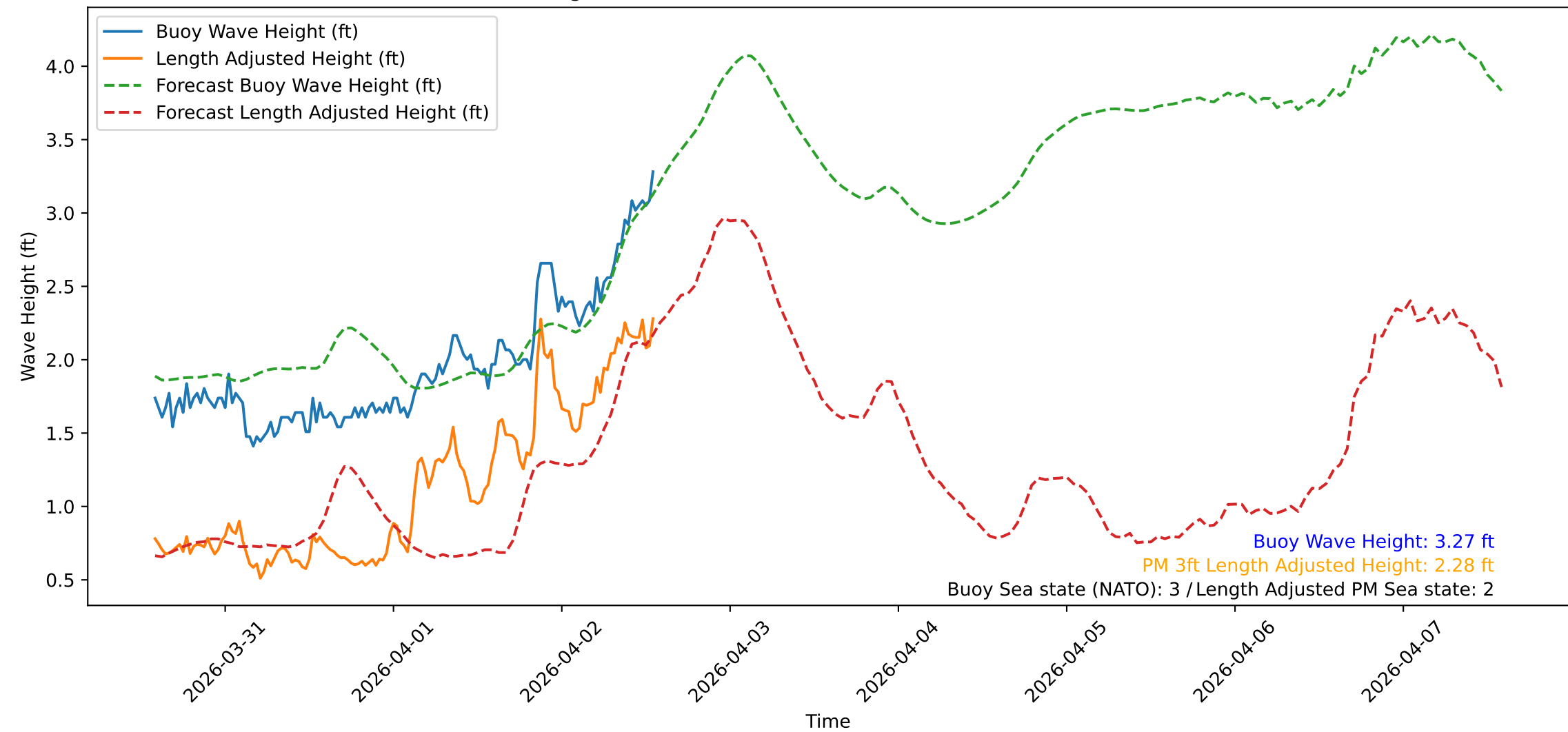
Wave Heights over Time for Green Beach at 2026-04-02 13:51:10
