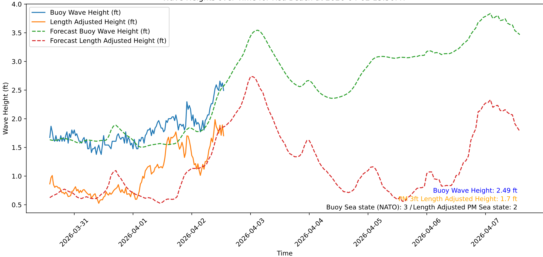
Wave Heights over Time for Red Beach at 2026-04-02 13:50:47
