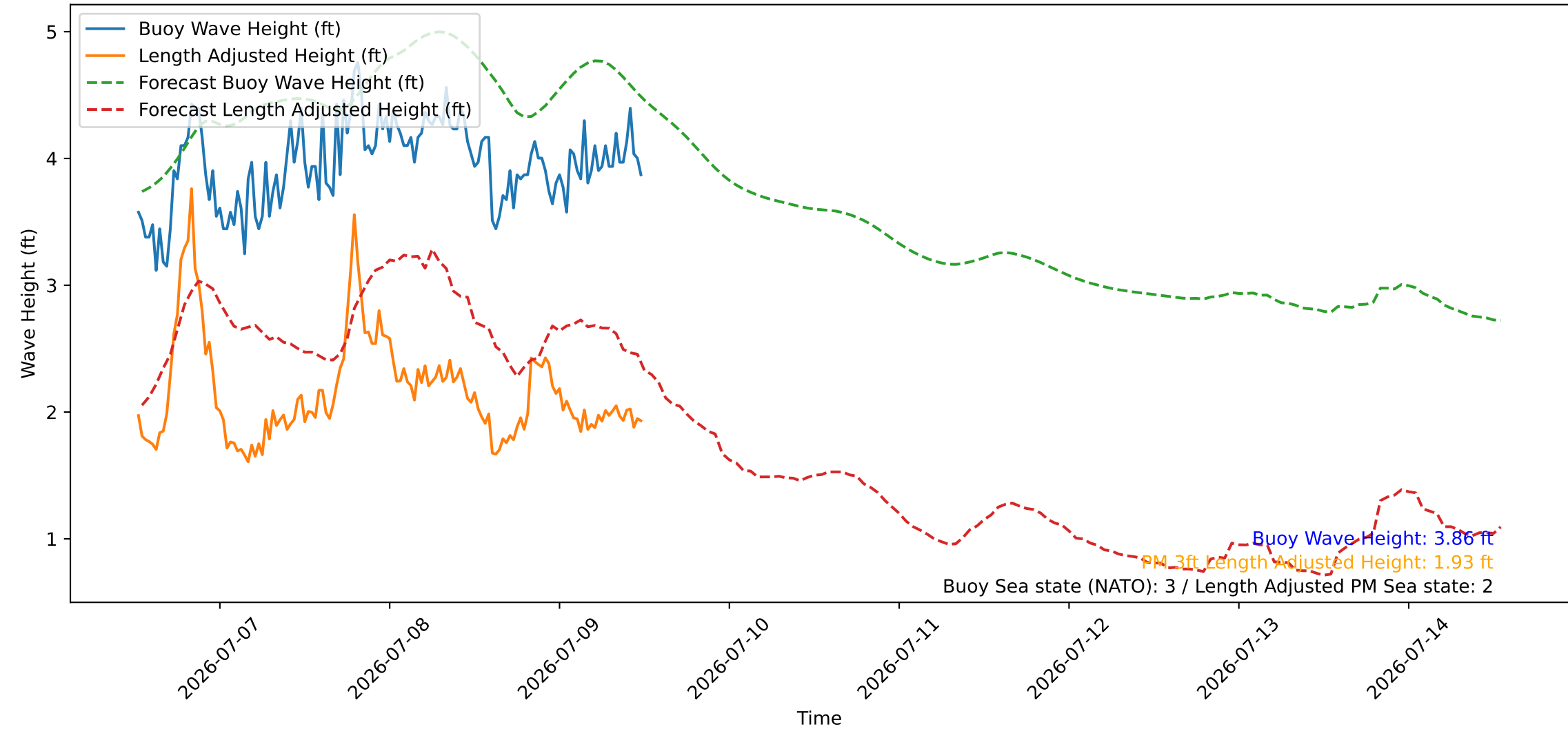
Wave Heights over Time for Green Beach at 2026-07-09 12:31:09
