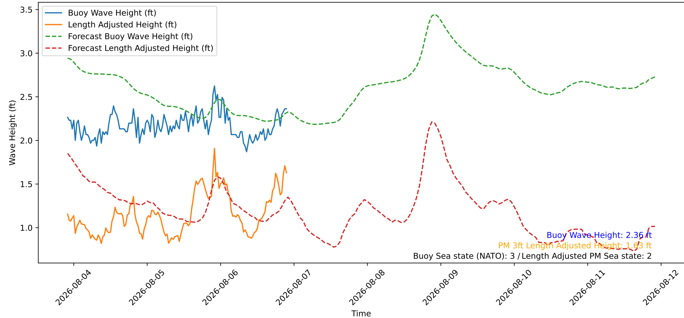
Wave Heights over Time for Green Beach at 2026-08-06 22:11:08
