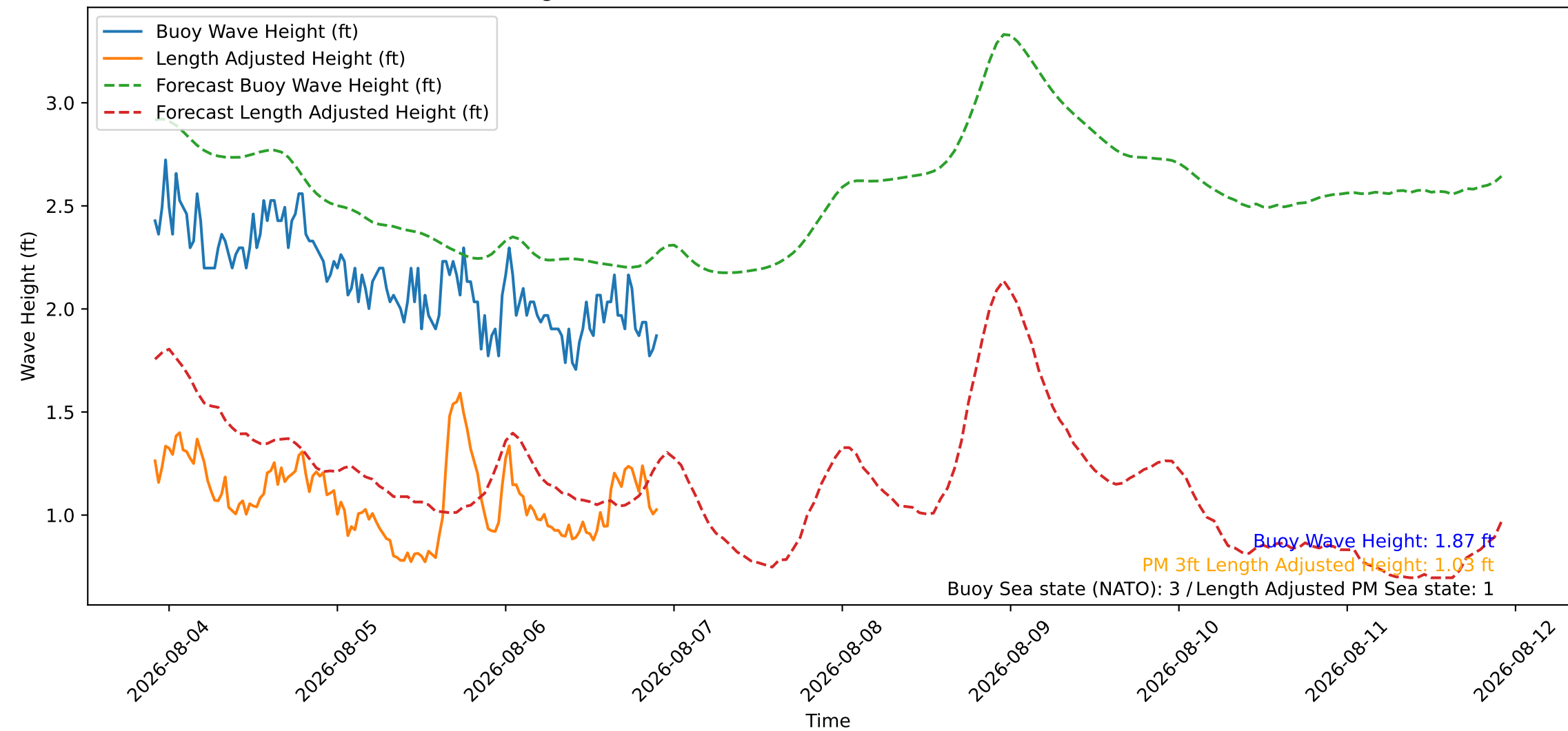
Wave Heights over Time for Oceanside Harbor at 2026-08-06 22:10:26
