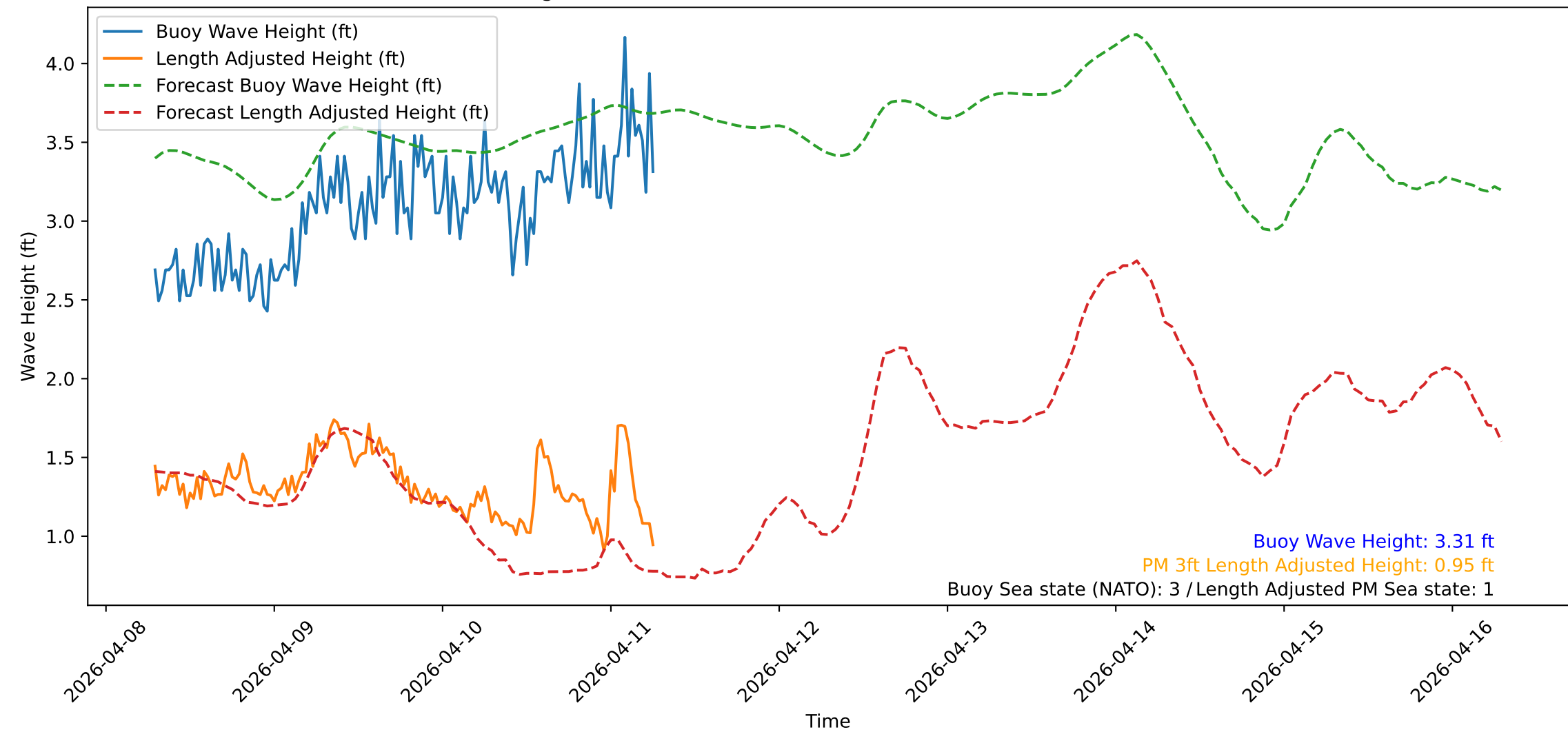
Wave Heights over Time for Oceanside Harbor at 2026-04-11 06:50:32
