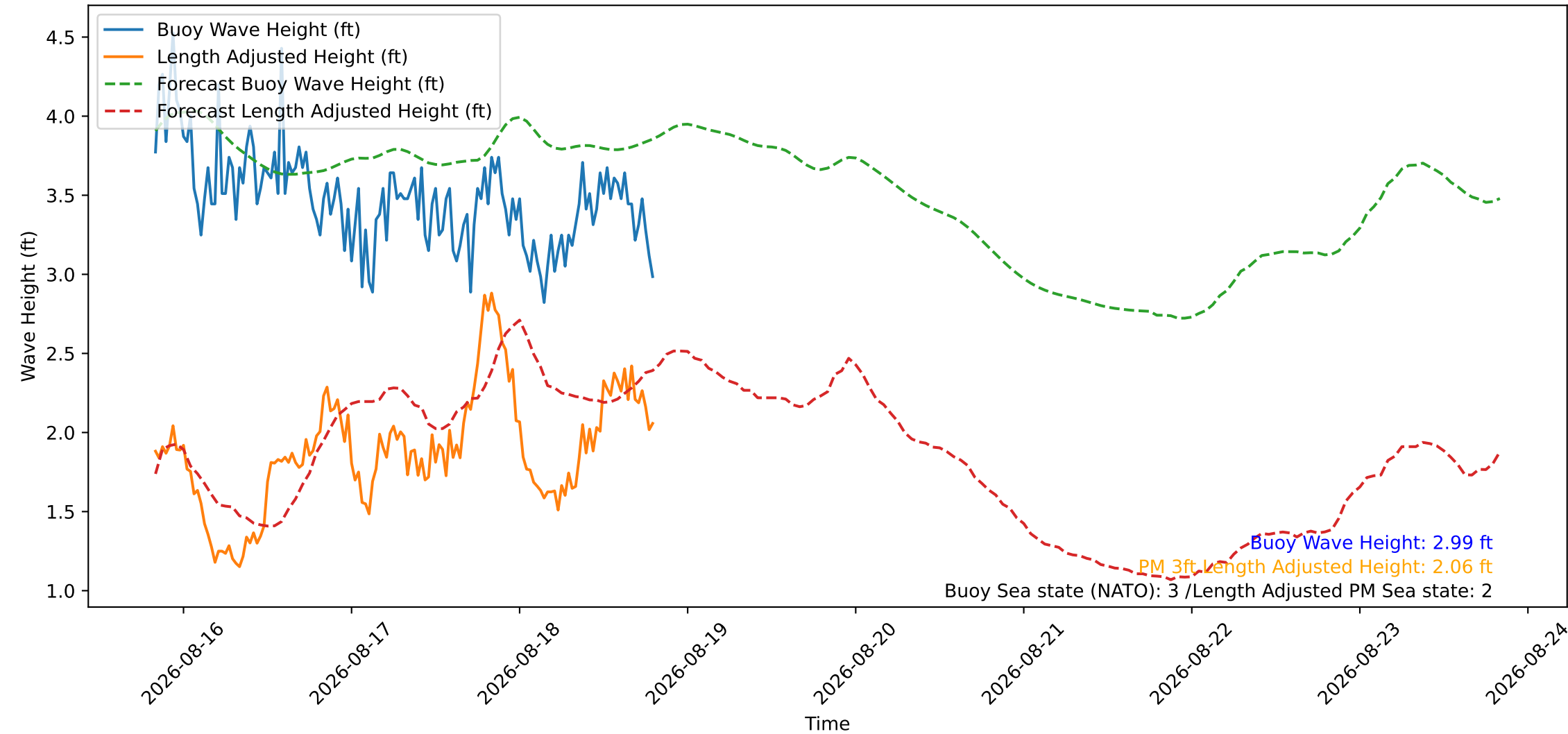
Wave Heights over Time for Oceanside Harbor at 2026-08-18 19:50:27
