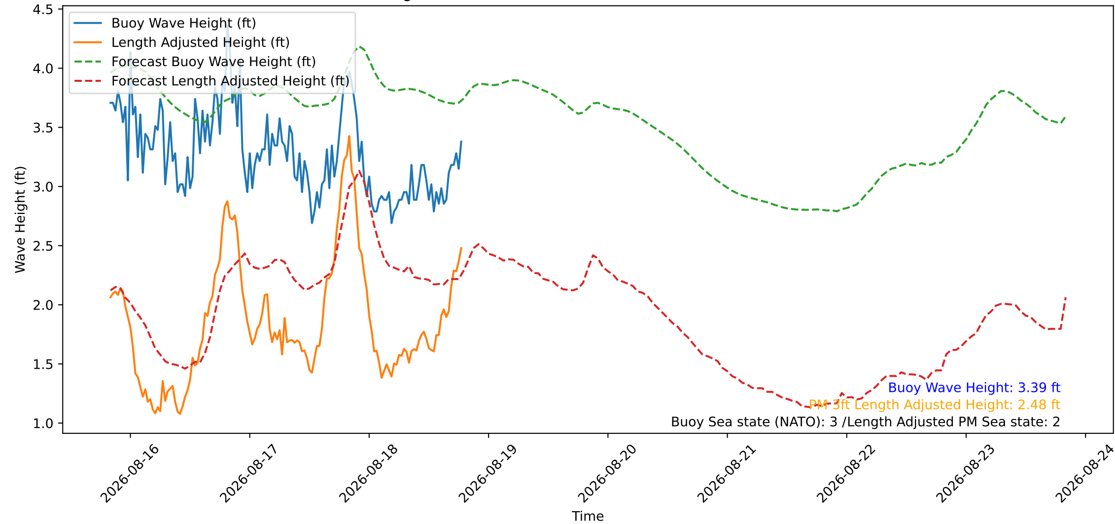
Wave Heights over Time for Green Beach at 2026-08-18 19:51:15
