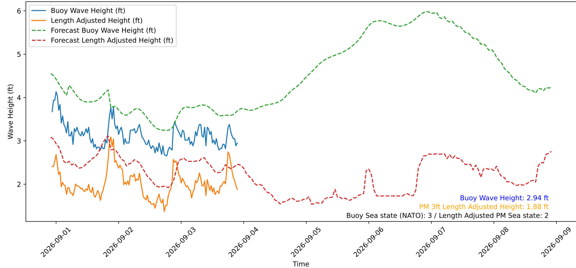
Wave Heights over Time for Green Beach at 2026-09-03 22:11:12
