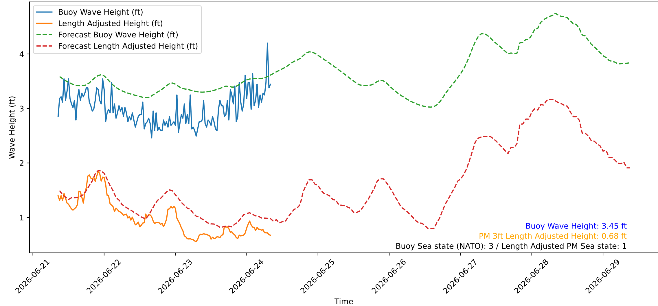
Wave Heights over Time for Green Beach at 2026-06-24 08:41:07
