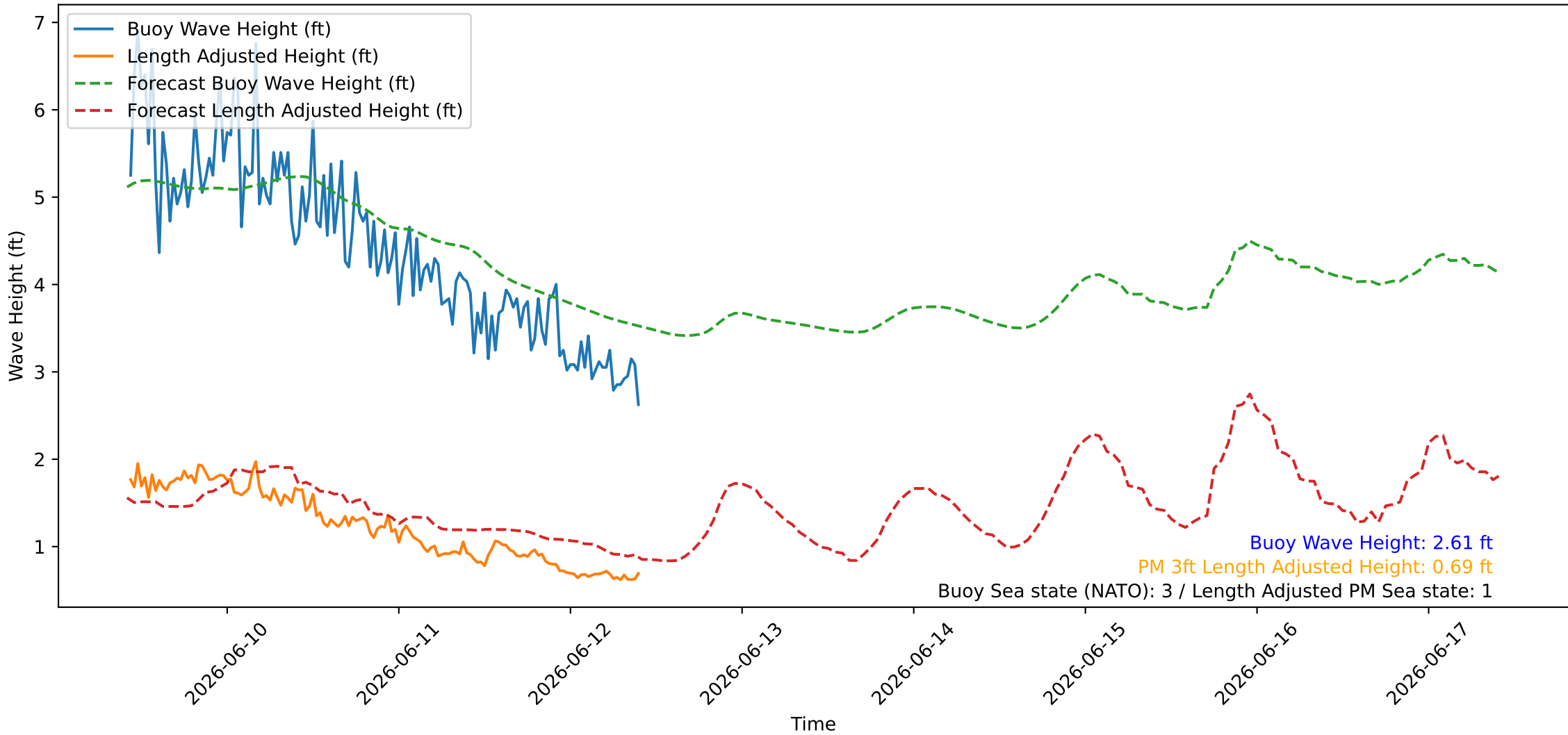
Wave Heights over Time for Red Beach at 2026-06-12 10:20:47
