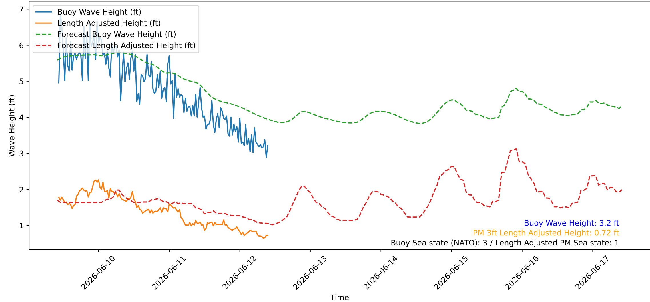
Wave Heights over Time for Green Beach at 2026-06-12 10:21:10
