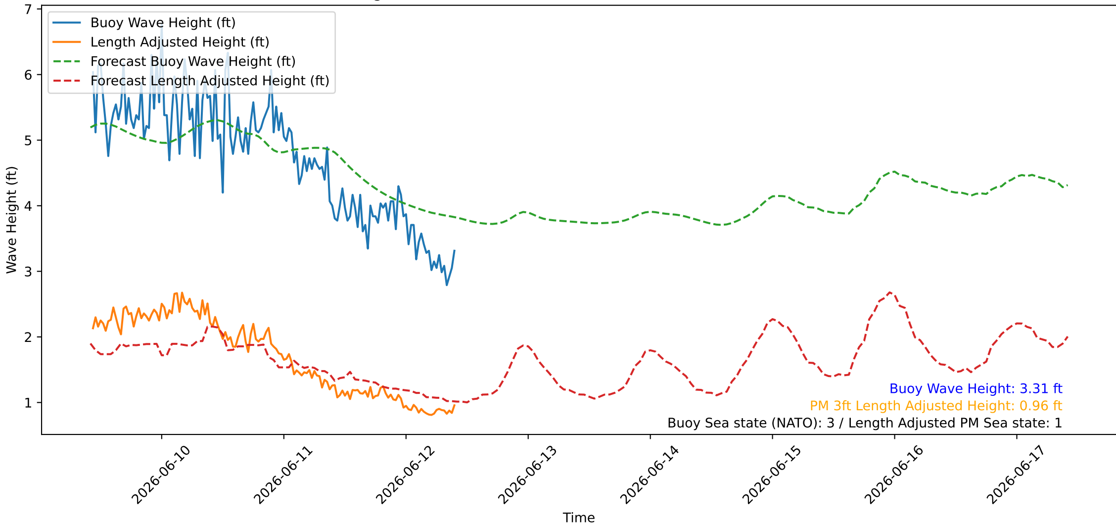
Wave Heights over Time for Oceanside Harbor at 2026-06-12 10:20:26
