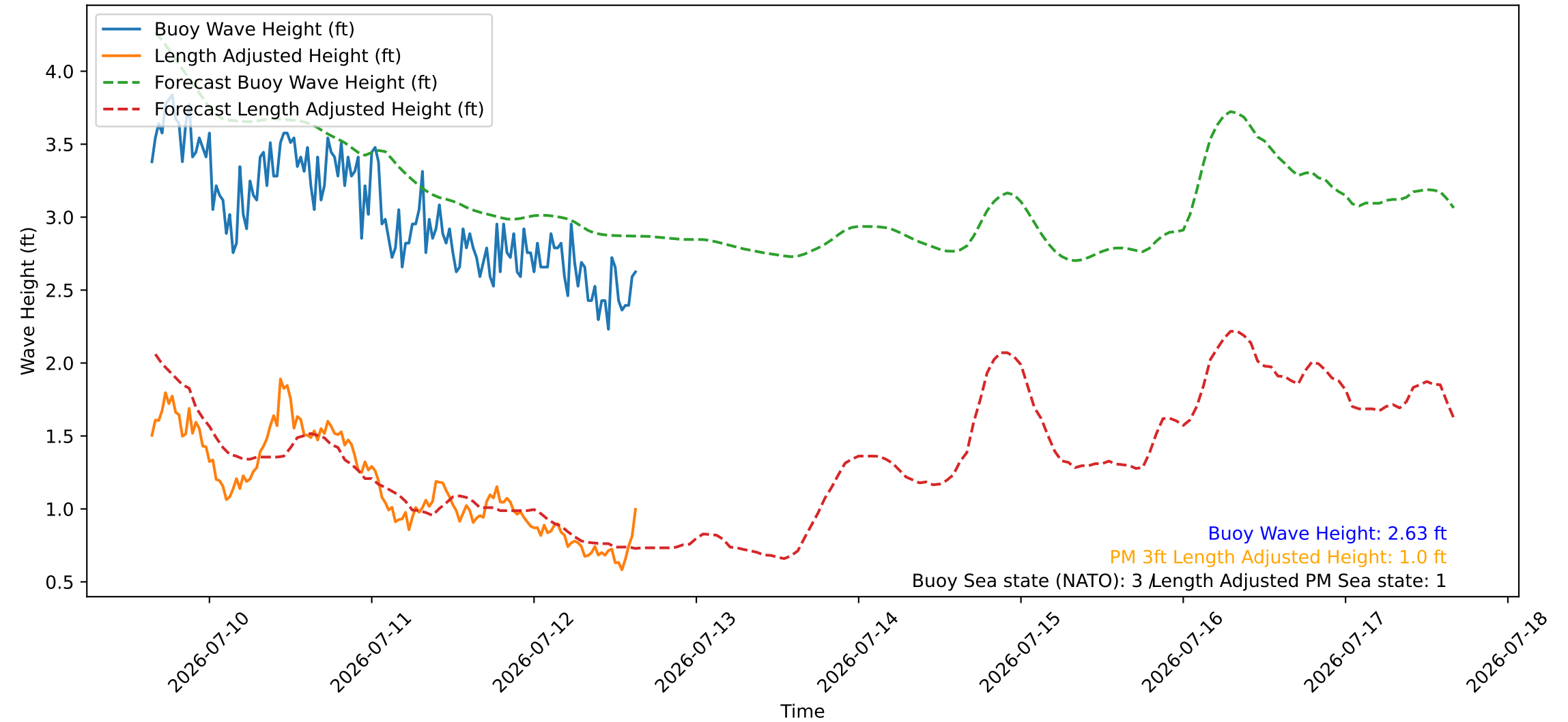
Wave Heights over Time for Green Beach at 2026-07-12 15:41:08
