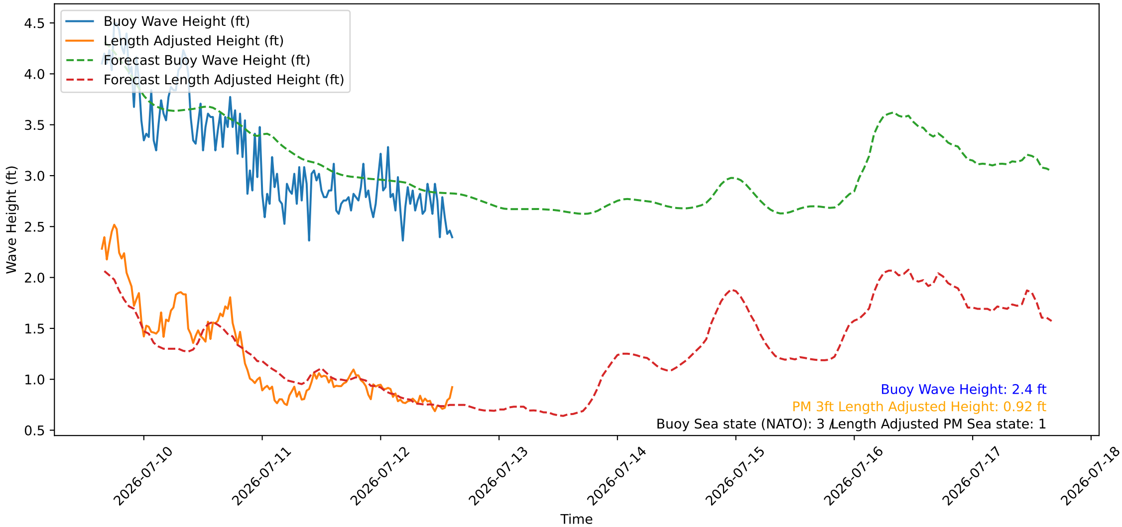
Wave Heights over Time for Oceanside Harbor at 2026-07-12 15:40:26
