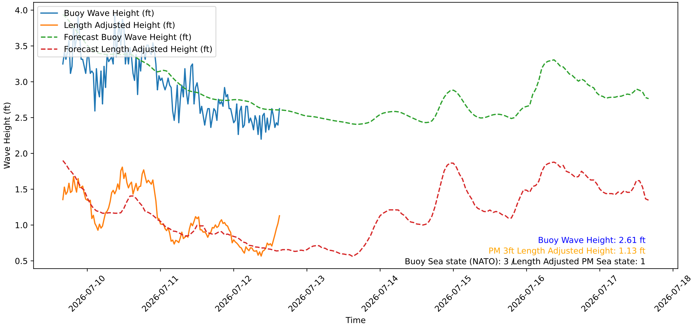
Wave Heights over Time for Red Beach at 2026-07-12 15:40:45
