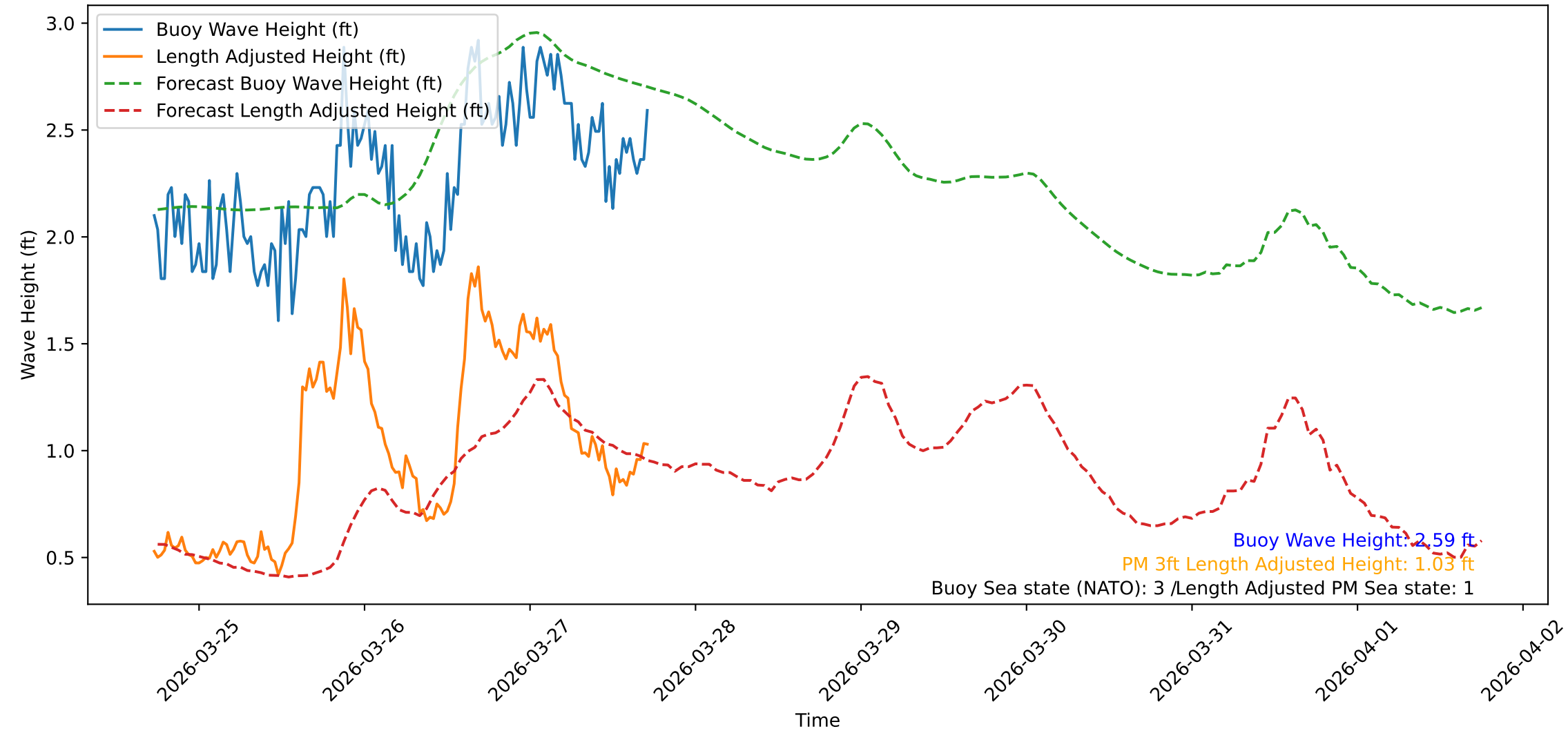
Wave Heights over Time for Oceanside Harbor at 2026-03-27 17:40:31
