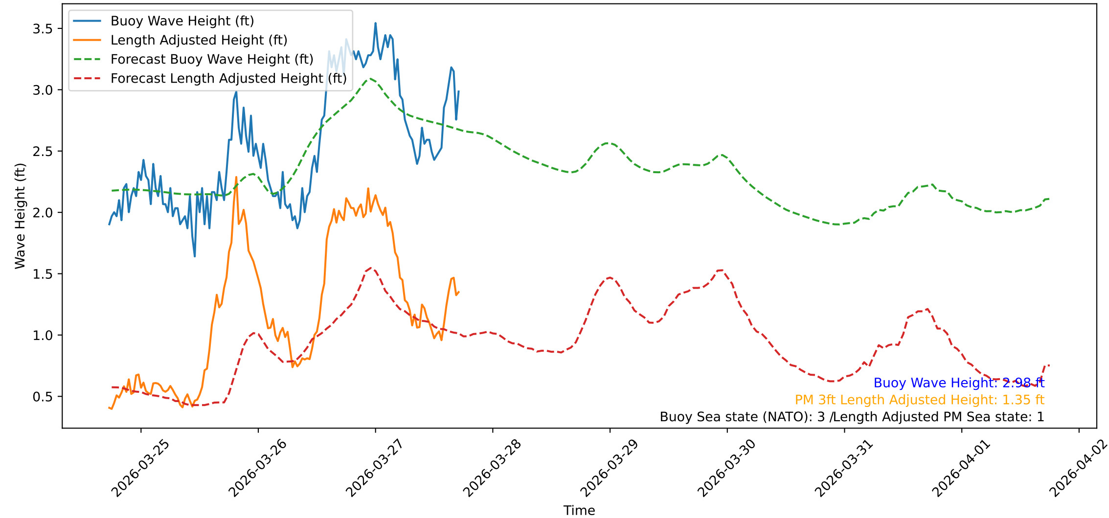
Wave Heights over Time for Green Beach at 2026-03-27 17:41:10
