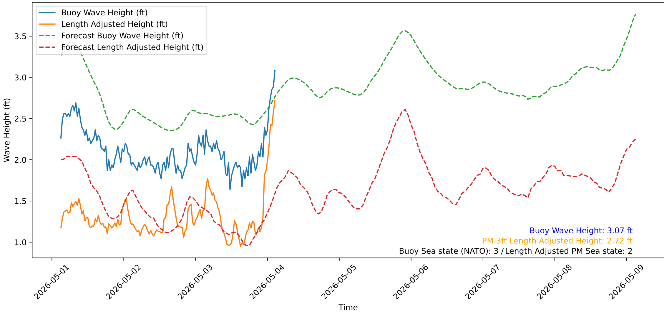
Wave Heights over Time for Oceanside Harbor at 2026-05-04 03:00:31
