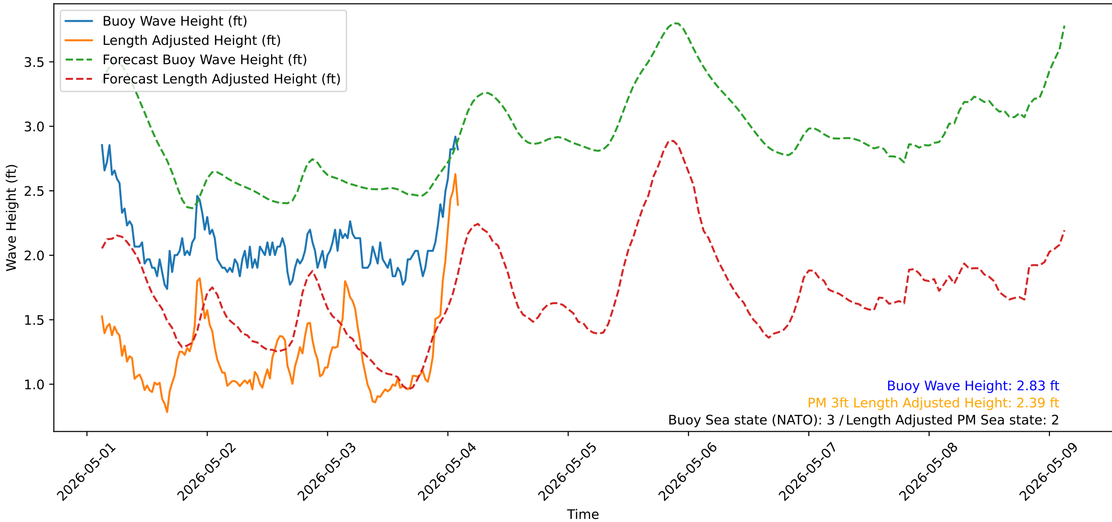
Wave Heights over Time for Green Beach at 2026-05-04 03:01:12
