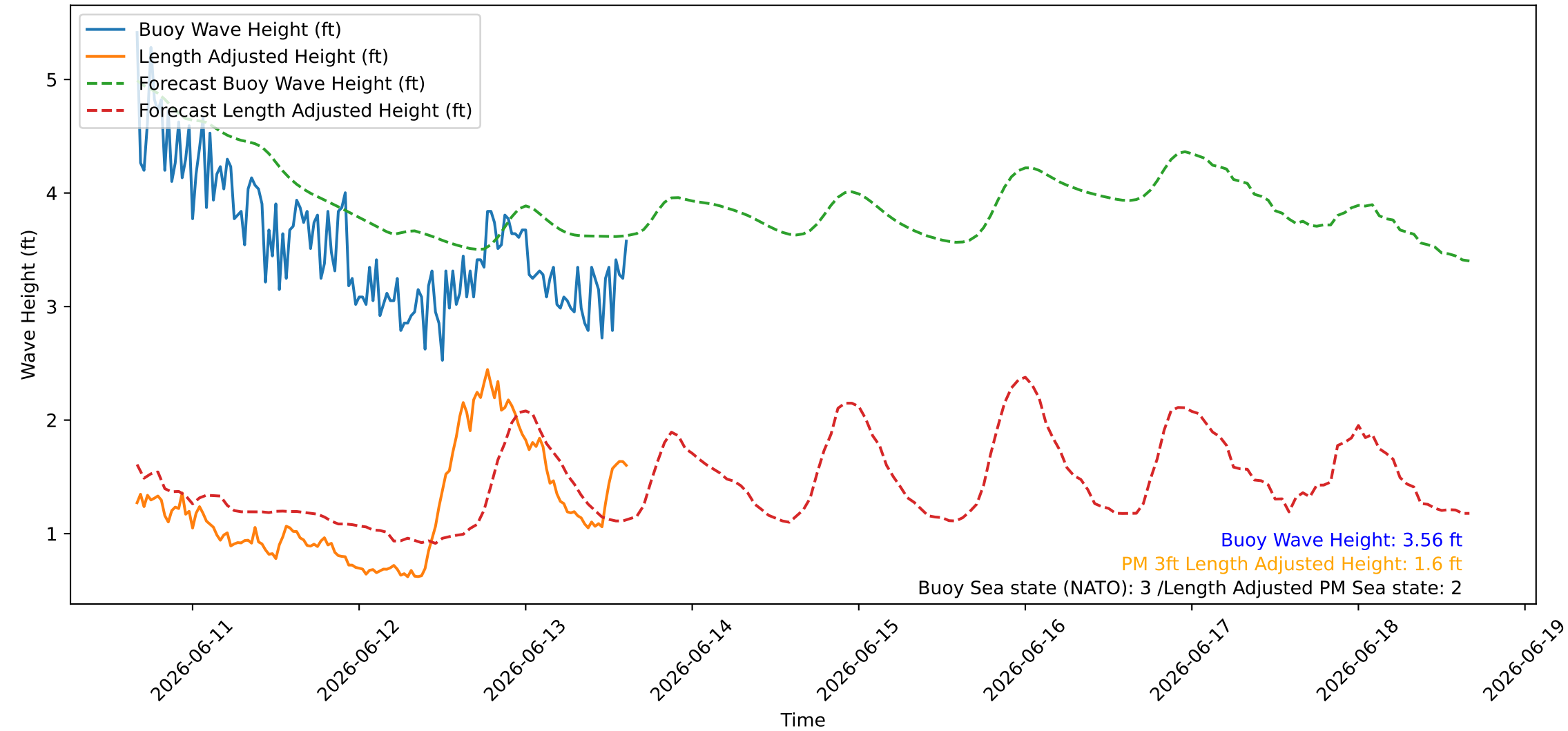
Wave Heights over Time for Red Beach at 2026-06-13 15:30:45
