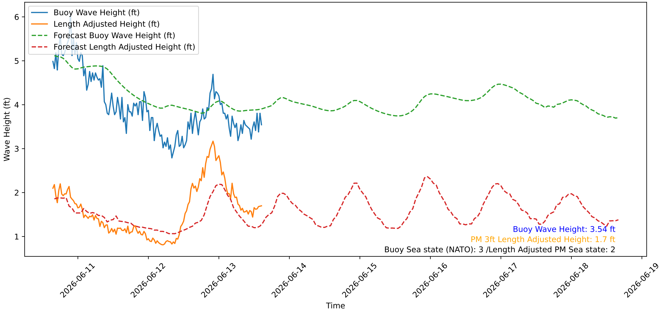
Wave Heights over Time for Oceanside Harbor at 2026-06-13 15:30:26
