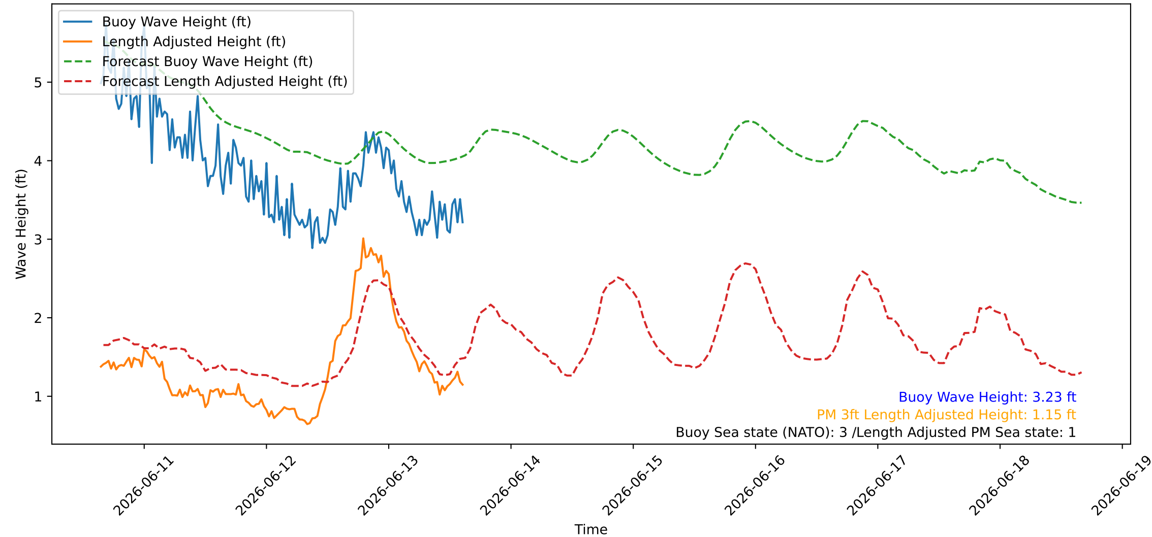
Wave Heights over Time for Green Beach at 2026-06-13 15:31:08
