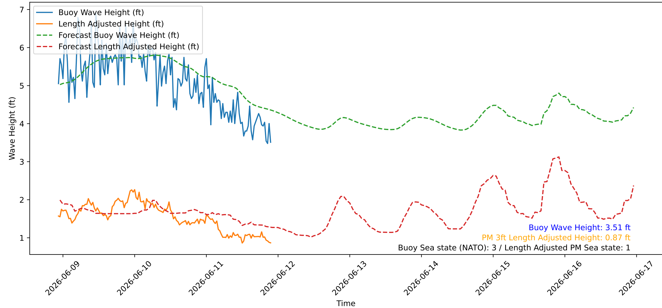
Wave Heights over Time for Green Beach at 2026-06-11 22:31:09
