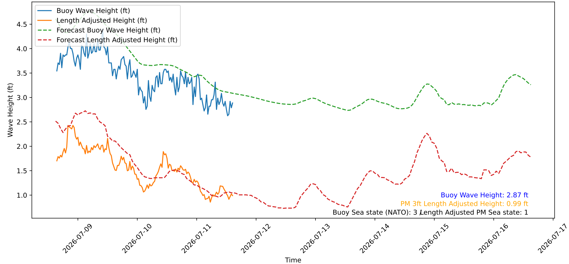
Wave Heights over Time for Green Beach at 2026-07-11 15:21:08
