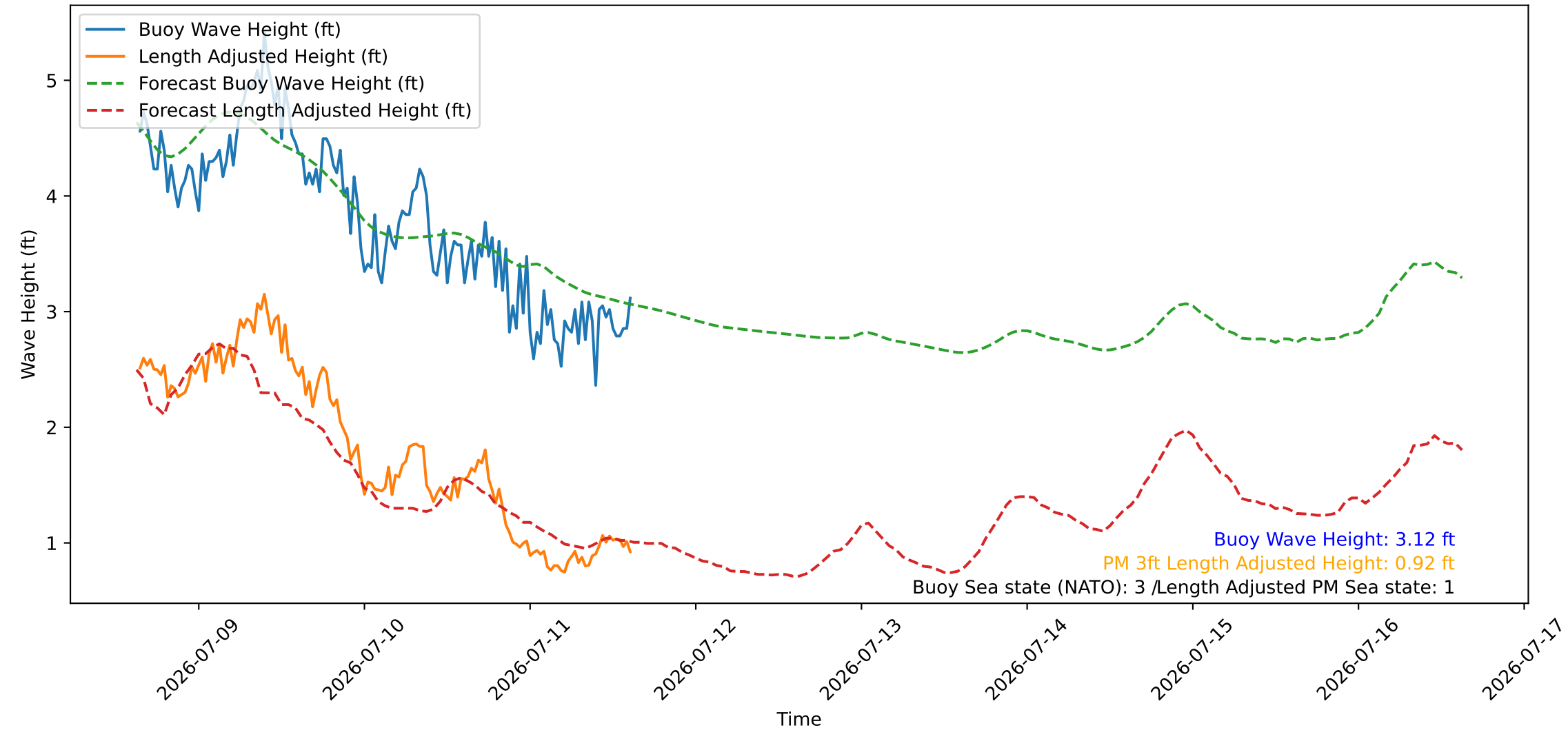
Wave Heights over Time for Oceanside Harbor at 2026-07-11 15:20:26
