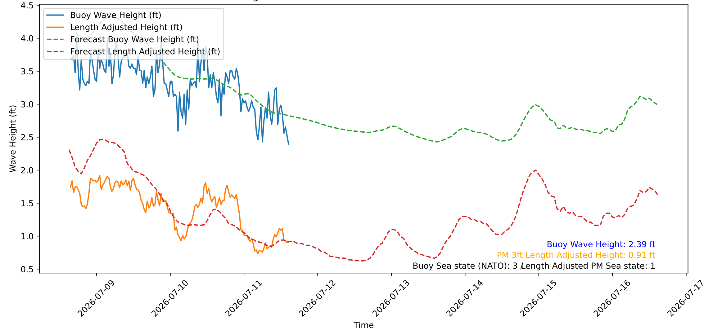
Wave Heights over Time for Red Beach at 2026-07-11 15:20:46
