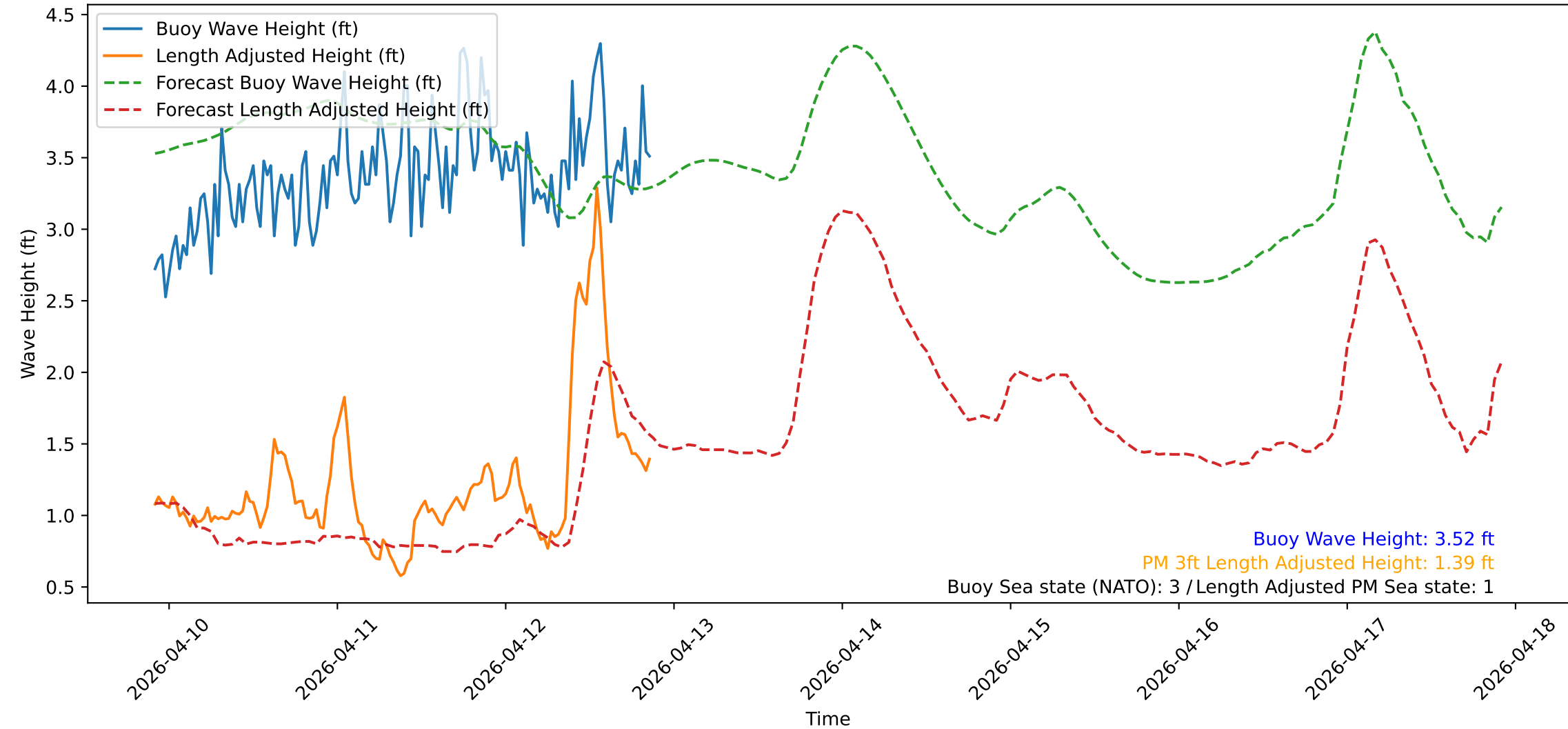
Wave Heights over Time for Red Beach at 2026-04-12 21:30:50
