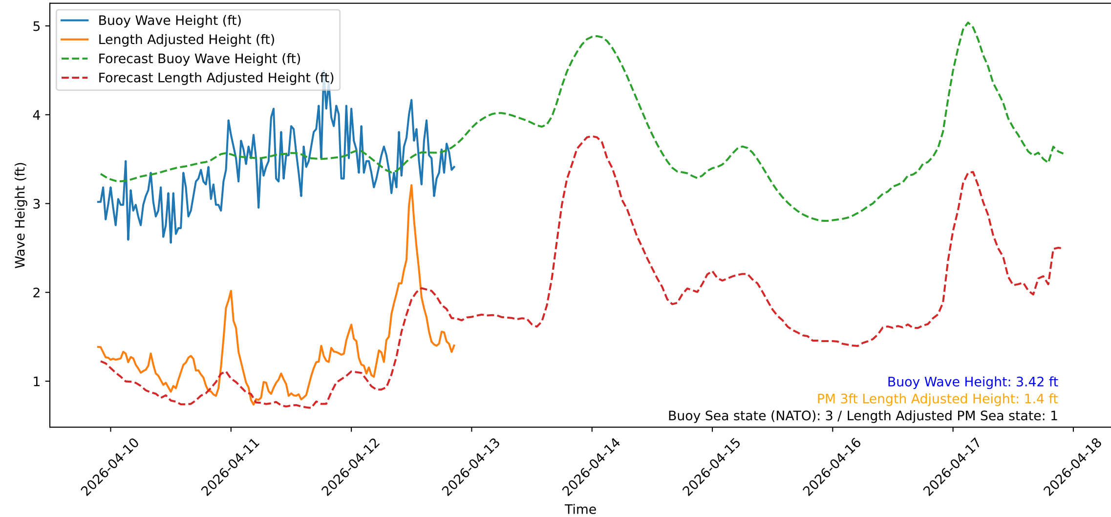
Wave Heights over Time for Green Beach at 2026-04-12 21:31:12
