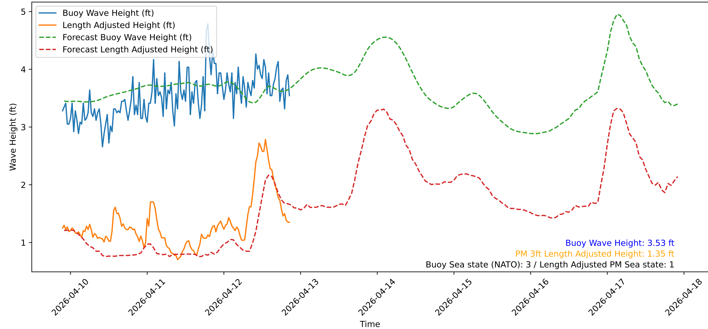
Wave Heights over Time for Oceanside Harbor at 2026-04-12 21:30:31
