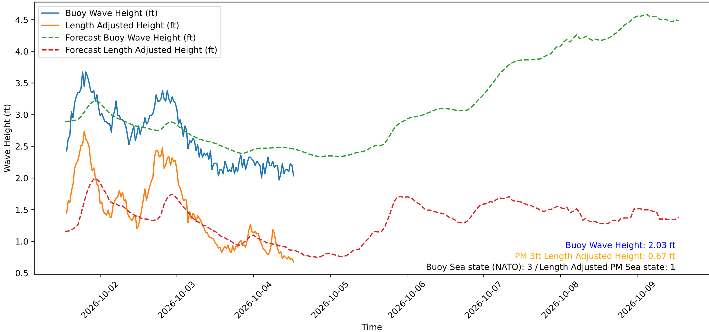
Wave Heights over Time for Green Beach at 2026-10-04 13:11:11
