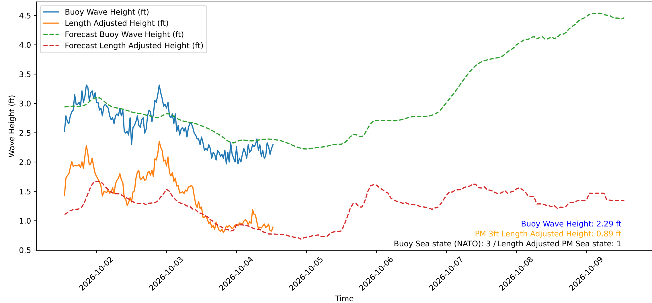
Wave Heights over Time for Oceanside Harbor at 2026-10-04 13:10:29
