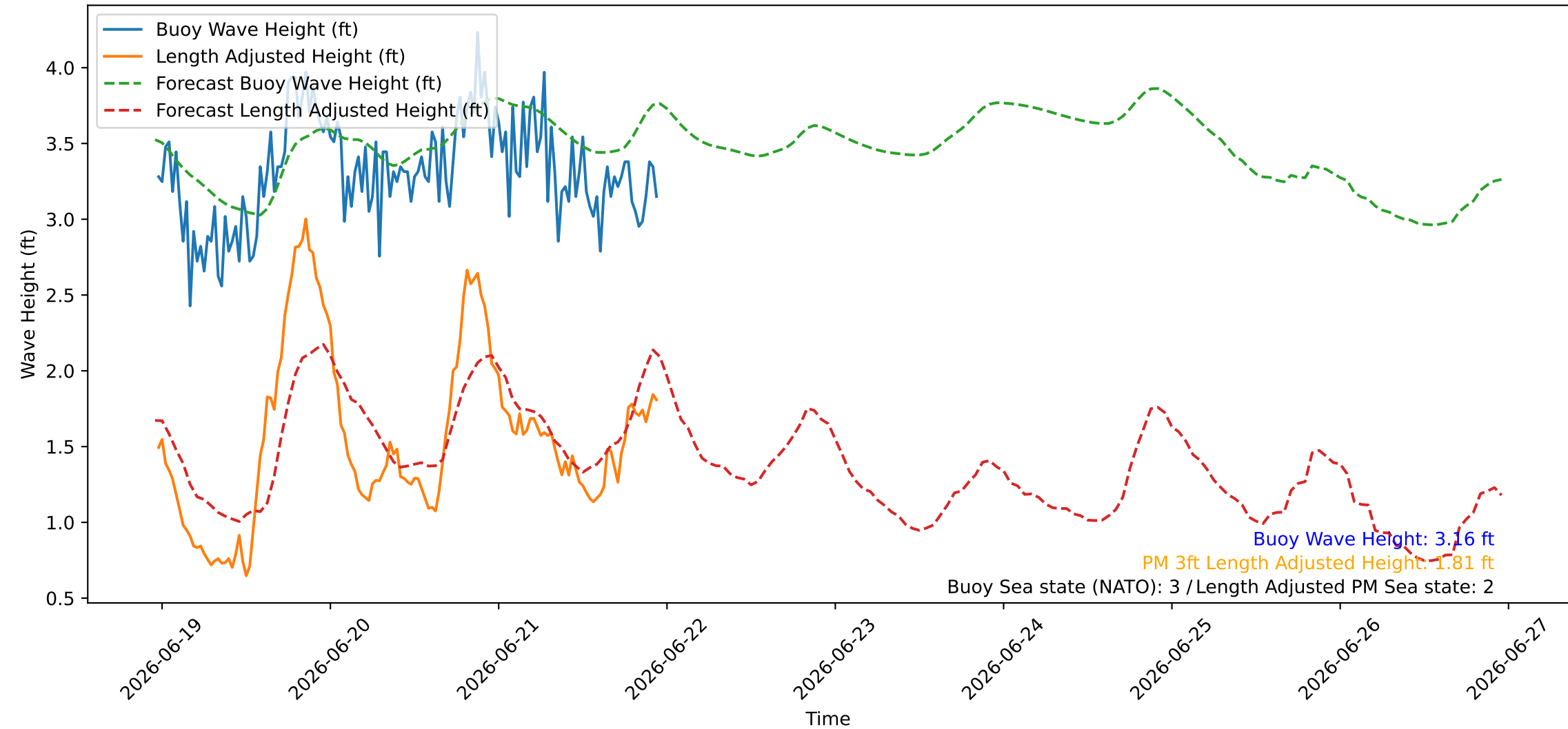
Wave Heights over Time for Green Beach at 2026-06-21 23:21:08
