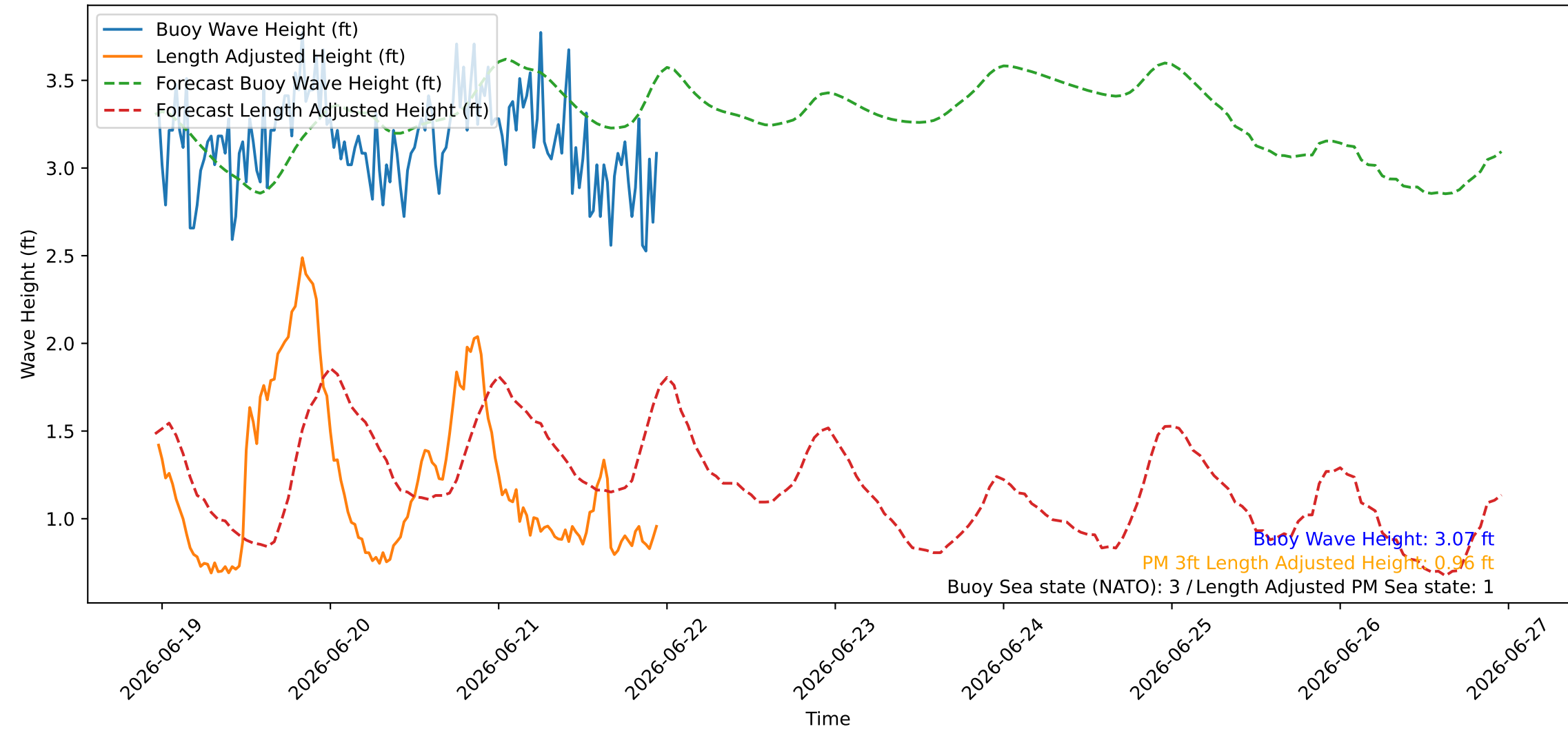
Wave Heights over Time for Red Beach at 2026-06-21 23:20:46
