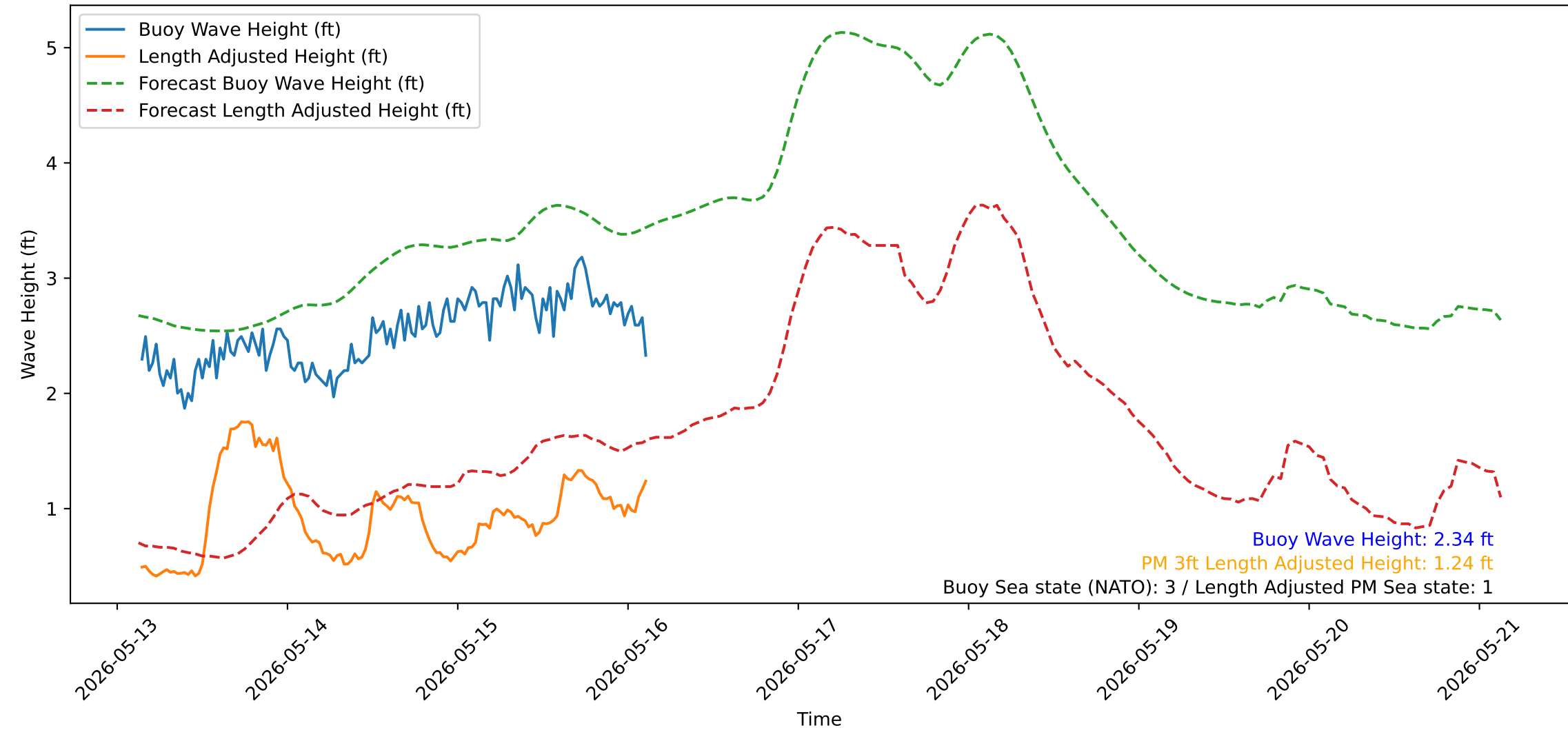
Wave Heights over Time for Red Beach at 2026-05-16 03:10:51
