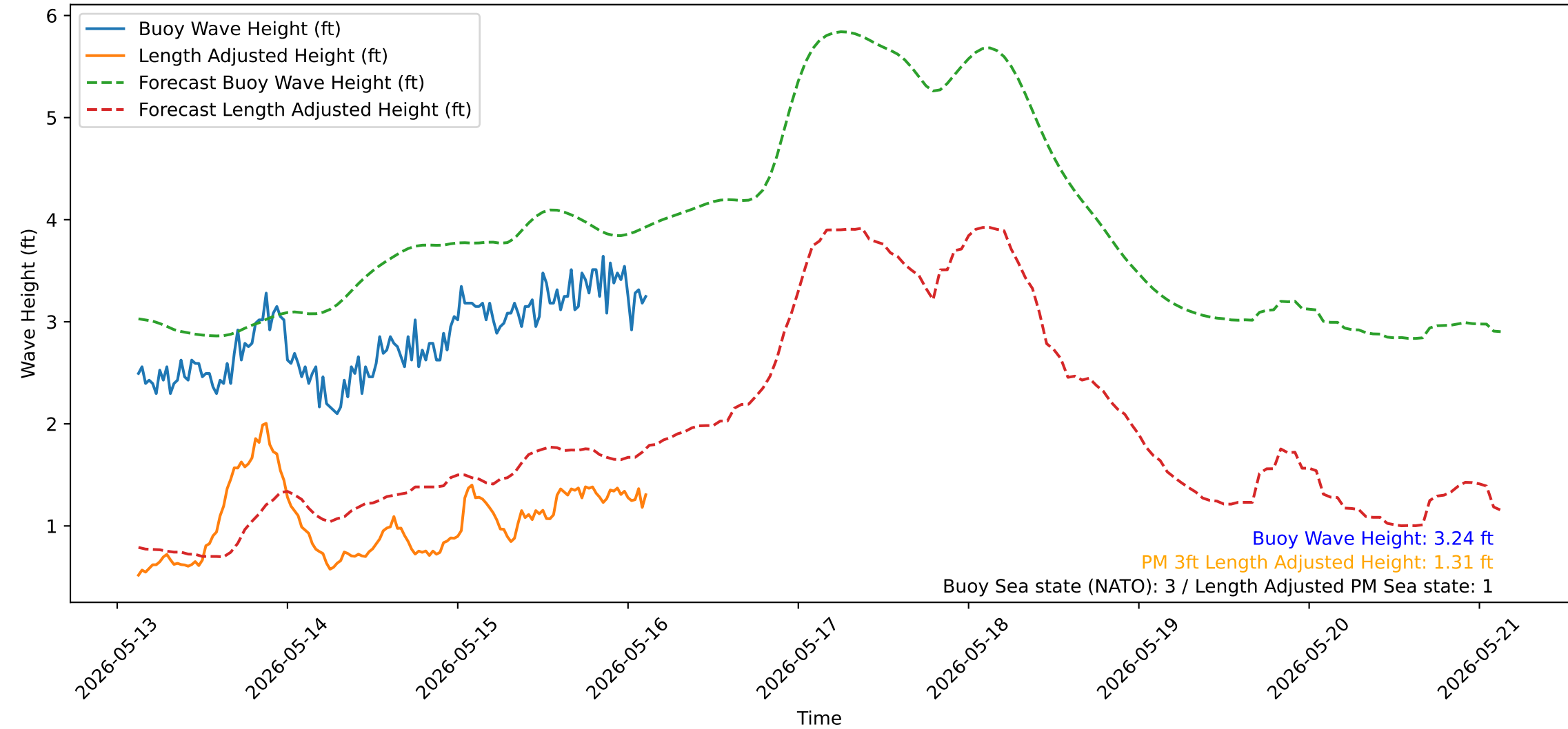
Wave Heights over Time for Green Beach at 2026-05-16 03:11:14
