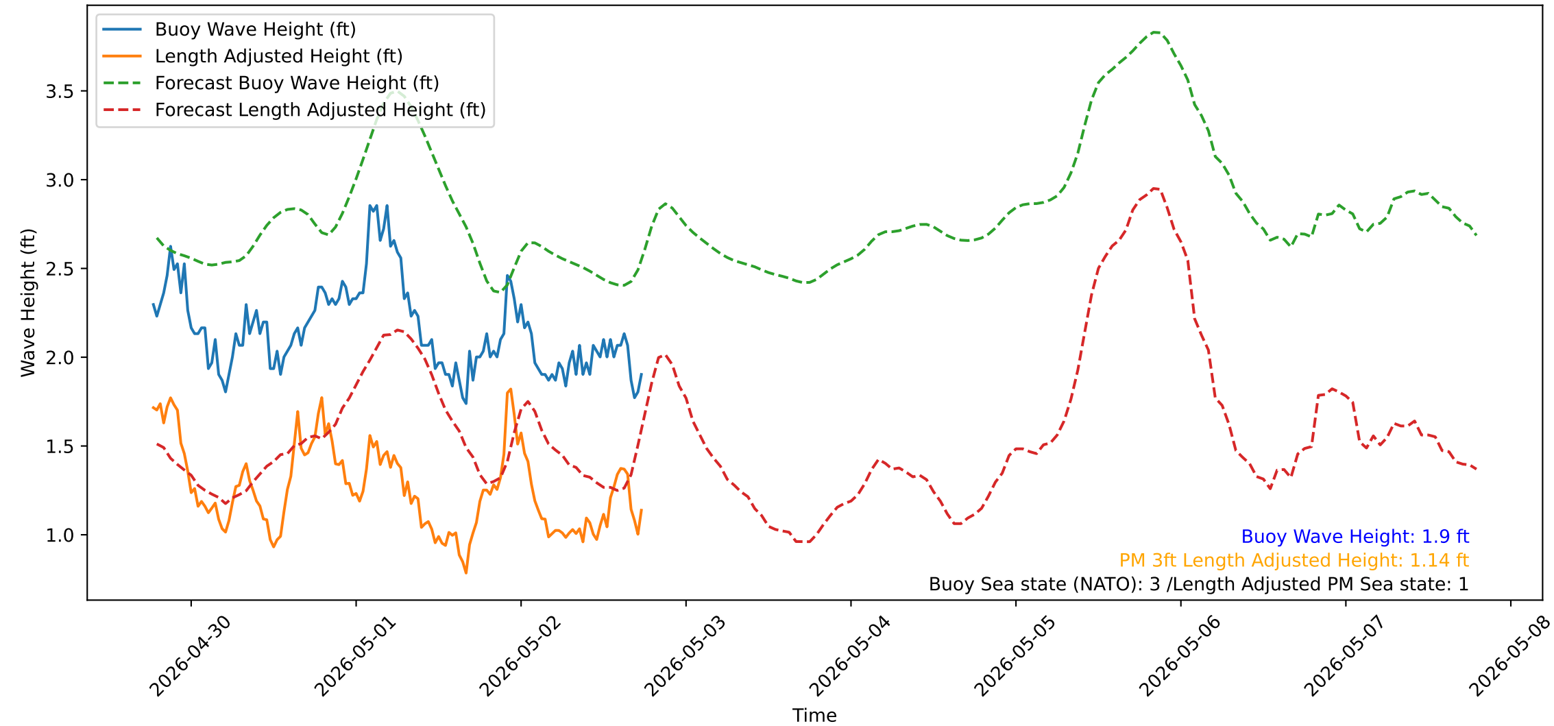
Wave Heights over Time for Green Beach at 2026-05-02 18:31:13
