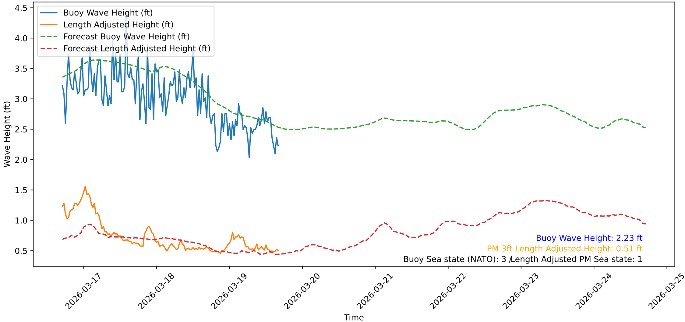
Wave Heights over Time for Oceanside Harbor at 2026-03-19 17:00:32
