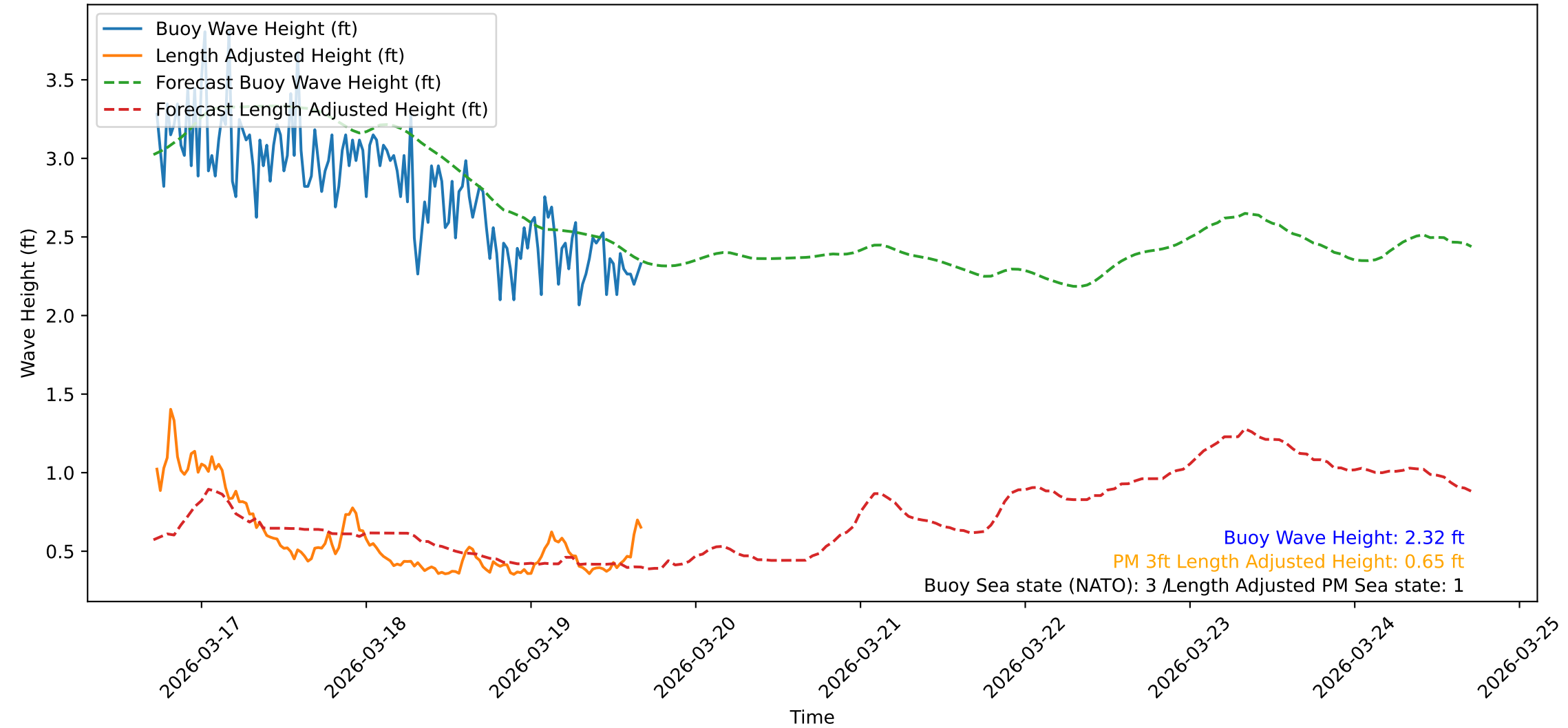
Wave Heights over Time for Red Beach at 2026-03-19 17:00:47
