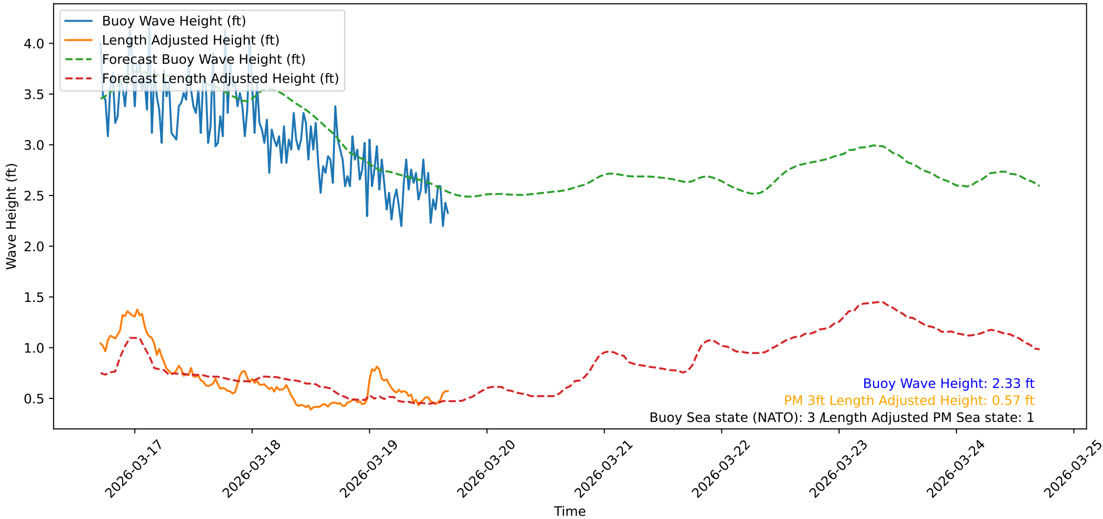
Wave Heights over Time for Green Beach at 2026-03-19 17:01:13
